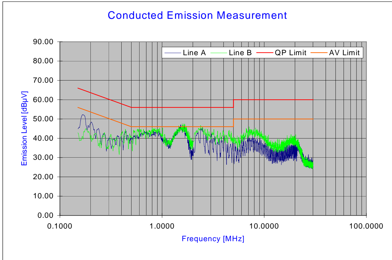
Plot C-1. Line-Conducted Test Plot
