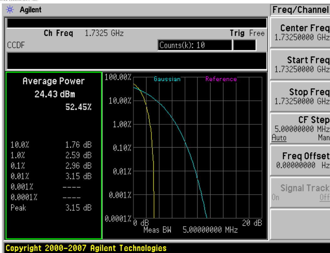
Plot 7-19. Peak-Average Ratio Plot (AWS CDMA Mode – Ch. 450)
