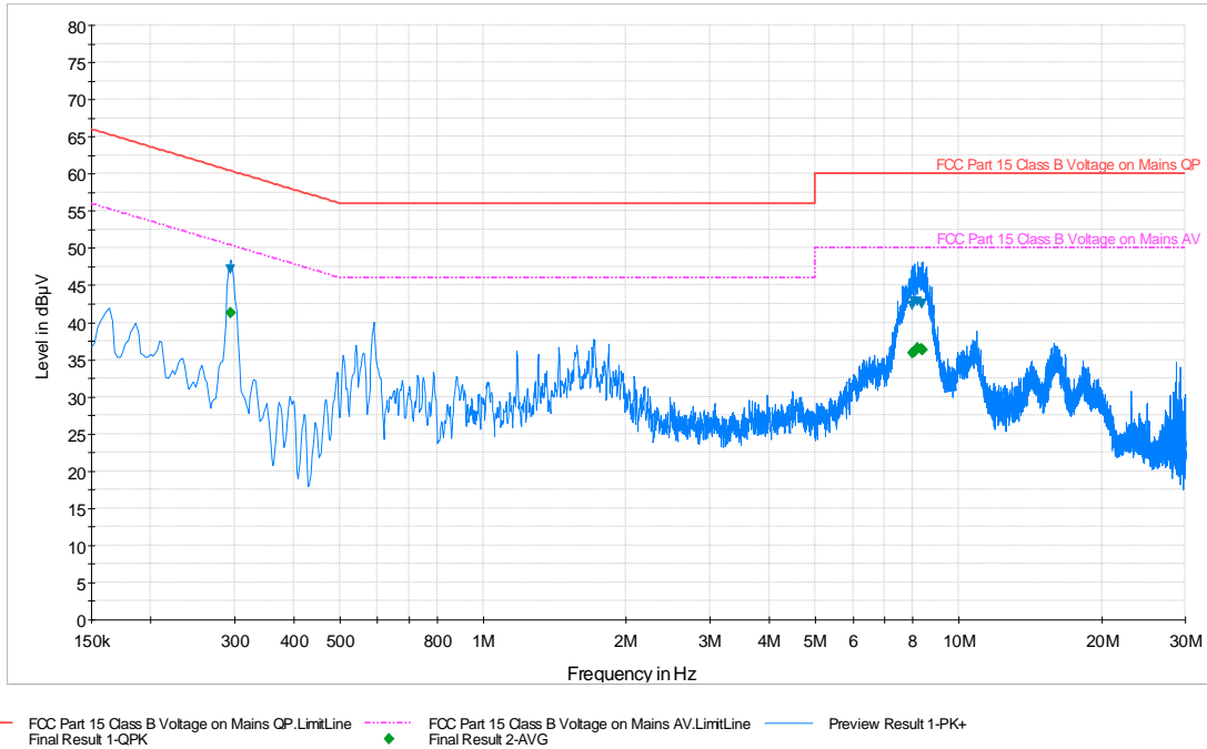
Plot 6-72. Line Conducted Plot with 802.11a UNII Band 2 (N)
