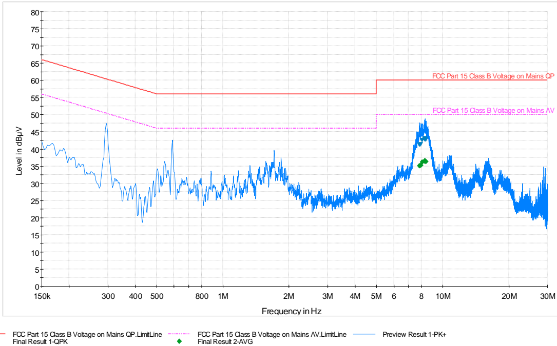
Plot 6-74. Line Conducted Plot with 802.11a UNII Band 3 (N)
