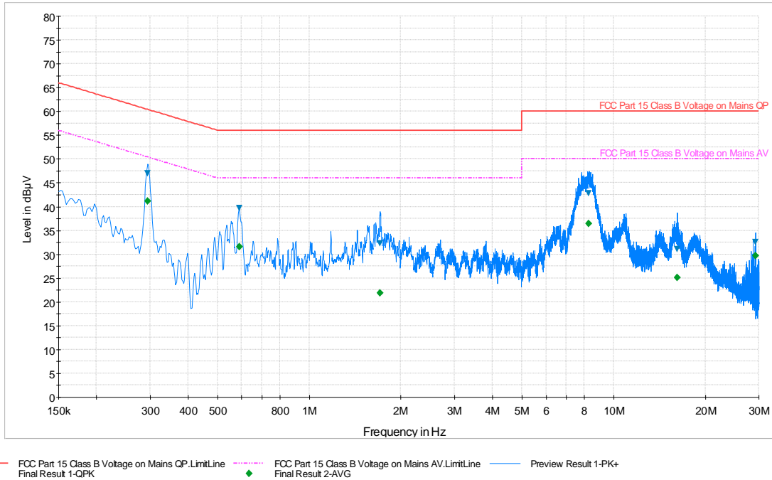
Plot 6-71. Line Conducted Plot with 802.11a UNII Band 2 (L1)
