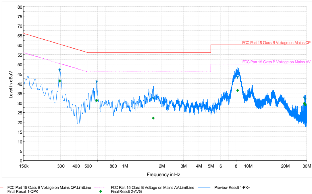
Plot 6-73. Line Conducted Plot with 802.11a UNII Band 3 (L1)
