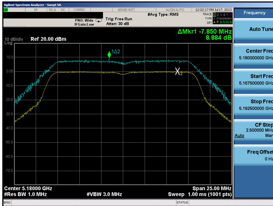
Plot 6-52. Peak Excursion Ratio Plot (802.11a)
