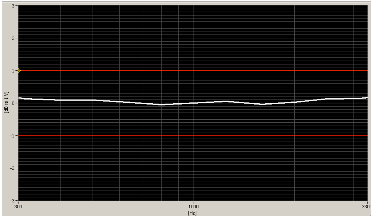
Figure 6-3 Helmholtz Coil Validation for Frequency Response
