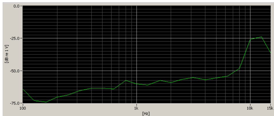
Figure 6-2 Worst-case ABM2 Plot for WD
