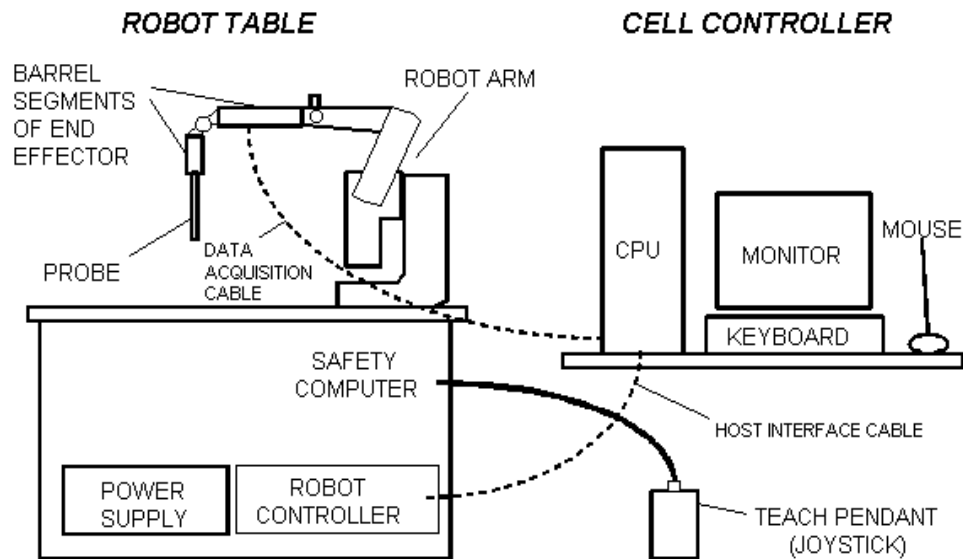
Figure 2. PCTEST Robotics SAR Test Measurement Set-up
