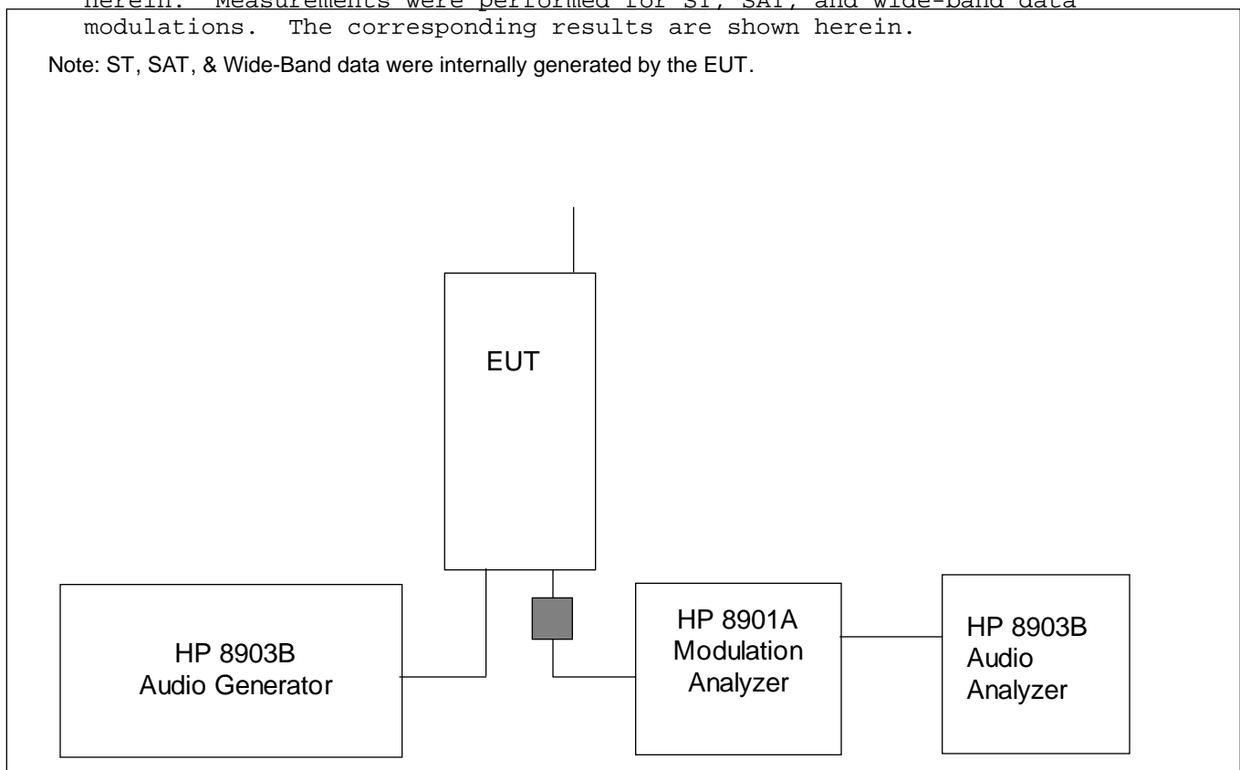
Fig. 3. Transmitter Audio Frequency & Tone Modulation Test Setup. © 2000 PCTEST Lab FCC ID: A3LSC855 SAMSUNG Dual-Mode Cellular Phone (AMPS/CDMA)
