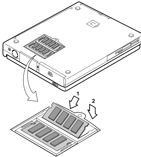
Figure 22. Installing a Memory Module
