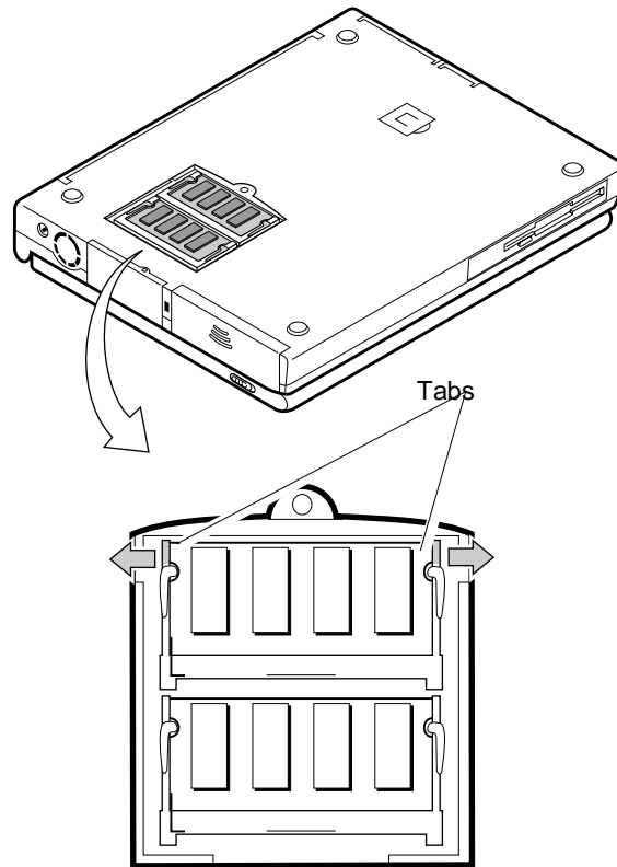
Figure 21. Removing a Memory Module
