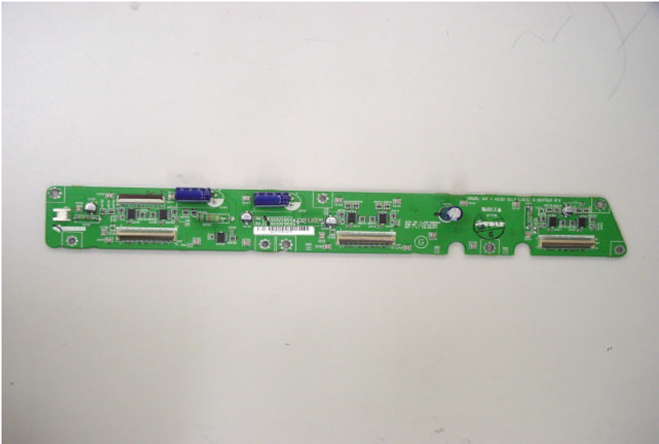
Logic-G-buffer board top view
