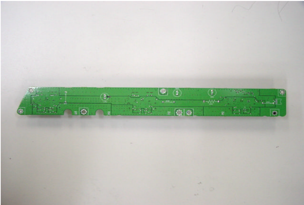
Logic-G-buffer board bottom view
