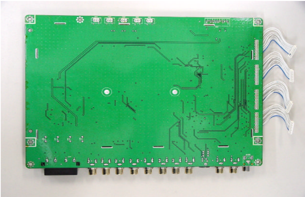
Analog visual board bottom view
