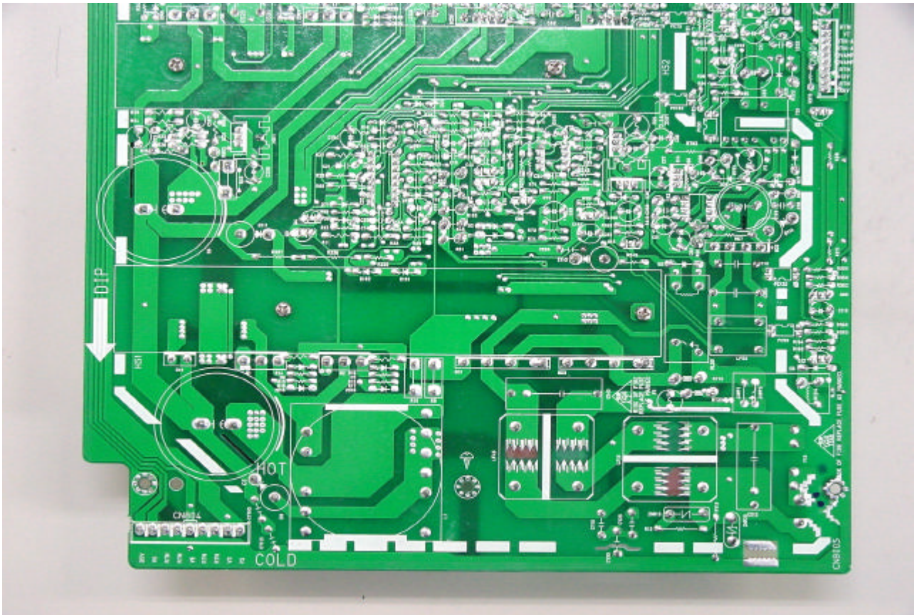
SMPS board - 1 bottom view
