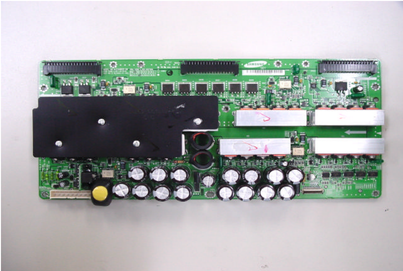
X-driver board top view
