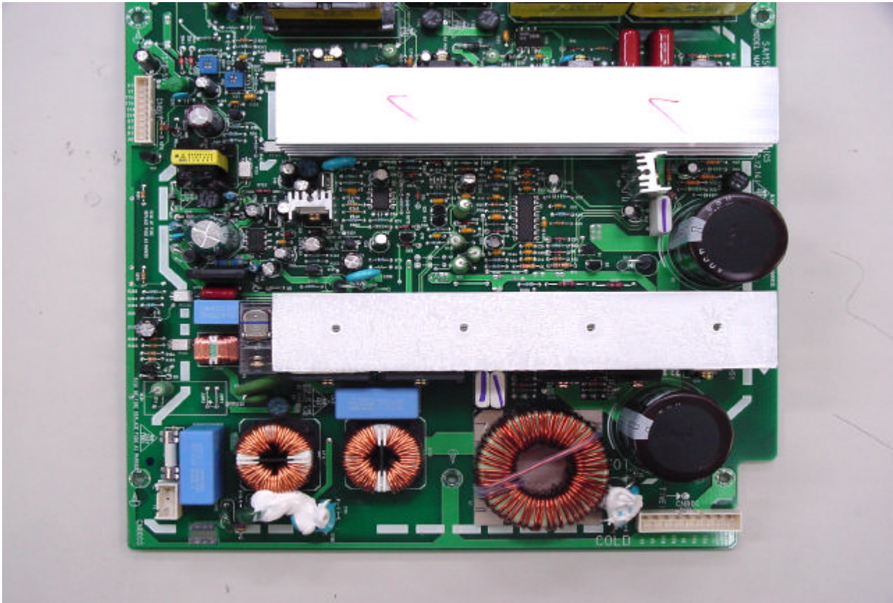
SMPS board - 1 top view
