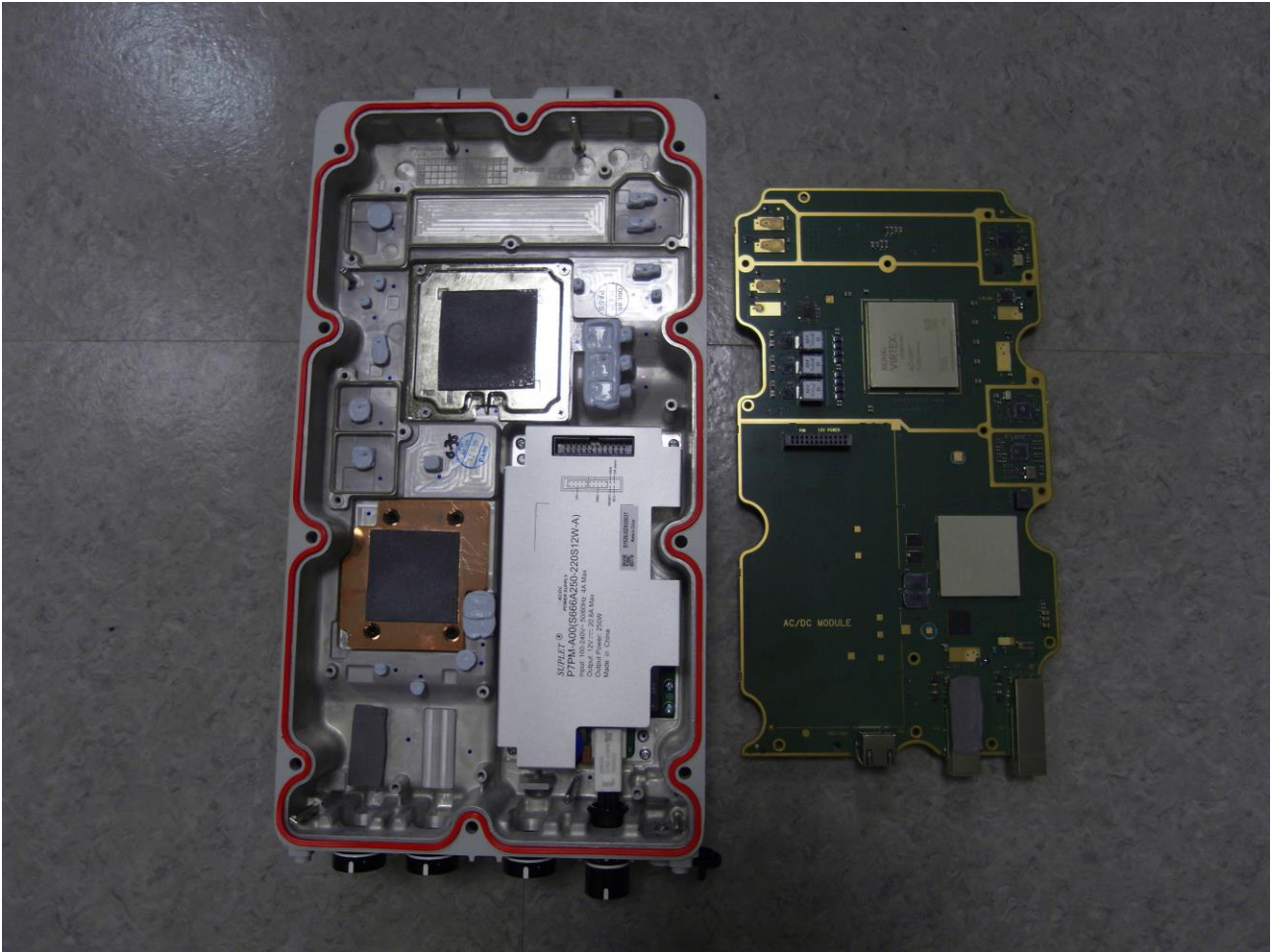
confidential Rear housing PBA component side view
