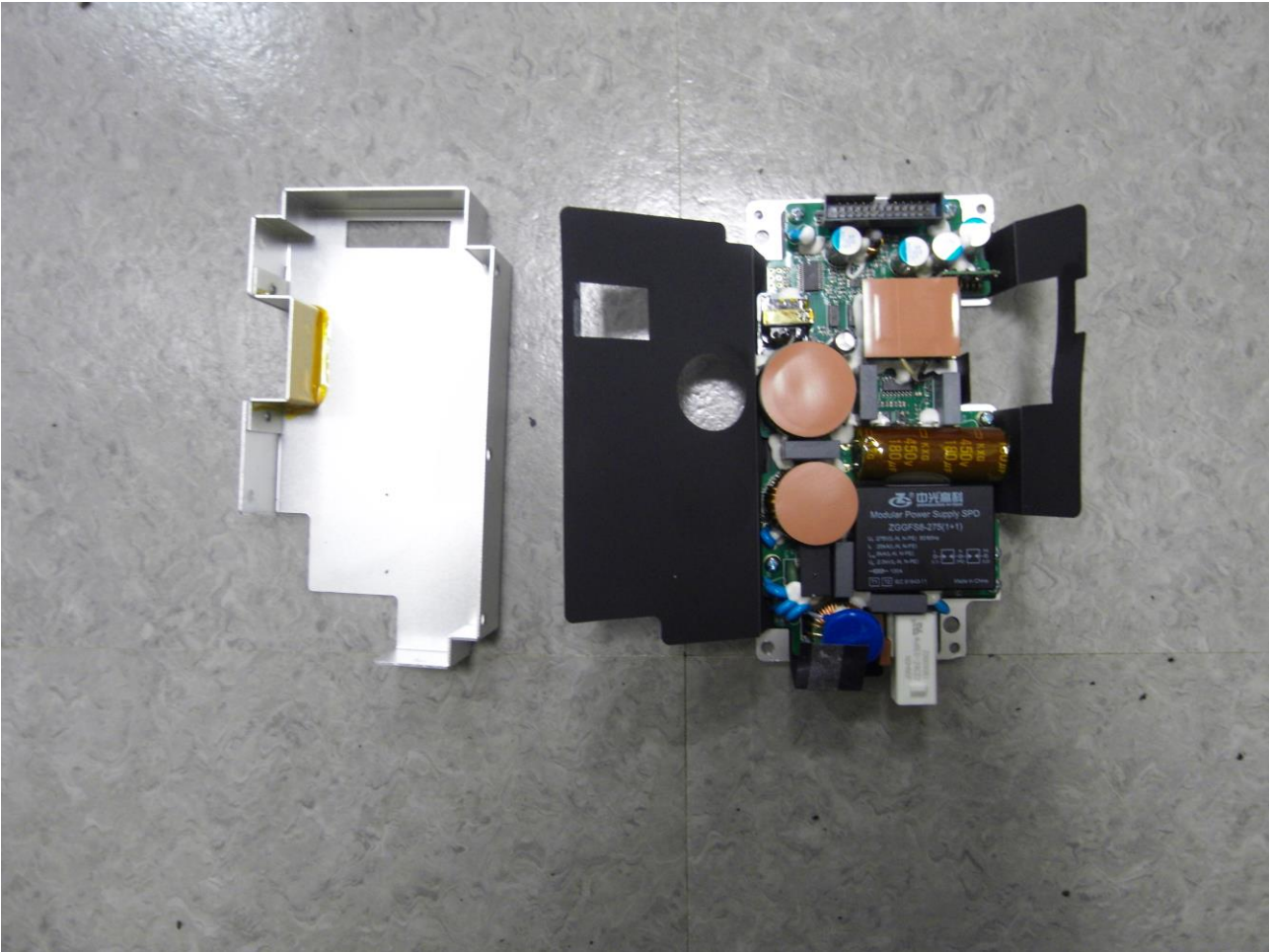
confidential Internal view of ACDC view
