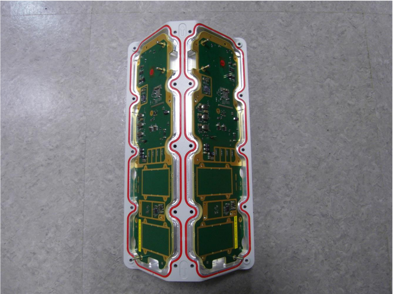
confidential Front housing PBA view without shield can view
