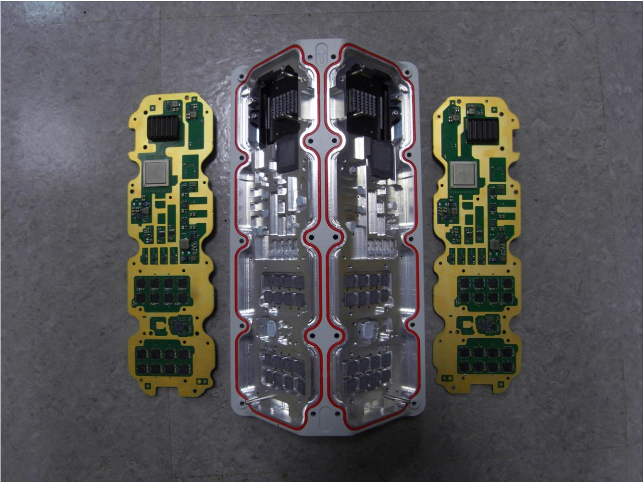
confidential Front housing PBA componet side view
