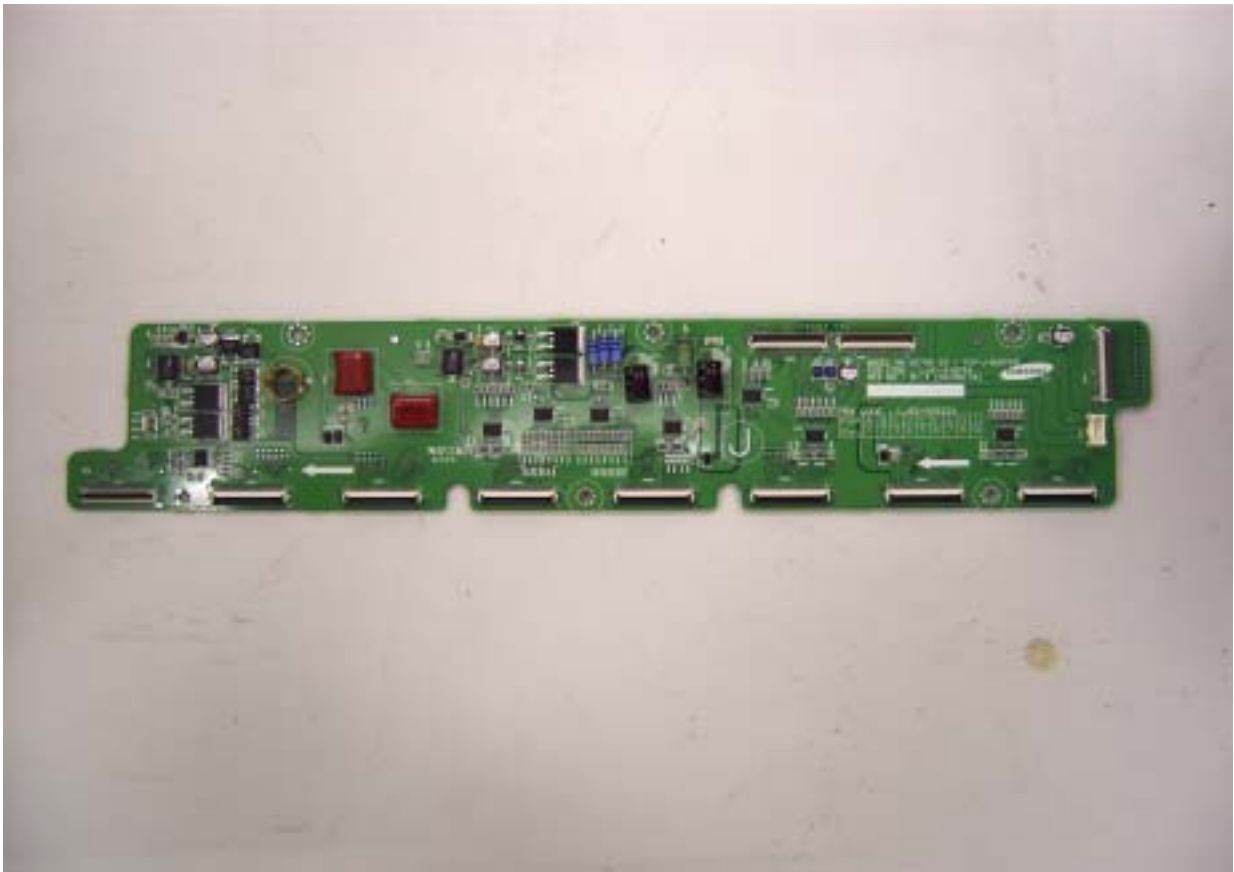
J Buffer board top view
