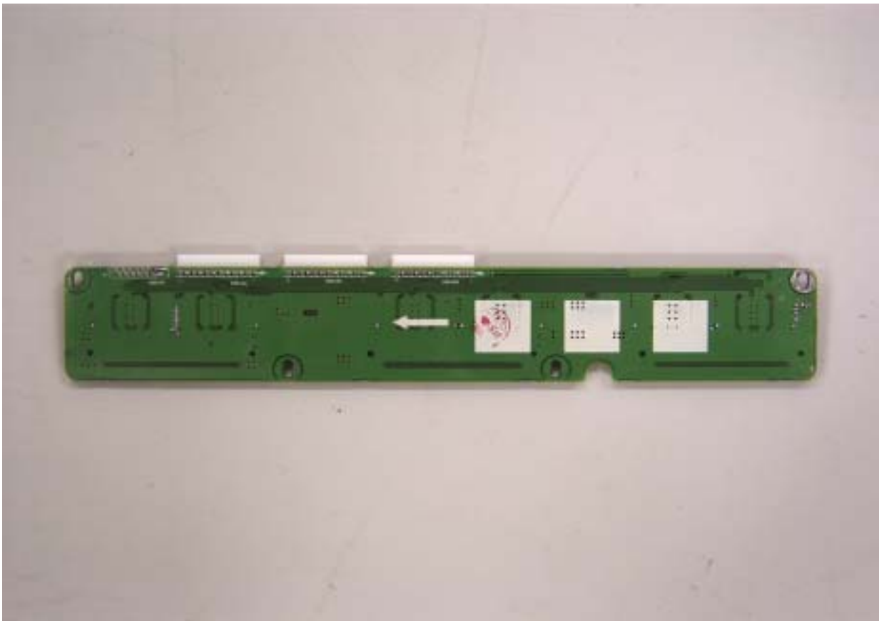
Upper board bottom view
