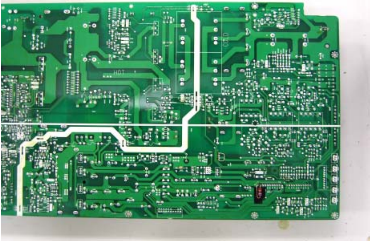
SMPS board bottom view
