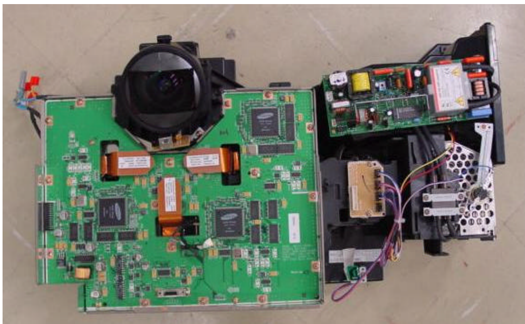
Top view of Drive B'd & Balast engine part
