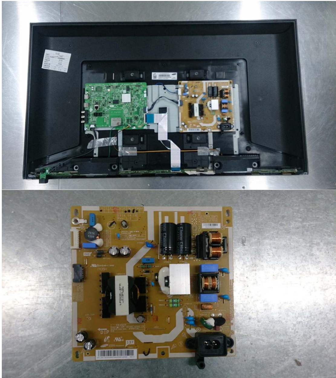
(Power Board)
