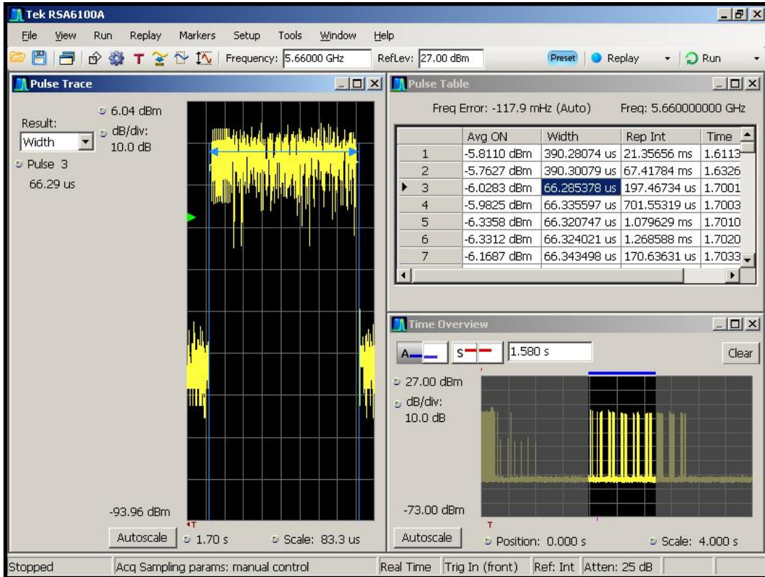
Figure 6-6. Pulse width analysis using Pulse Table and Pulse Trace Function
