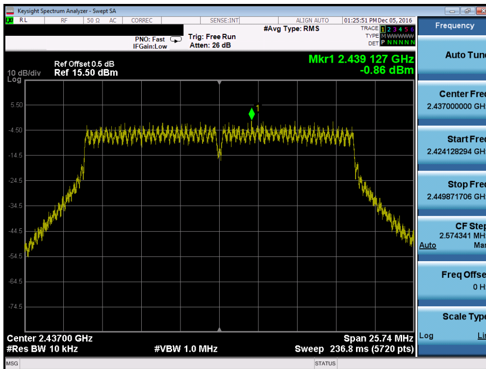
Plot 7-74. Power Spectral Density Plot (802.11n (2.4GHz) – Ch. 6)
