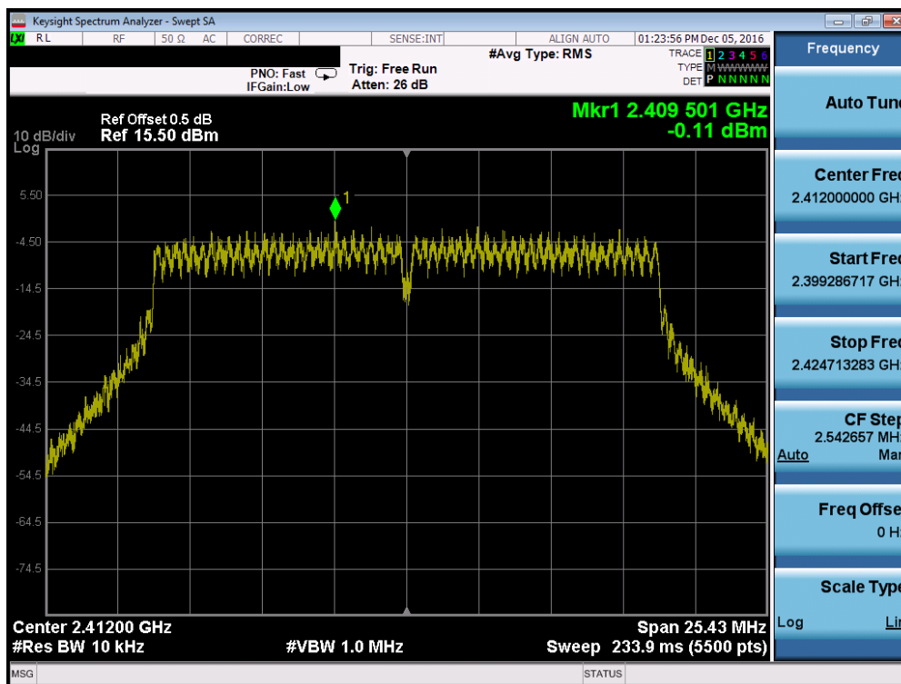
Plot 7-73. Power Spectral Density Plot (802.11n (2.4GHz) – Ch. 1)
