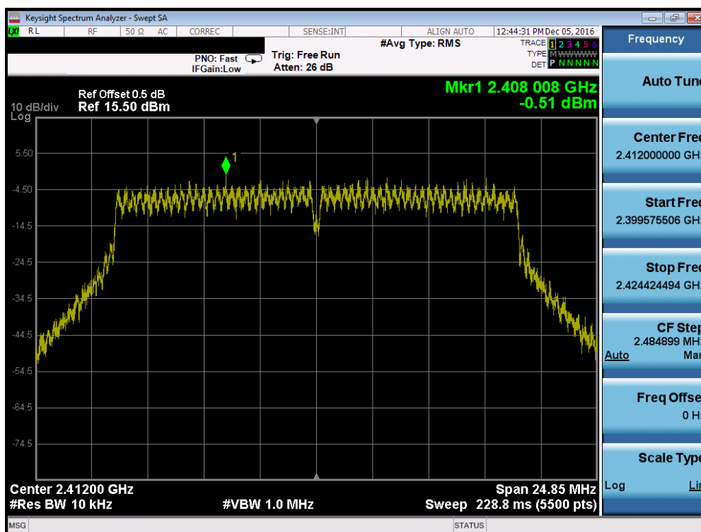
Plot 7-55. Power Spectral Density Plot (802.11n (2.4GHz) – Ch. 1)
