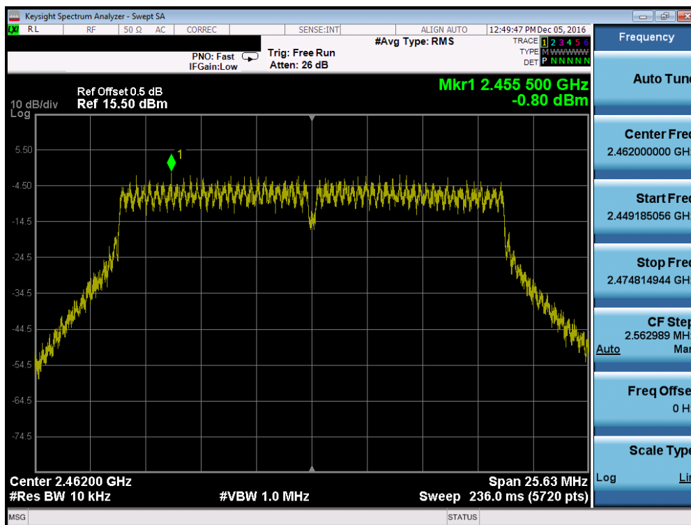
Plot 7-75. Power Spectral Density Plot (802.11n (2.4GHz) – Ch. 11)
