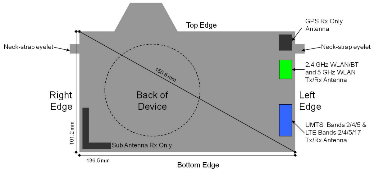
Figure 1-1 DUT Antenna Locations
