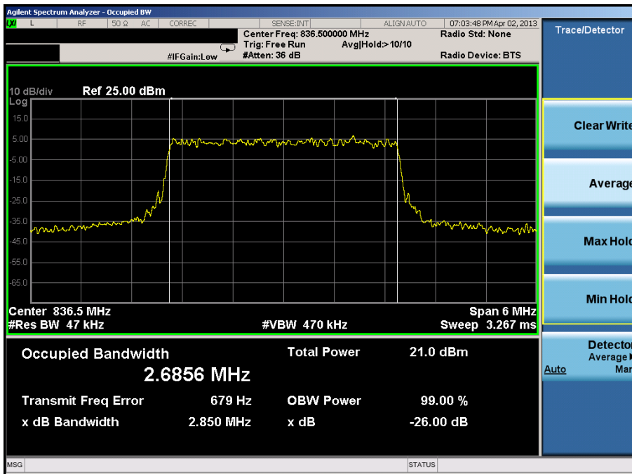
Plot 7-6. Occupied Bandwidth Plot (3.0MHz QPSK – RB Size 15)
