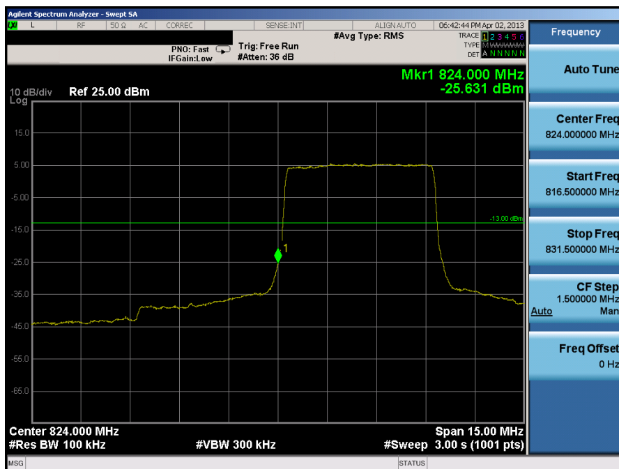
Plot 7-9. Lower Band Edge Plot (5.0MHz QPSK – RB Size 25)
