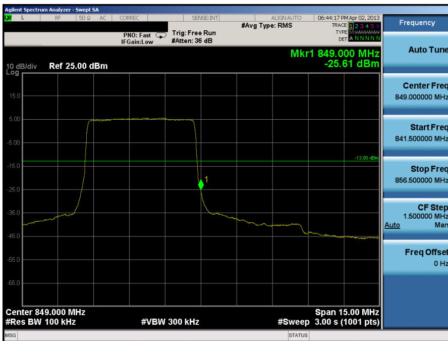
Plot 7-12. Upper Band Edge Plot (5.0MHz QPSK – RB Size 25)
