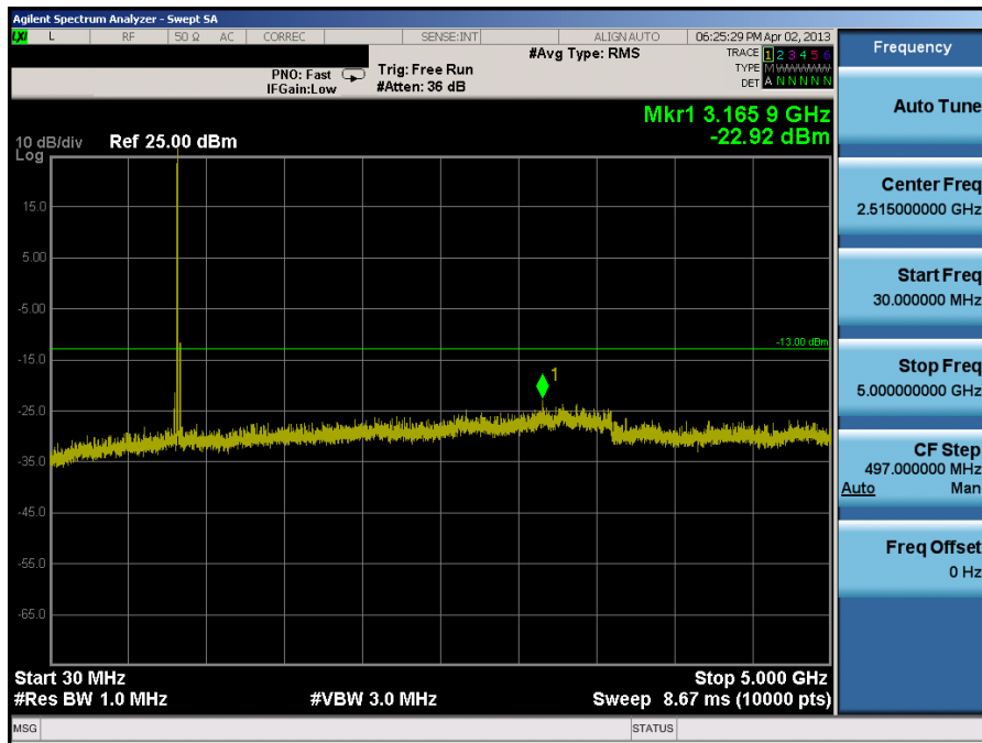
Plot 7-20. Conducted Spurious Plot (10.0MHz QPSK – RB Size 1, RB Offset 0 – High Channel)
