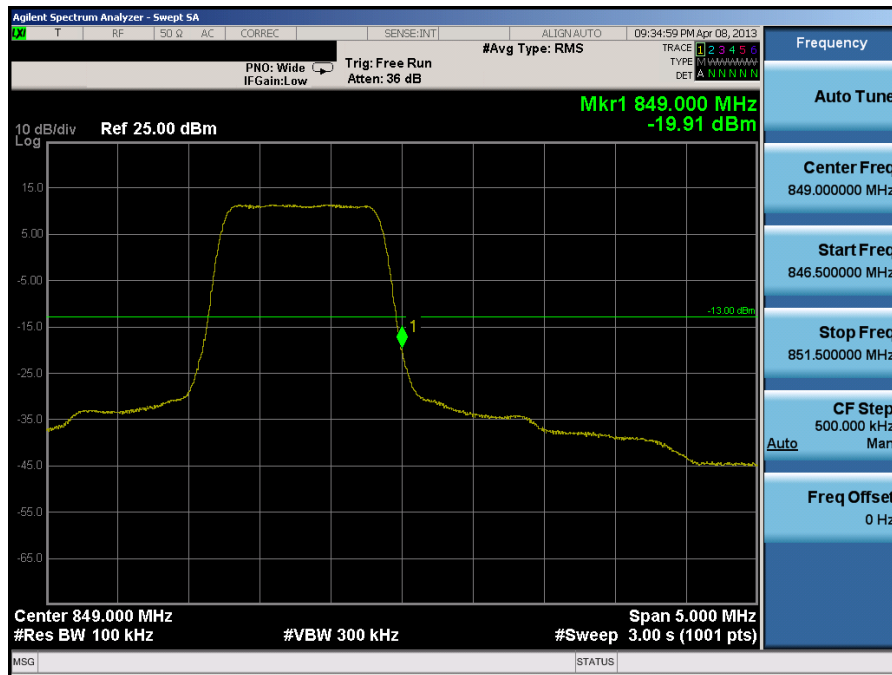
Plot 7-4. Upper Band Edge Plot (1.4MHz QPSK – RB Size 6)
