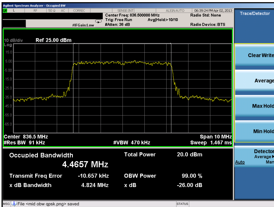
Plot 7-11. Occupied Bandwidth Plot (5.0MHz 16-QAM – RB Size 25)
