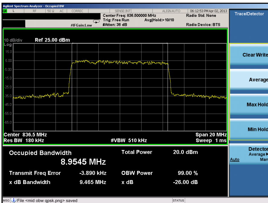
Plot 7-15. Occupied Bandwidth Plot (10.0MHz 16-QAM – RB Size 50)
