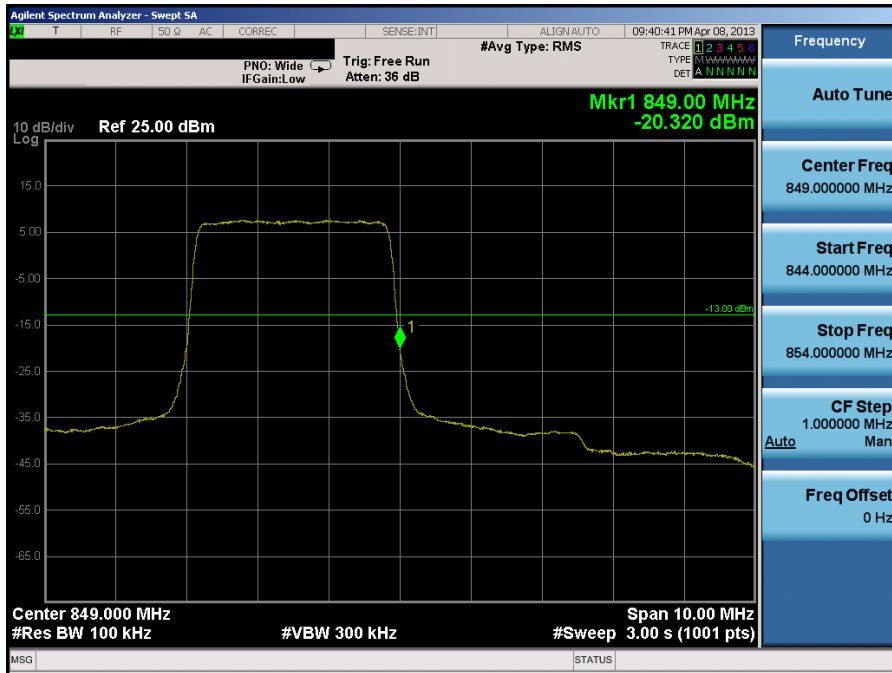
Plot 7-8. Upper Band Edge Plot (3.0MHz QPSK – RB Size 15)
