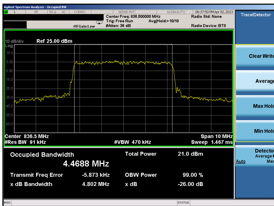
Plot 7-10. Occupied Bandwidth Plot (5.0MHz QPSK – RB Size 25)
