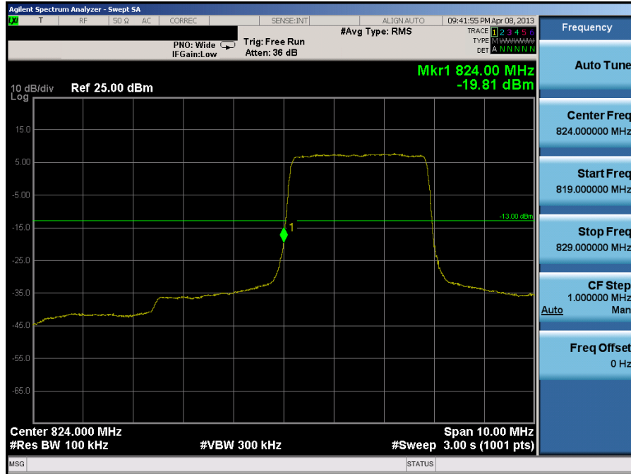
Plot 7-5. Lower Band Edge Plot (3.0MHz QPSK – RB Size 15)
