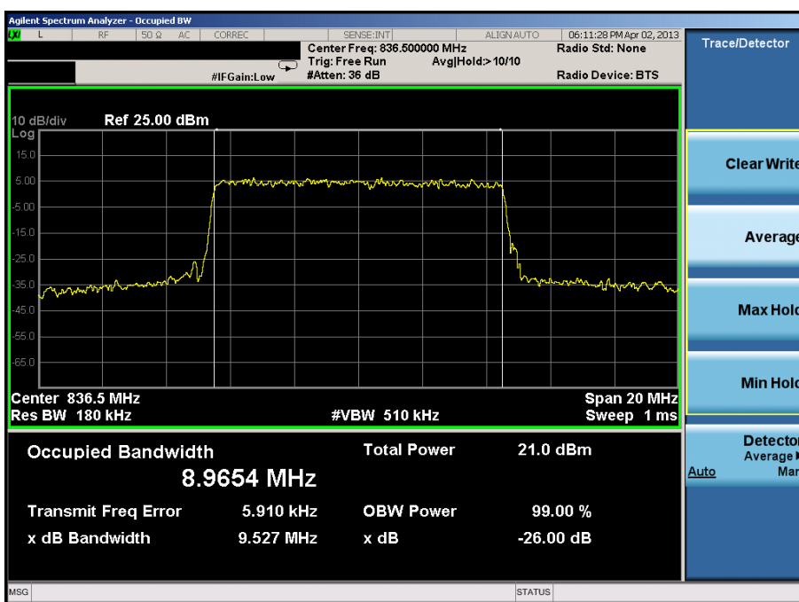
Plot 7-14. Occupied Bandwidth Plot (10.0MHz QPSK – RB Size 50)
