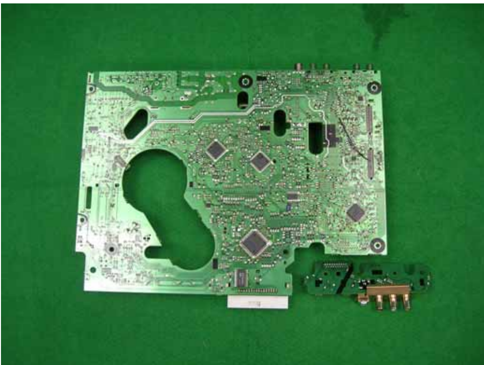
BOTTOM OF MAIN PCB VIEW
