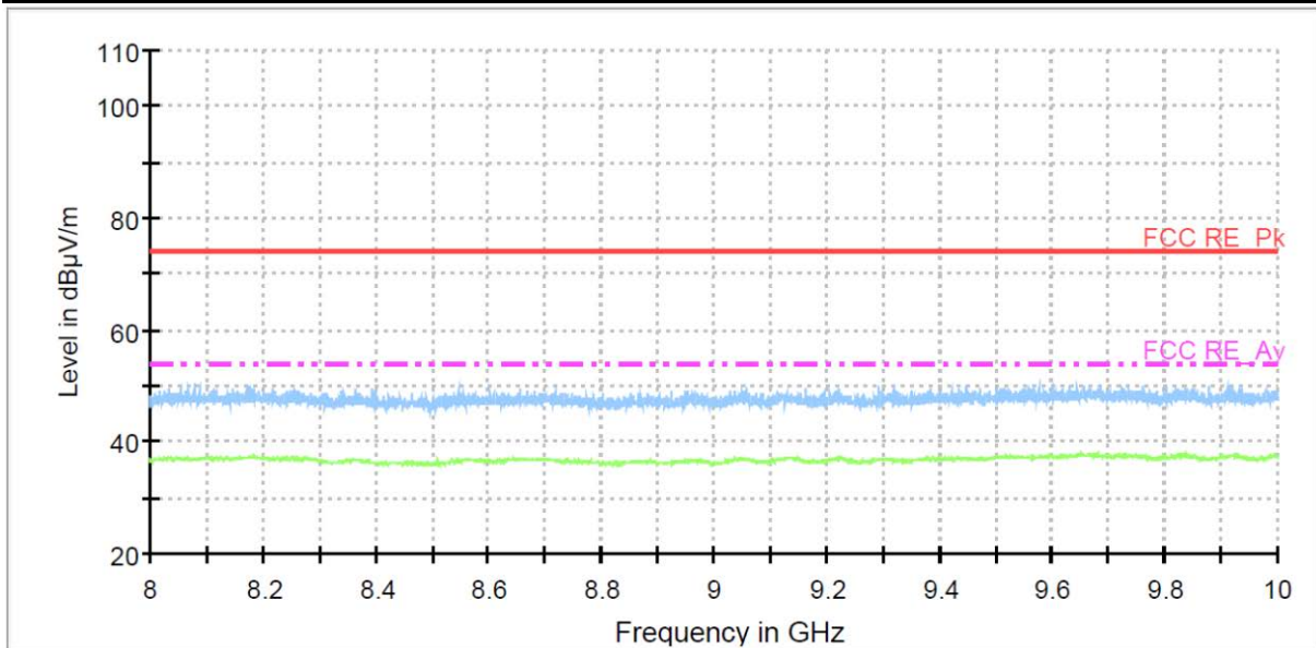
Worst Channel (916 MHz) : Above 1GHz to 10 th Harmonic of highest fundamental frequency
