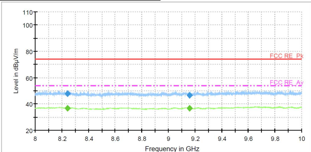
Worst channel 916.00 MHz : 8 GHz to 10 GHz
