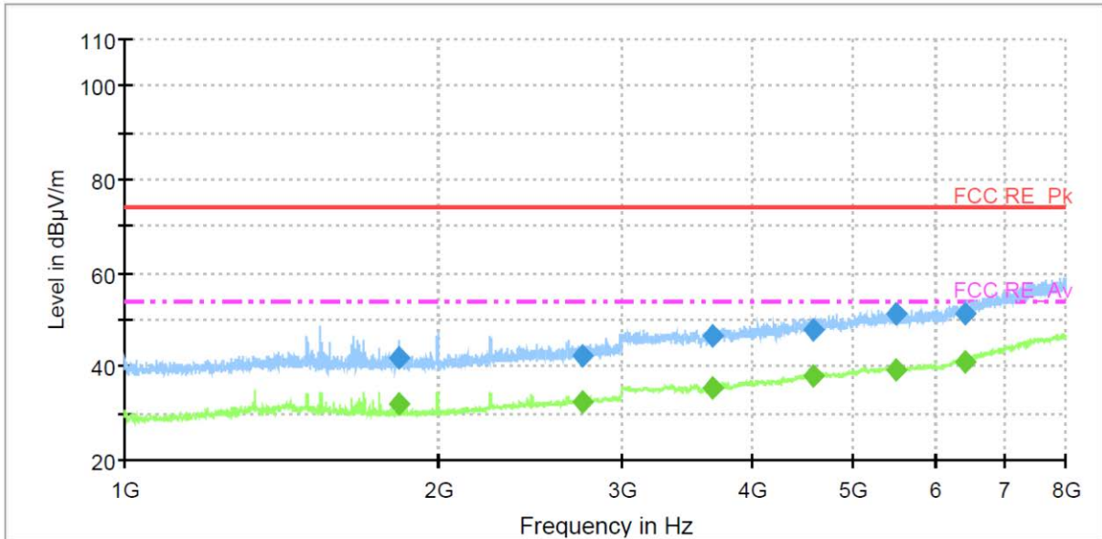
Worst channel 916.00 MHz : 1 GHz to 8 GHz
