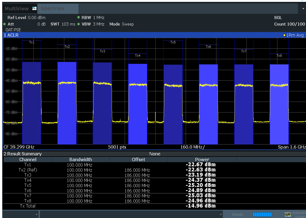
Plot 7-51. Antenna A EIRP Density Plot (100 MHz BW 8CC NC 64QAM High Channel)
