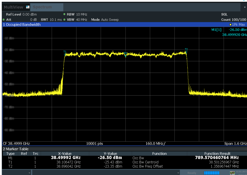
Plot 7-5. Occupied Bandwidth Plot (100 MHz BW 8CC 16QAM Mid Channel)
