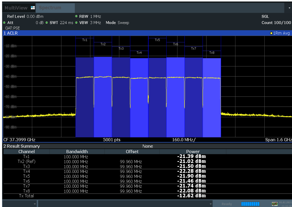
Plot 7-109. Antenna D EIRP Density Plot (100 MHz BW 8CC QPSK Low Channel)
