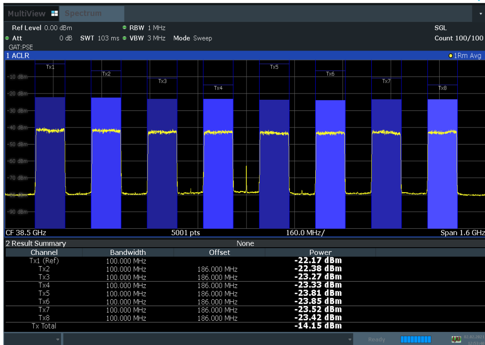
Plot 7-41. Antenna A EIRP Density Plot (100 MHz BW 8CC NC 16QAM Mid Channel)
