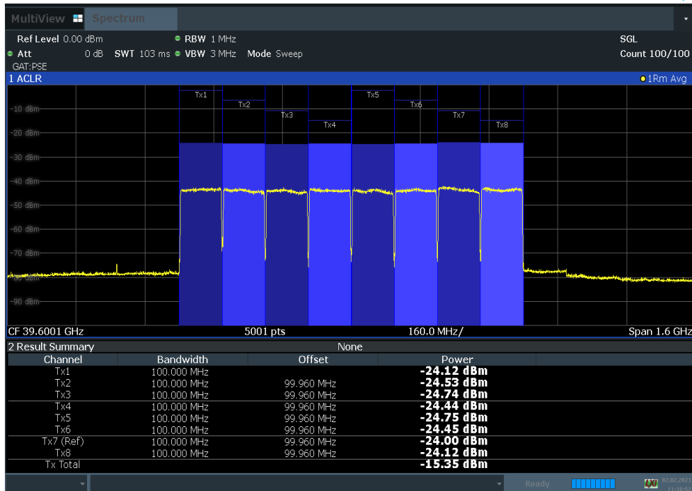
Plot 7-73. Antenna B EIRP Density Plot (100 MHz BW 8CC QPSK High Channel)
