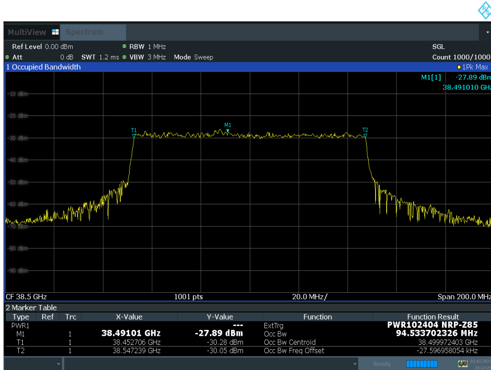
Plot 7-19. Occupied Bandwidth Plot (100 MHz BW 1CC QPSK Mid Channel)
