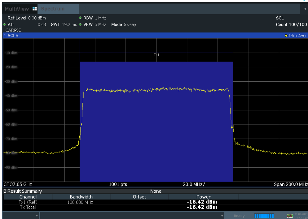
Plot 7-80. Antenna C EIRP Density Plot (100 MHz BW 1CC 16QAM Low Channel)
