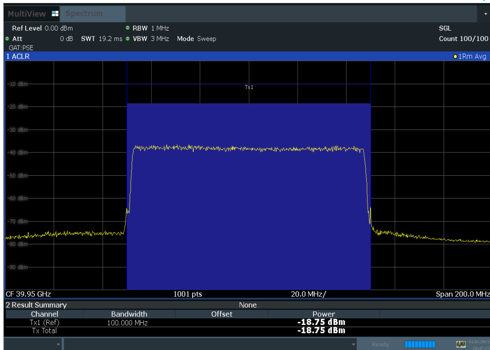
Plot 7-72. Antenna B EIRP Density Plot (100 MHz 1CC BW 64QAM High Channel)
