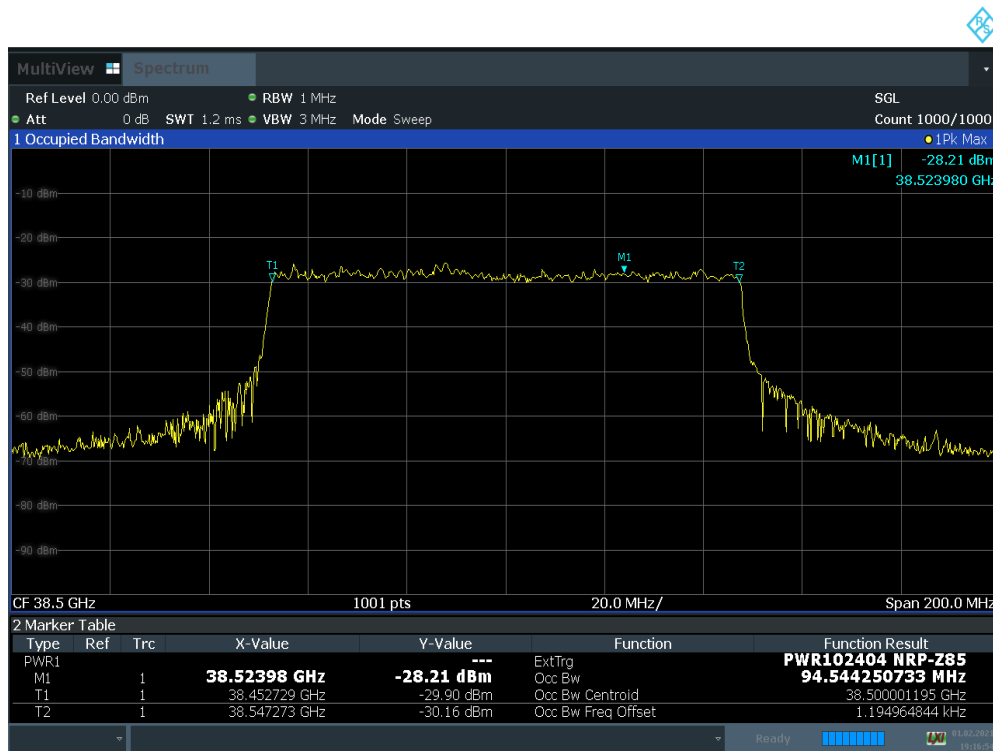
Plot 7-7. Occupied Bandwidth Plot (100 MHz BW 1CC QPSK Mid Channel)
