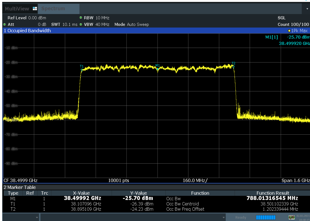
Plot 7-18. Occupied Bandwidth Plot (100 MHz BW 8CC 64QAM Mid Channel)
