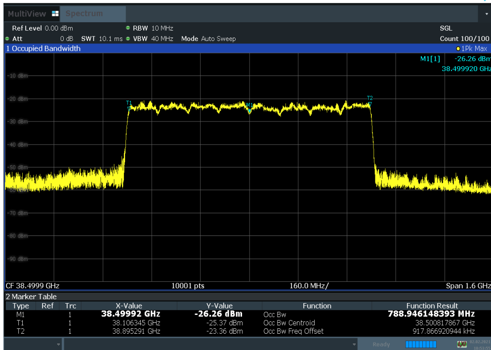
Plot 7-4. Occupied Bandwidth Plot (100 MHz BW 8CC QPSK Mid Channel)
