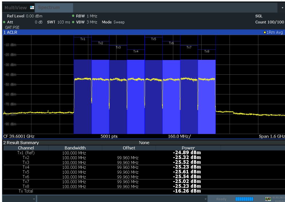
Plot 7-102. Antenna C EIRP Density Plot (100 MHz BW 8CC 64QAM High Channel)
