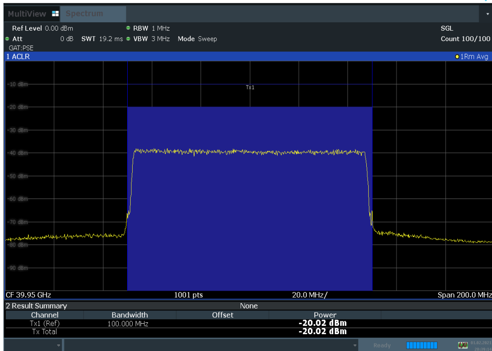
Plot 7-99. Antenna C EIRP Density Plot (100 MHz 1CC BW 64QAM High Channel)
