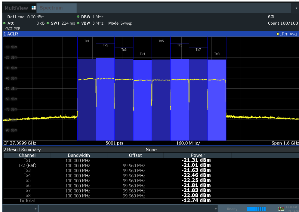
Plot 7-55. Antenna B EIRP Density Plot (100 MHz BW 8CC QPSK Low Channel)
