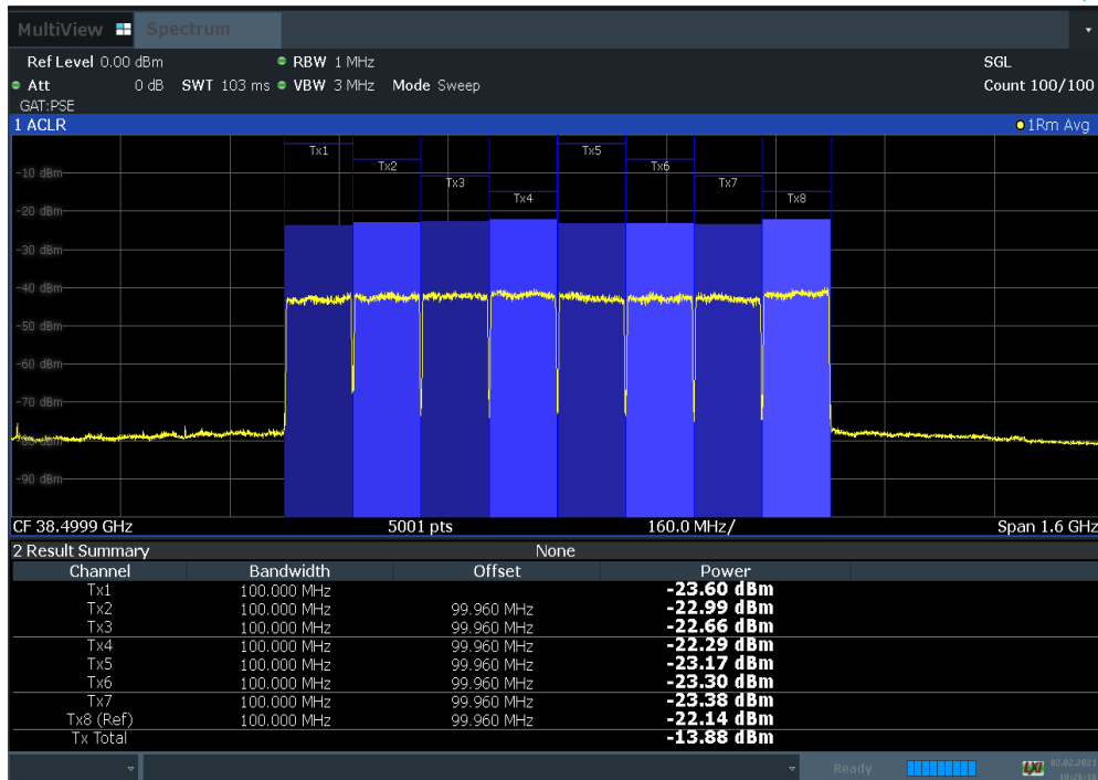
Plot 7-92. Antenna C EIRP Density Plot (100 MHz BW 8CC 16QAM Mid Channel)
