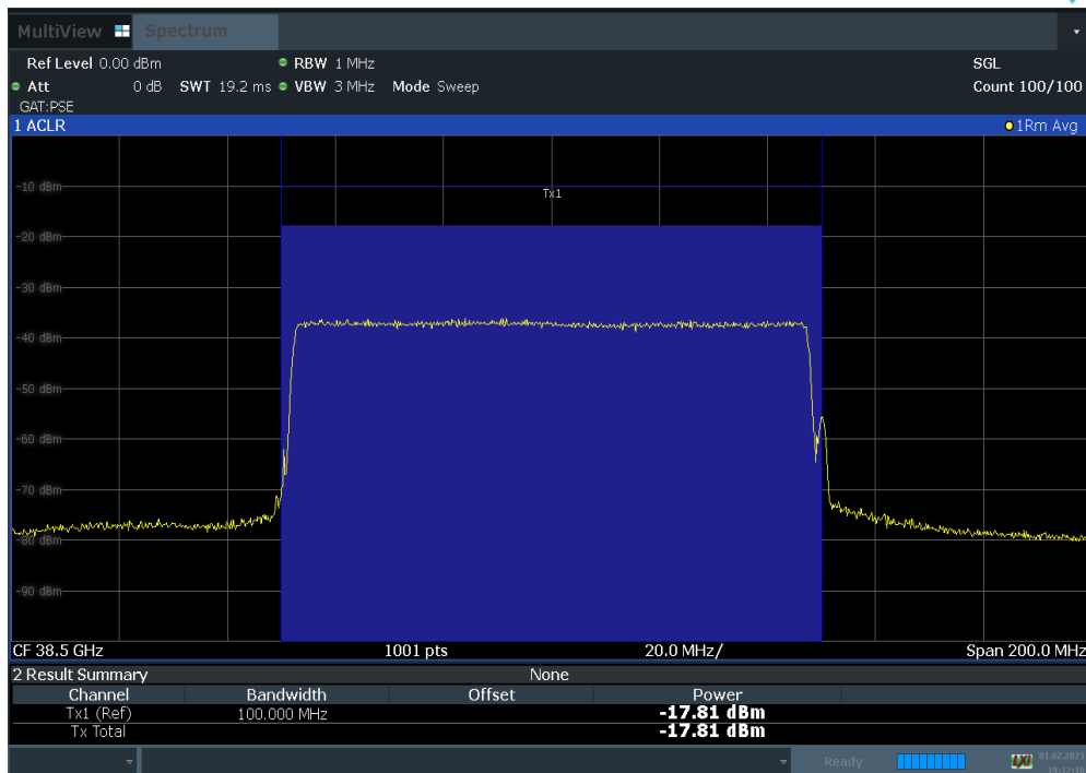
Plot 7-115. Antenna D EIRP Density Plot (100 MHz BW 1CC QPSK Mid Channel)
