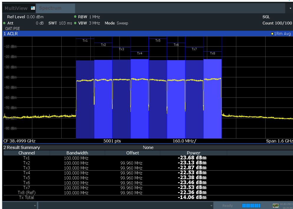
Plot 7-91. Antenna C EIRP Density Plot (100 MHz BW 8CC QPSK Mid Channel)
