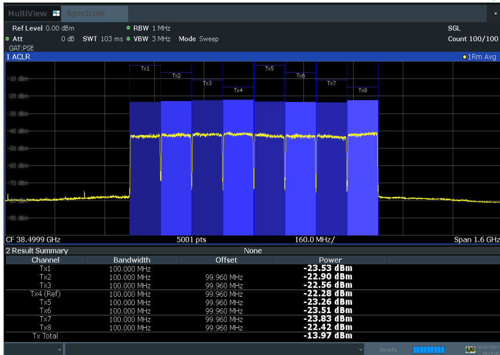
Plot 7-65. Antenna B EIRP Density Plot (100 MHz BW 8CC 16QAM Mid Channel)
