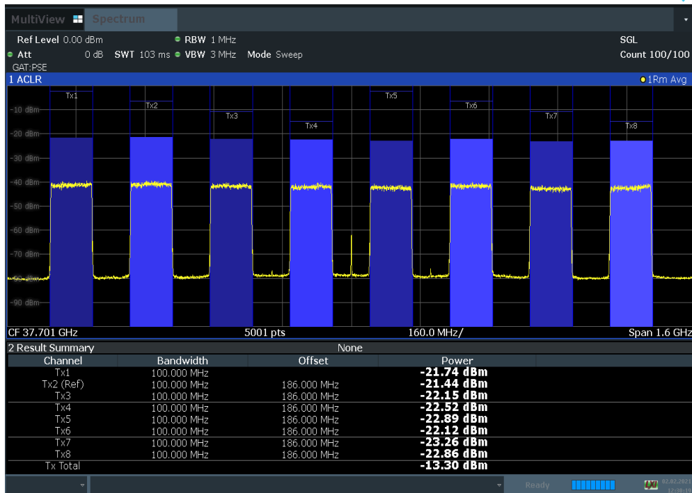
Plot 7-114. Antenna D EIRP Density Plot (100 MHz BW 8CC NC 64QAM Low Channel)
