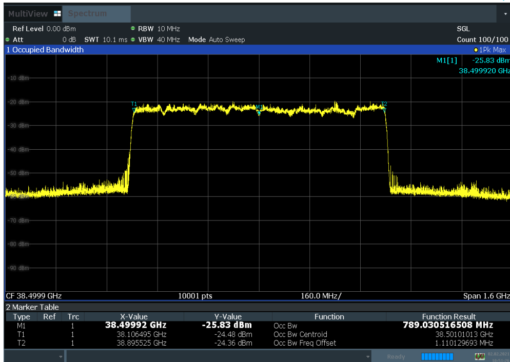
Plot 7-11. Occupied Bandwidth Plot (100 MHz BW 8CC 16QAM Mid Channel)
