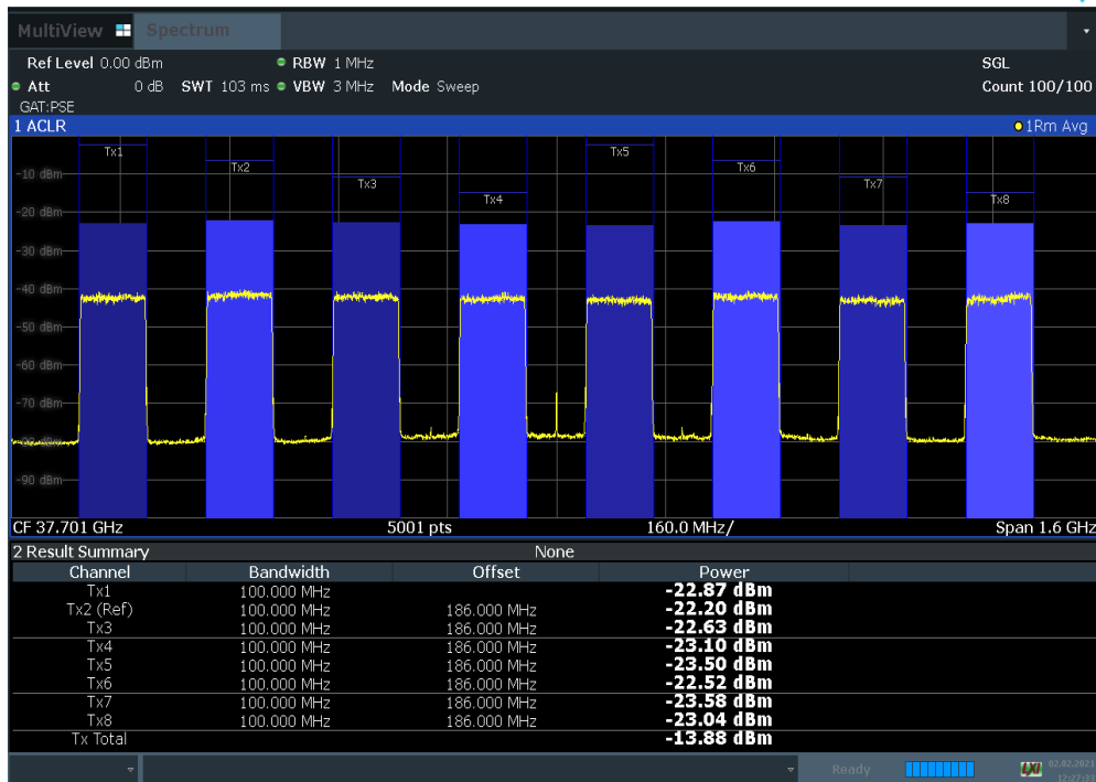
Plot 7-33. Antenna A EIRP Density Plot (100 MHz BW 8CC NC 64QAM Low Channel)
