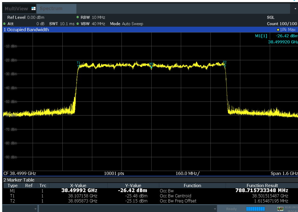
Plot 7-17. Occupied Bandwidth Plot (100 MHz BW 8CC 16QAM Mid Channel)
