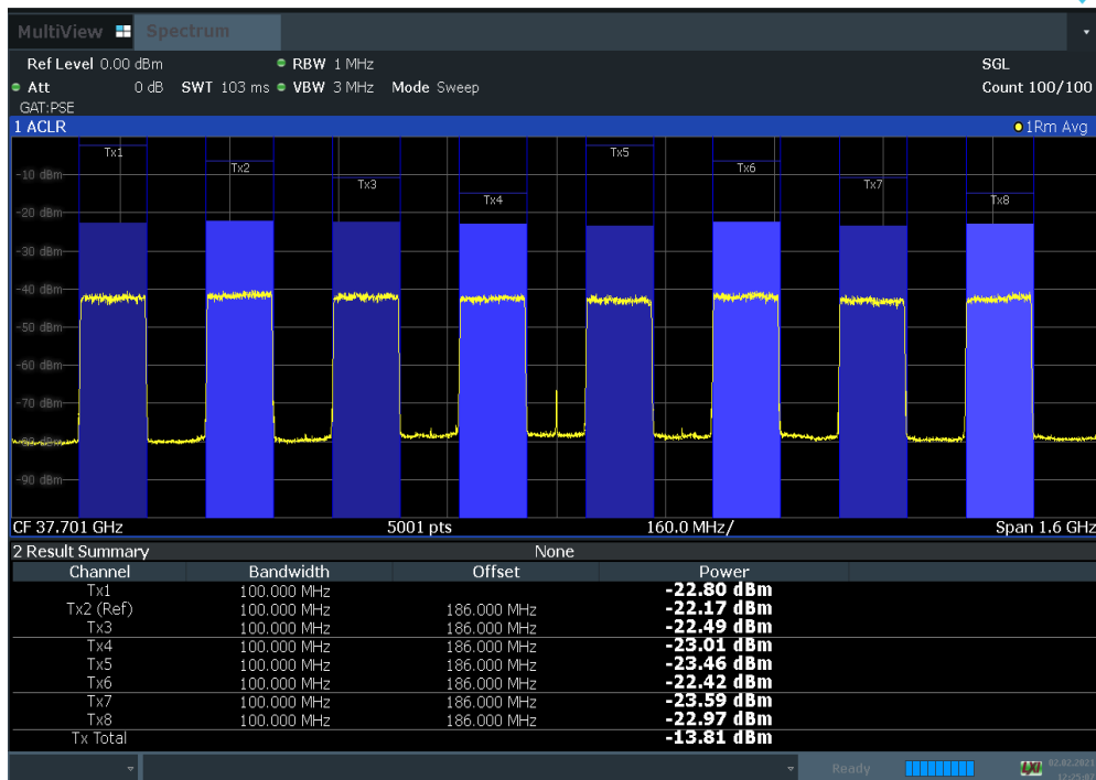
Plot 7-32. Antenna A EIRP Density Plot (100 MHz BW 8CC NC 16QAM Low Channel)
