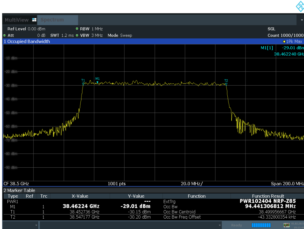
Plot 7-13. Occupied Bandwidth Plot (100 MHz BW 1CC QPSK Mid Channel)
