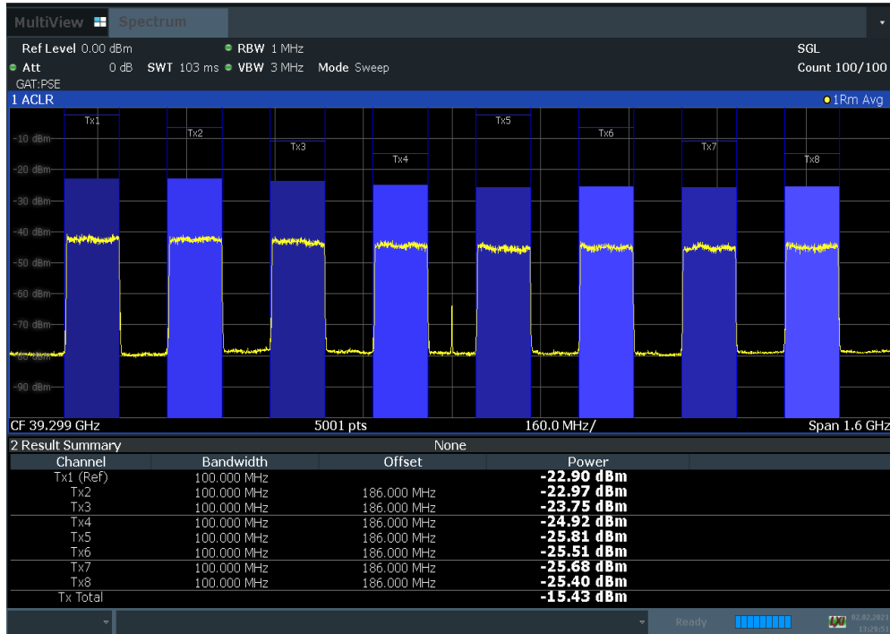
Plot 7-105. Antenna C EIRP Density Plot (100 MHz BW 8CC NC 64QAM High Channel)
