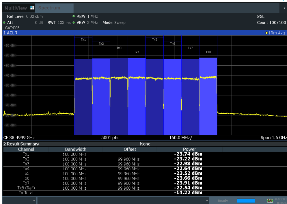
Plot 7-39. Antenna A EIRP Density Plot (100 MHz BW 8CC 64QAM Mid Channel)
