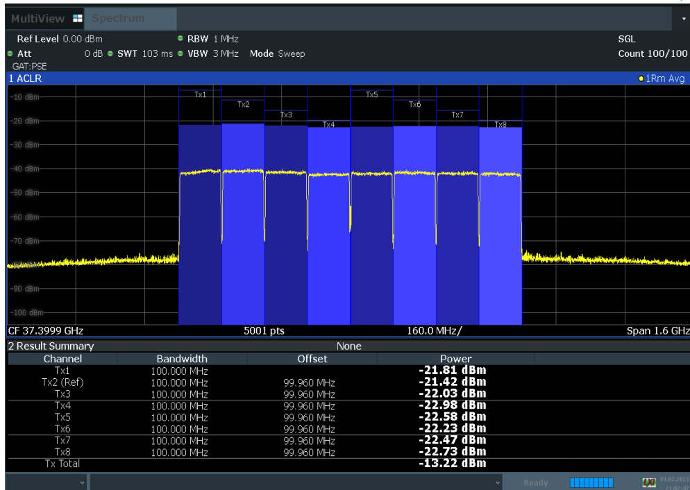
Plot 7-28. Antenna A EIRP Density Plot (100 MHz BW 8CC QPSK Low Channel)
