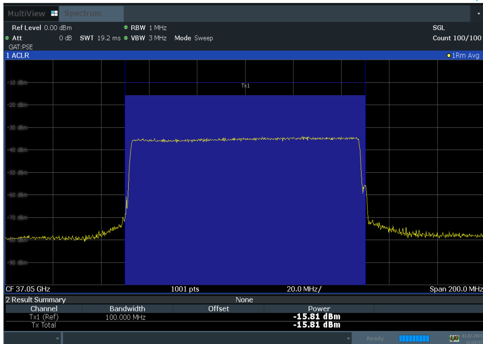
Plot 7-106. Antenna D EIRP Density Plot (100 MHz BW 1CC QPSK Low Channel)
