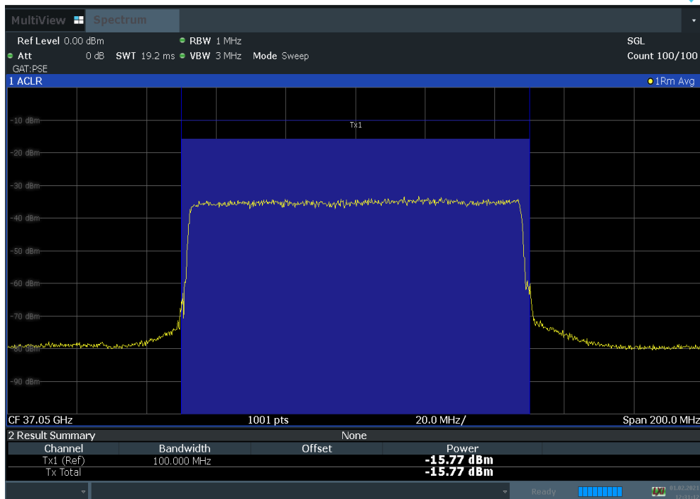
Plot 7-53. Antenna B EIRP Density Plot (100 MHz 1CC BW 16QAM Low Channel)
