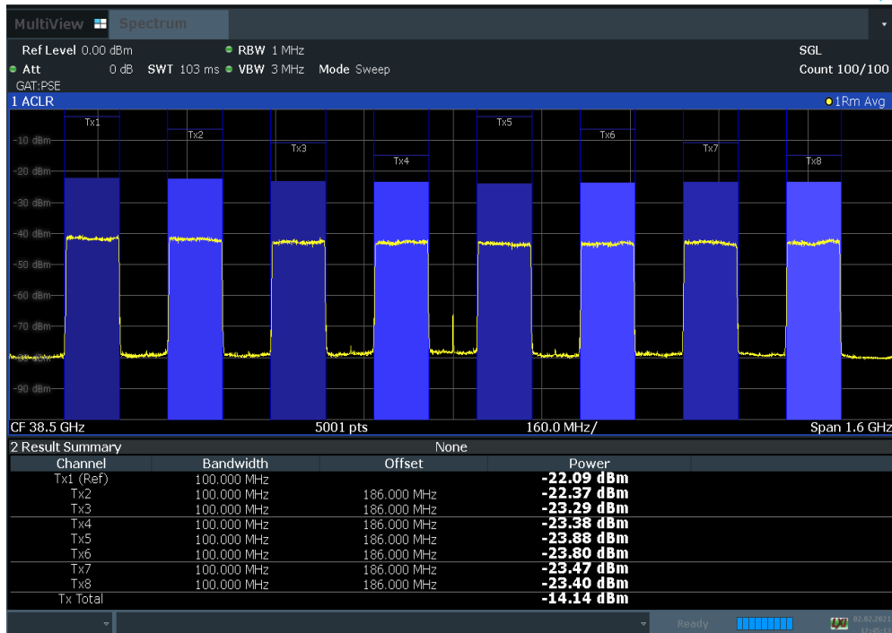
Plot 7-40. Antenna A EIRP Density Plot (100 MHz BW 8CC NC QPSK Mid Channel)
