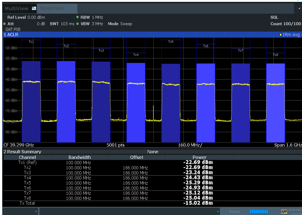
Plot 7-49. Antenna A EIRP Density Plot (100 MHz BW 8CC NC QPSK High Channel)
