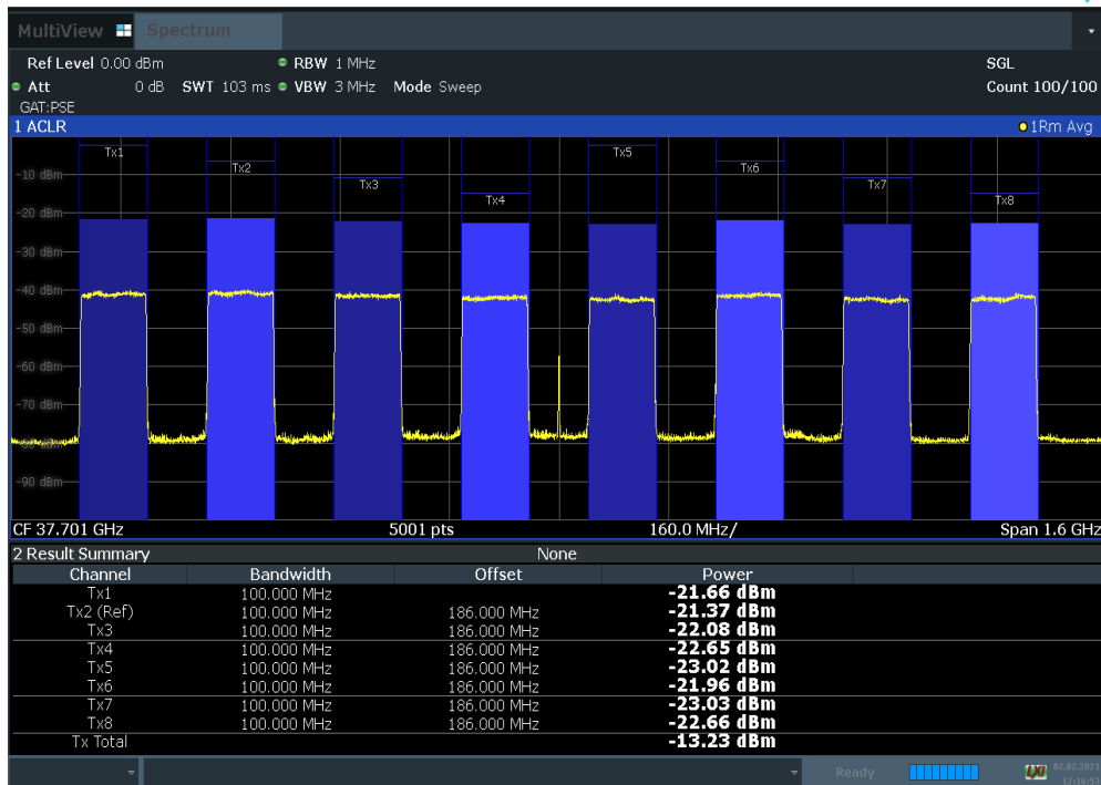
Plot 7-58. Antenna B EIRP Density Plot (100 MHz BW 8CC NC QPSK Low Channel)
