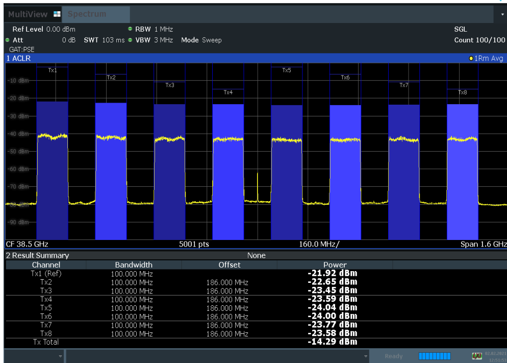
Plot 7-95. Antenna C EIRP Density Plot (100 MHz BW 8CC NC 16QAM Mid Channel)
