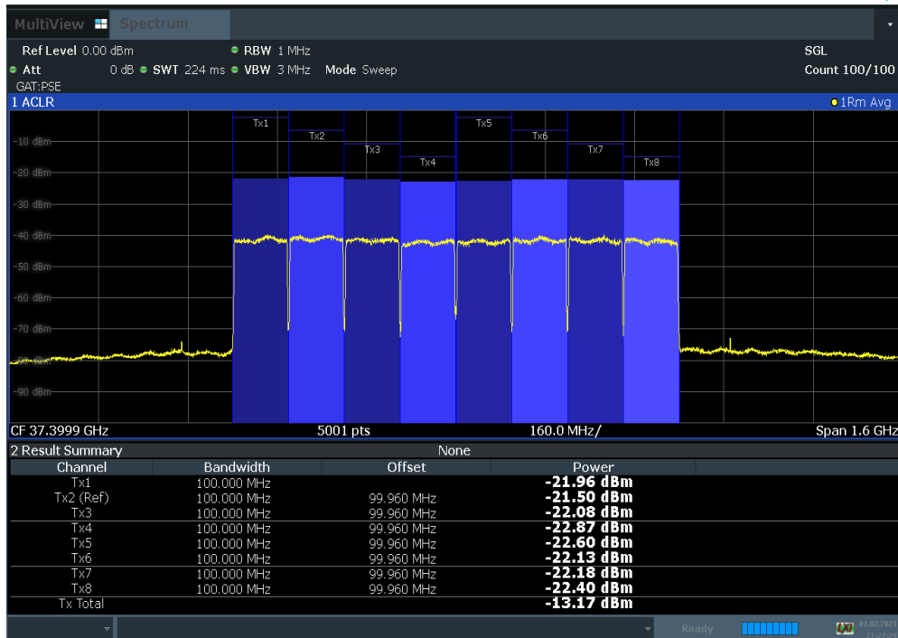
Plot 7-84. Antenna C EIRP Density Plot (100 MHz BW 8CC 64QAM Low Channel)
