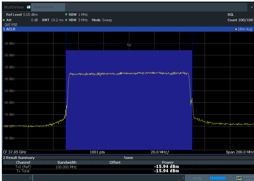
Plot 7-27. Antenna A EIRP Density Plot (100 MHz 1CC BW 64QAM Low Channel)
