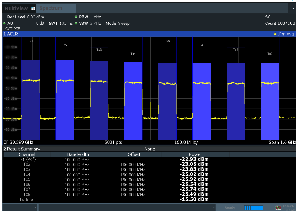
Plot 7-103. Antenna C EIRP Density Plot (100 MHz BW 8CC NC QPSK High Channel)
