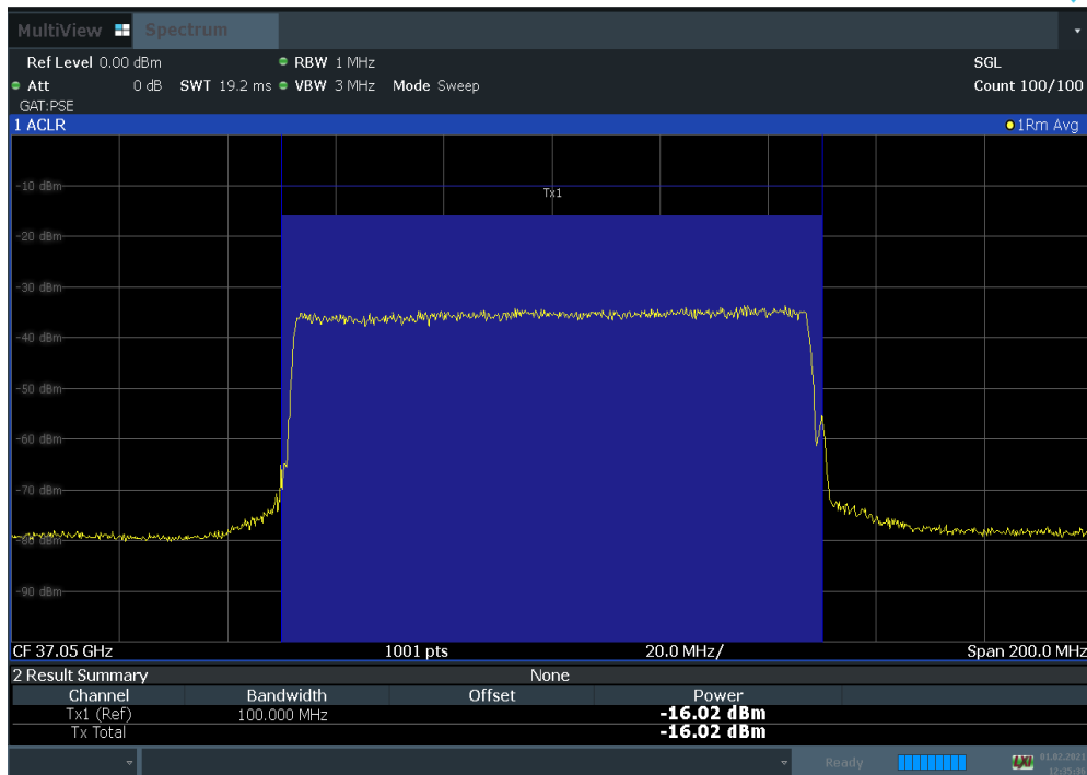
Plot 7-108. Antenna D EIRP Density Plot (100 MHz 1CC BW 64QAM Low Channel)
