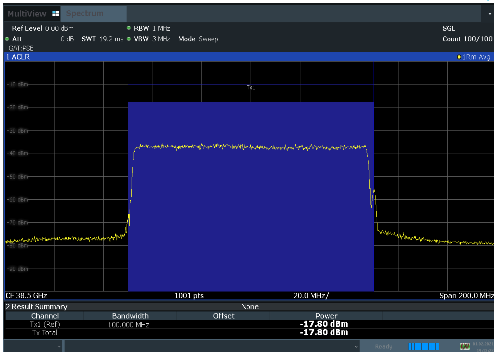
Plot 7-116. Antenna D EIRP Density Plot (100 MHz 1CC BW 16QAM Mid Channel)
