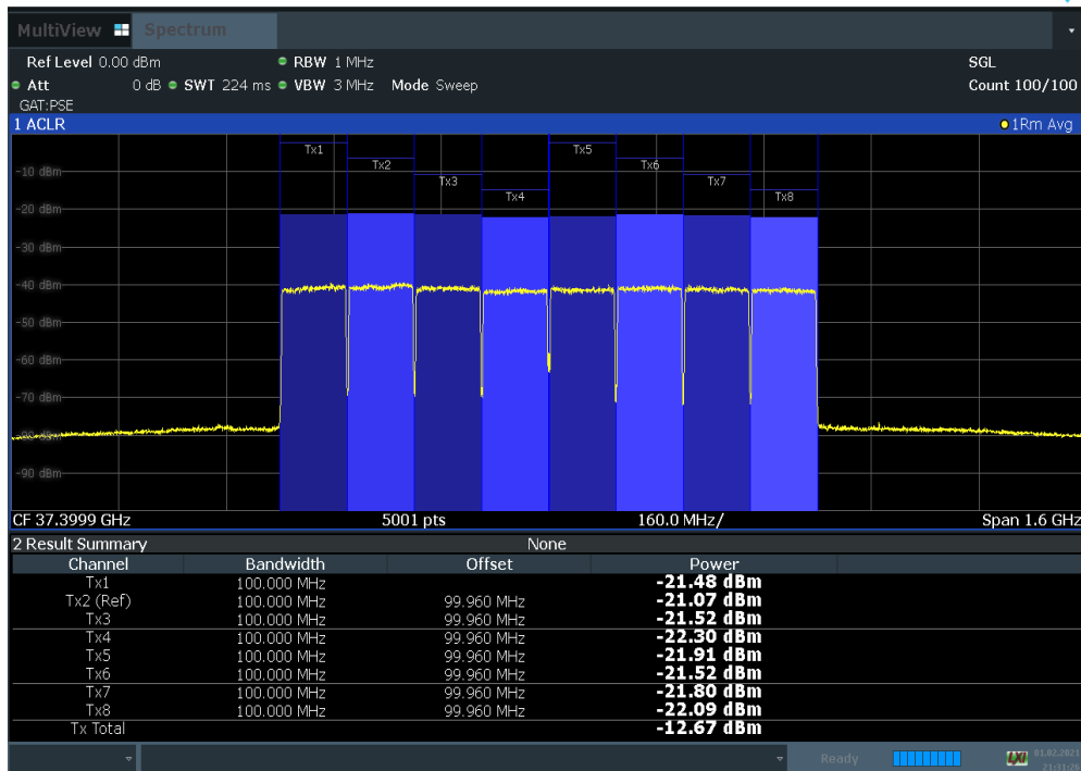
Plot 7-110. Antenna D EIRP Density Plot (100 MHz BW 8CC 16QAM Low Channel)
