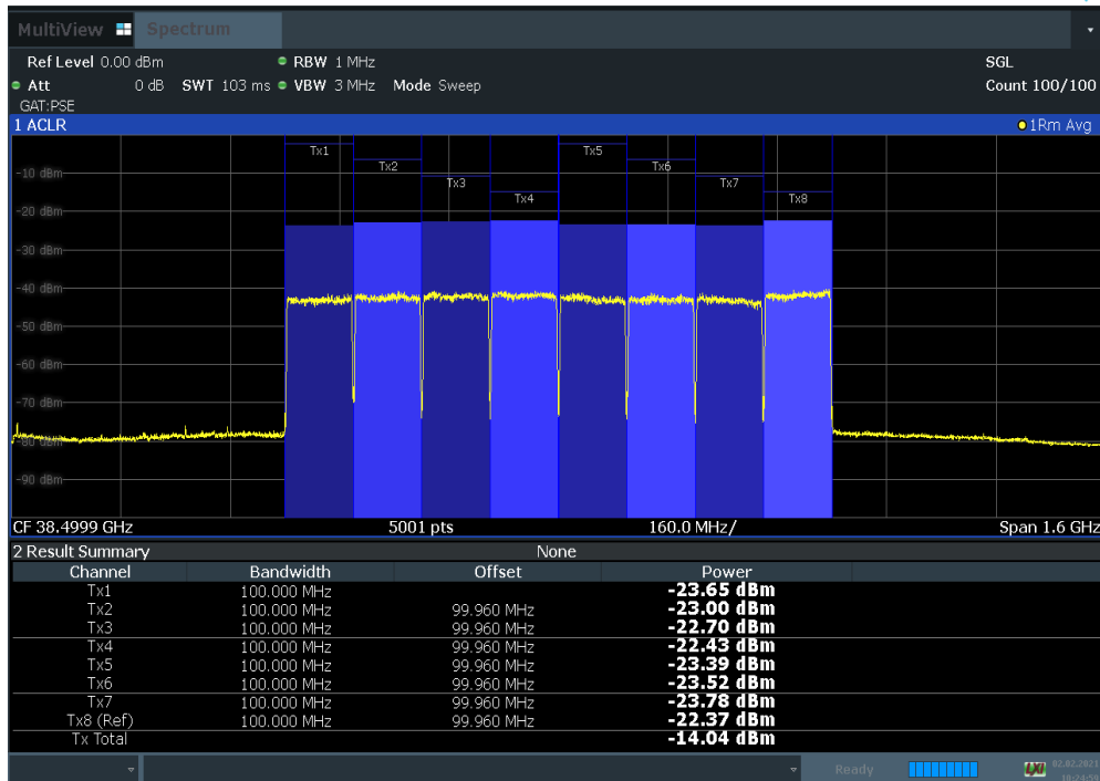
Plot 7-38. Antenna A EIRP Density Plot (100 MHz BW 8CC 16QAM Mid Channel)
