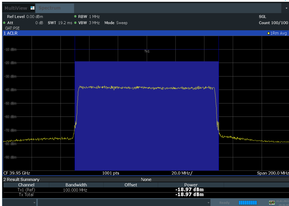
Plot 7-43. Antenna A EIRP Density Plot (100 MHz BW 1CC QPSK High Channel)
