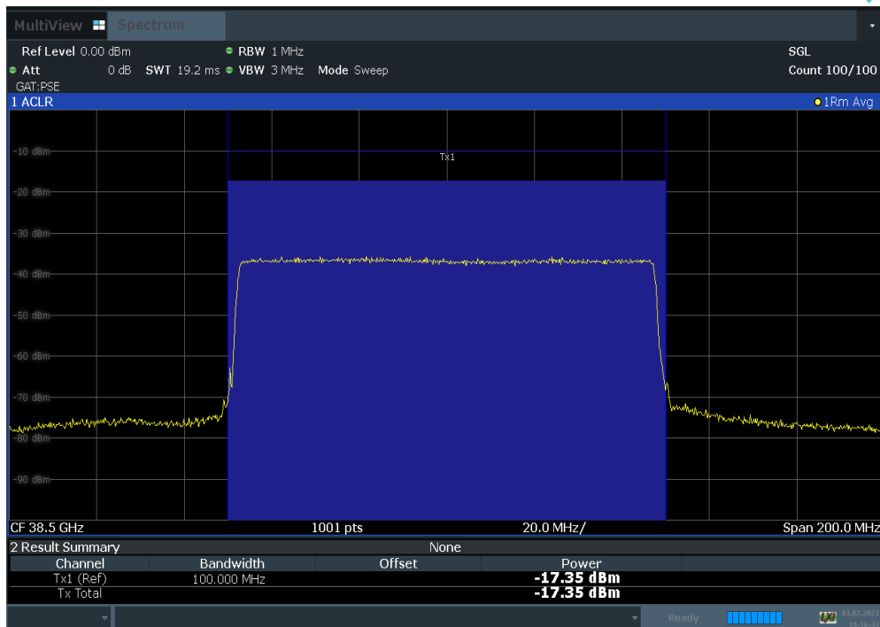
Plot 7-61. Antenna B EIRP Density Plot (100 MHz BW 1CC QPSK Mid Channel)
