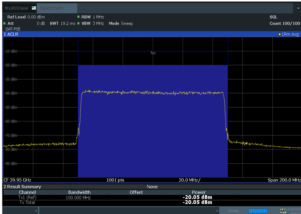
Plot 7-98. Antenna C EIRP Density Plot (100 MHz BW 1CC 16QAM High Channel)
