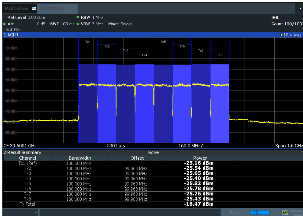
Plot 7-101. Antenna C EIRP Density Plot (100 MHz BW 8CC 16QAM High Channel)
