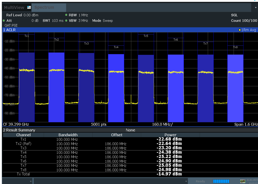
Plot 7-50. Antenna A EIRP Density Plot (100 MHz BW 8CC NC 16QAM High Channel)
