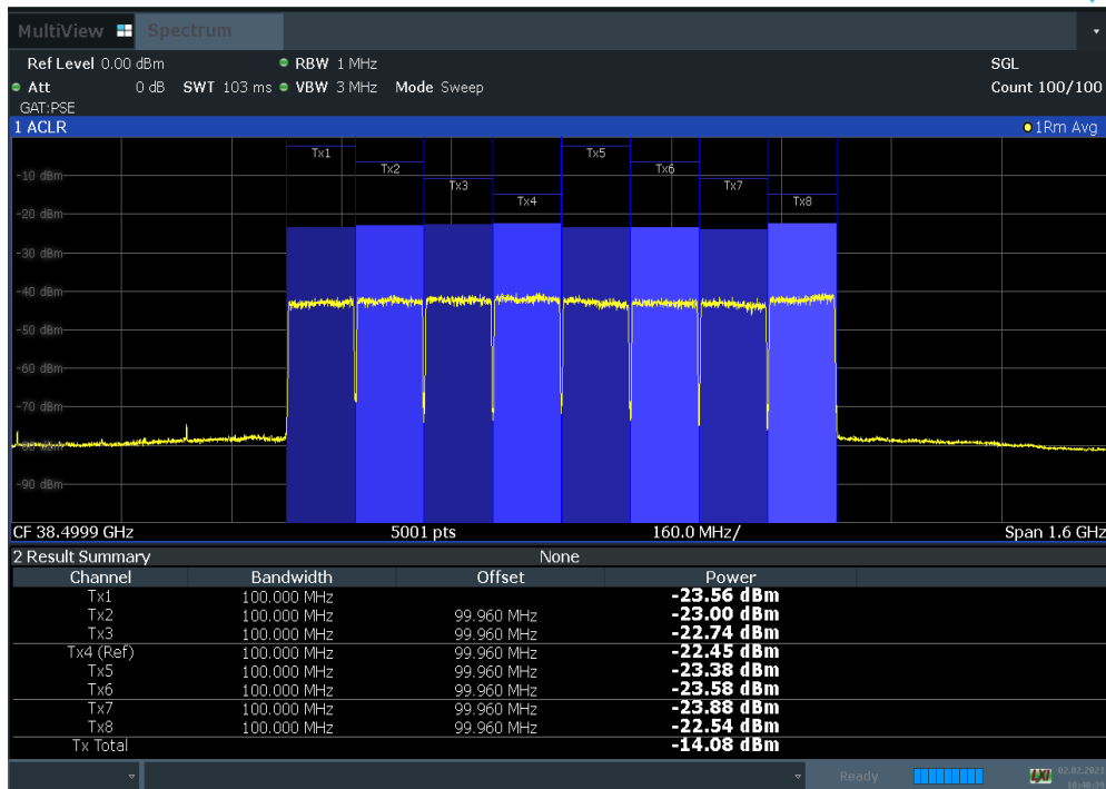
Plot 7-66. Antenna B EIRP Density Plot (100 MHz BW 8CC 64QAM Mid Channel)
