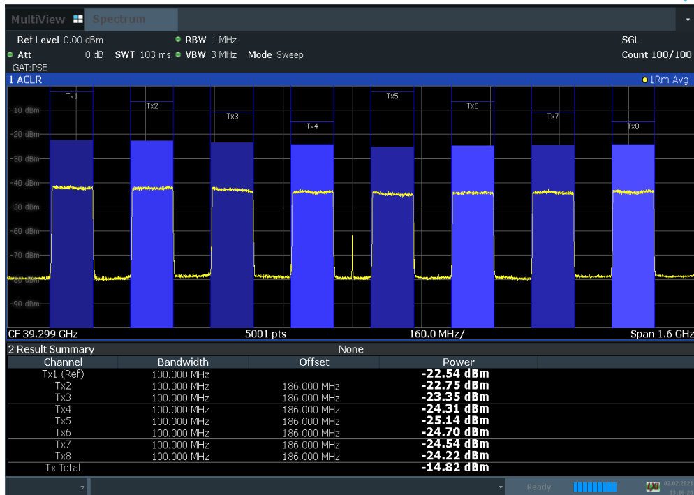
Plot 7-76. Antenna B EIRP Density Plot (100 MHz BW 8CC NC QPSK High Channel)
