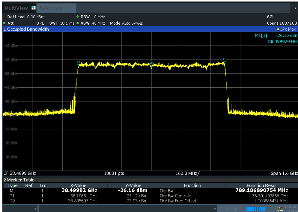
Plot 7-23. Occupied Bandwidth Plot (100 MHz BW 8CC 16QAM Mid Channel)
