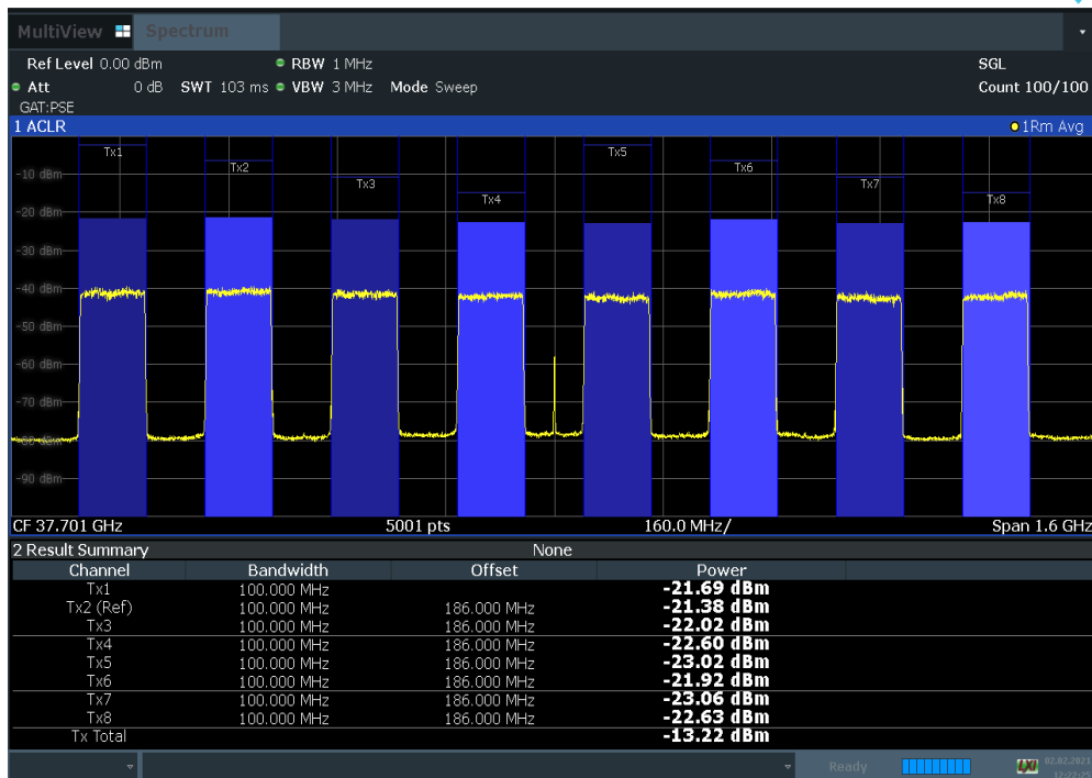
Plot 7-59. Antenna B EIRP Density Plot (100 MHz BW 8CC NC 16QAM Low Channel)
