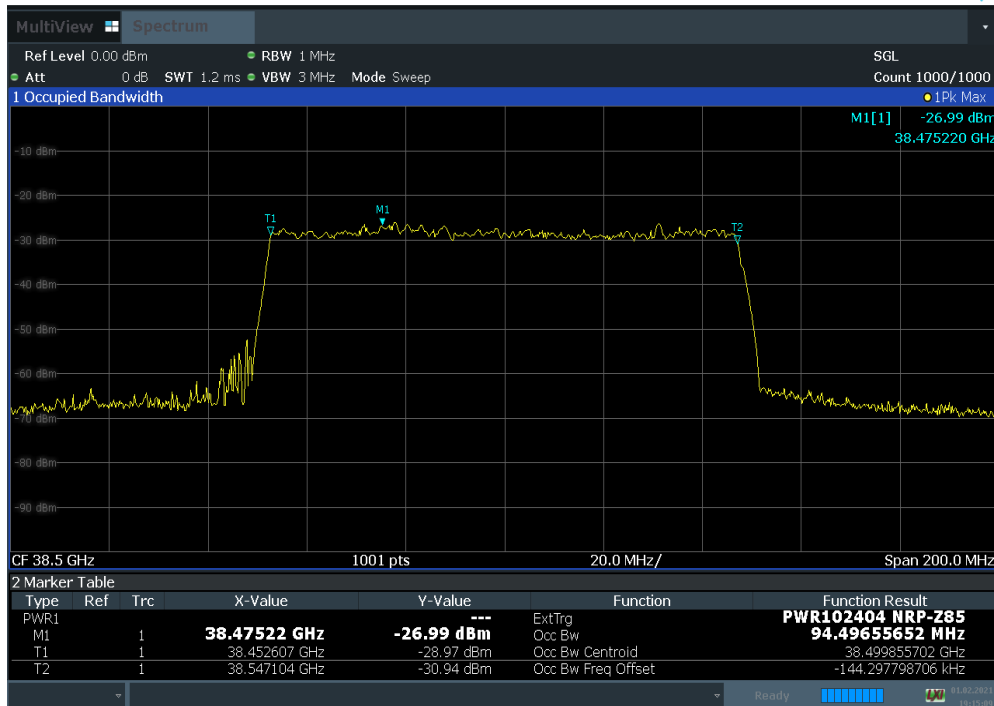
Plot 7-9. Occupied Bandwidth Plot (100 MHz 1CC BW 64QAM Mid Channel)
