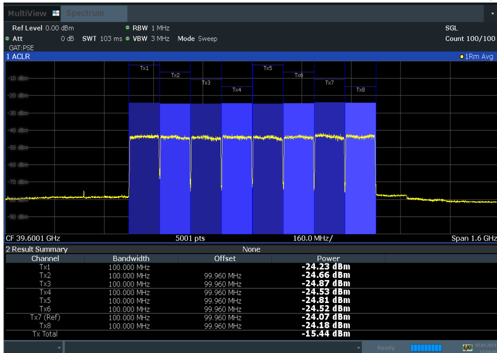
Plot 7-75. Antenna B EIRP Density Plot (100 MHz BW 8CC 64QAM High Channel)
