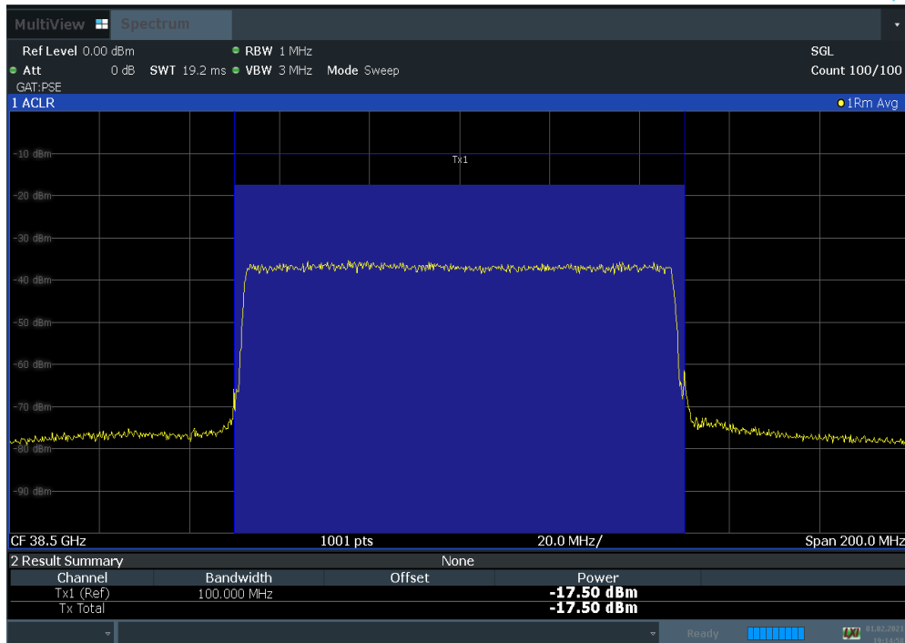
Plot 7-63. Antenna B EIRP Density Plot (100 MHz 1CC BW 64QAM Mid Channel)
