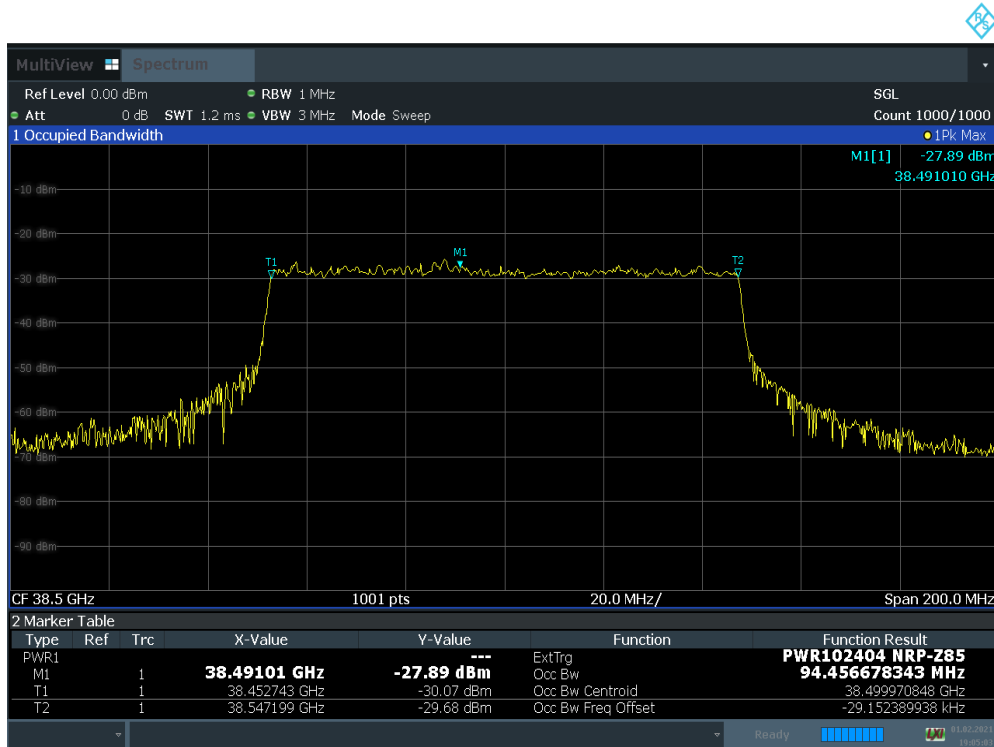
Plot 7-1. Occupied Bandwidth Plot (100 MHz BW 1CC QPSK Mid Channel)
