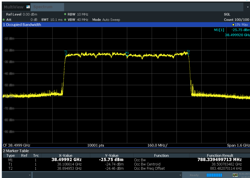
Plot 7-24. Occupied Bandwidth Plot (100 MHz BW 8CC 64QAM Mid Channel)
