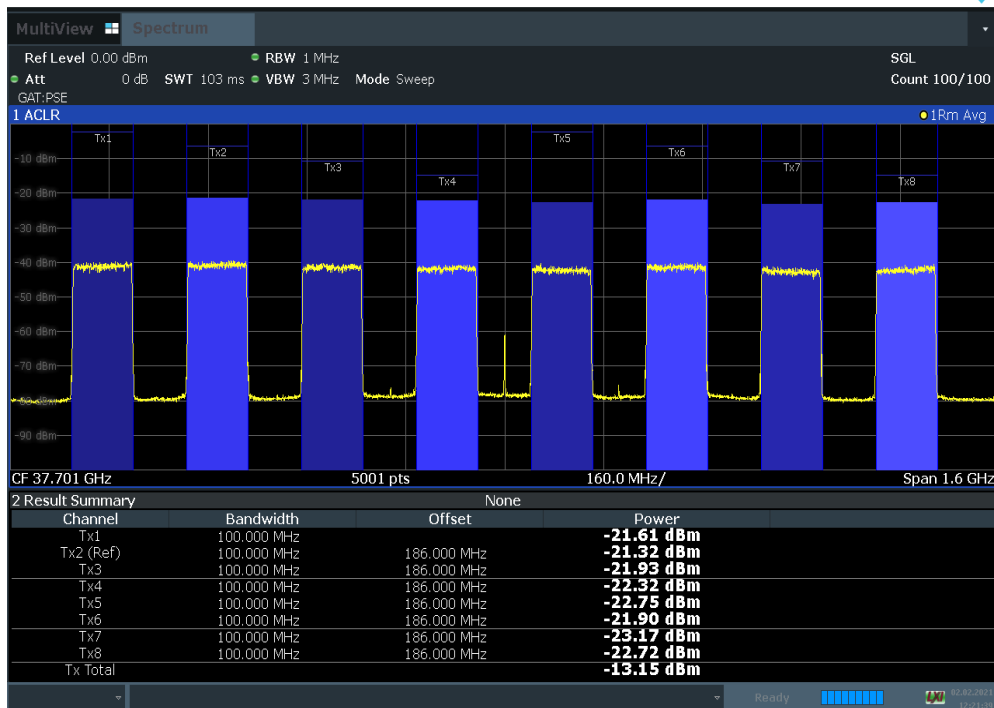
Plot 7-113. Antenna D EIRP Density Plot (100 MHz BW 8CC NC 16QAM Low Channel)
