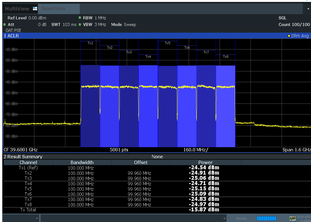
Plot 7-47. Antenna A EIRP Density Plot (100 MHz BW 8CC 16QAM High Channel)
