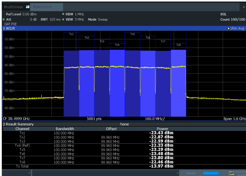
Plot 7-64. Antenna B EIRP Density Plot (100 MHz BW 8CC QPSK Mid Channel)
