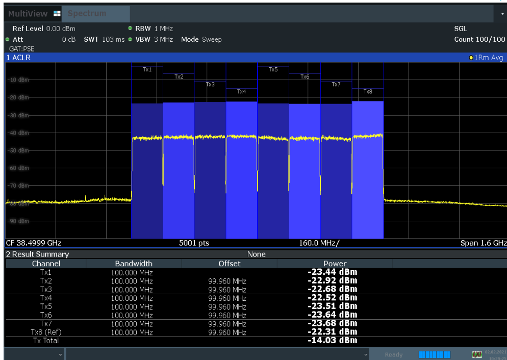
Plot 7-119. Antenna D EIRP Density Plot (100 MHz BW 8CC 16QAM Mid Channel)
