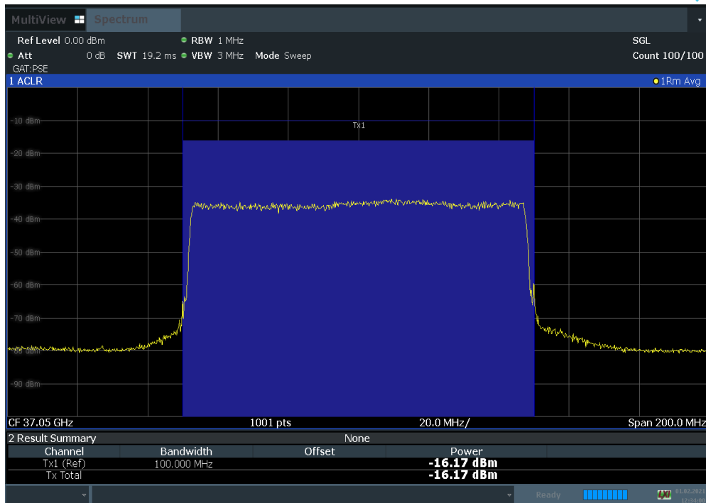
Plot 7-81. Antenna C EIRP Density Plot (100 MHz 1CC BW 64QAM Low Channel)
