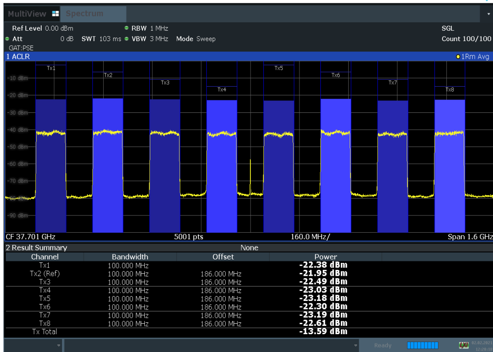
Plot 7-87. Antenna C EIRP Density Plot (100 MHz BW 8CC NC 64QAM Low Channel)
