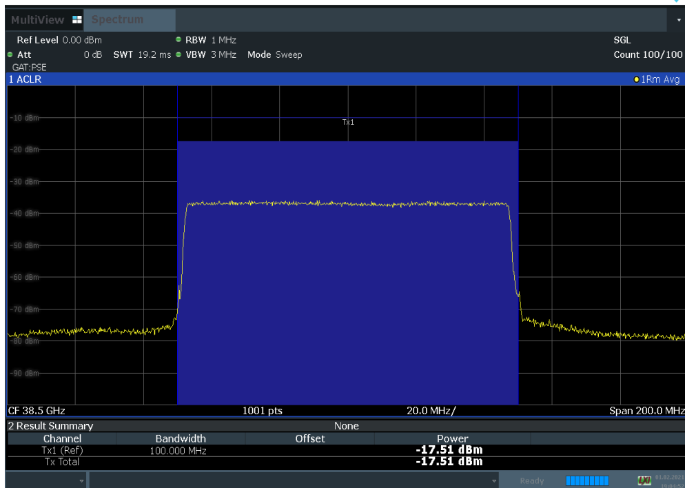
Plot 7-34. Antenna A EIRP Density Plot (100 MHz BW 1CC QPSK Mid Channel)
