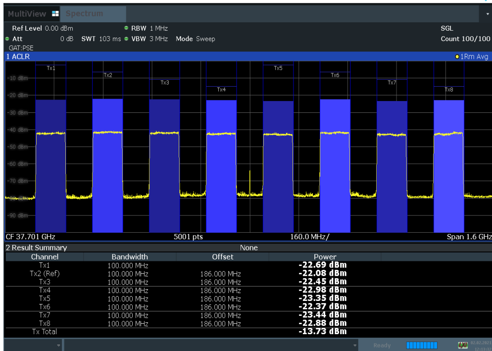
Plot 7-31. Antenna A EIRP Density Plot (100 MHz BW 8CC NC QPSK Low Channel)
