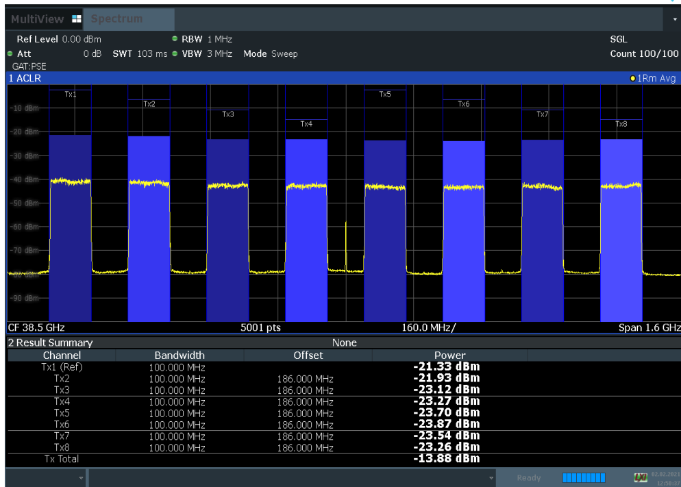
Plot 7-68. Antenna B EIRP Density Plot (100 MHz BW 8CC NC 16QAM Mid Channel)
