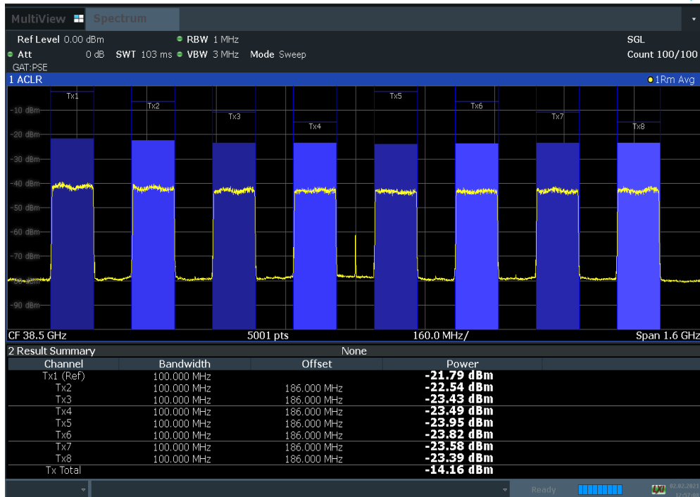
Plot 7-96. Antenna C EIRP Density Plot (100 MHz BW 8CC NC 64QAM Mid Channel)
