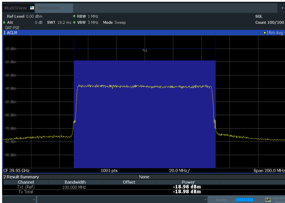
Plot 7-45. Antenna A EIRP Density Plot (100 MHz 1CC BW 64QAM High Channel)
