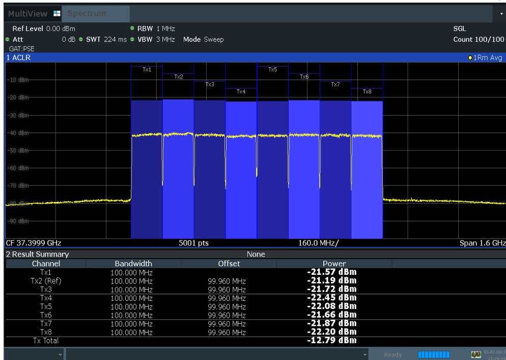
Plot 7-111. Antenna D EIRP Density Plot (100 MHz BW 8CC 64QAM Low Channel)
