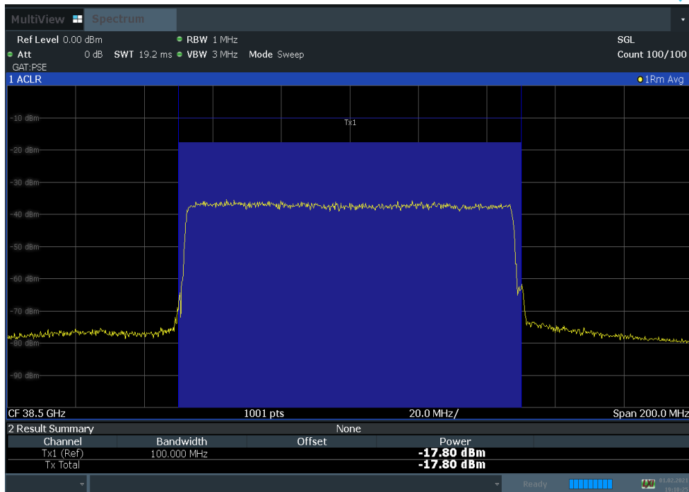
Plot 7-89. Antenna C EIRP Density Plot (100 MHz 1CC BW 16QAM Mid Channel)
