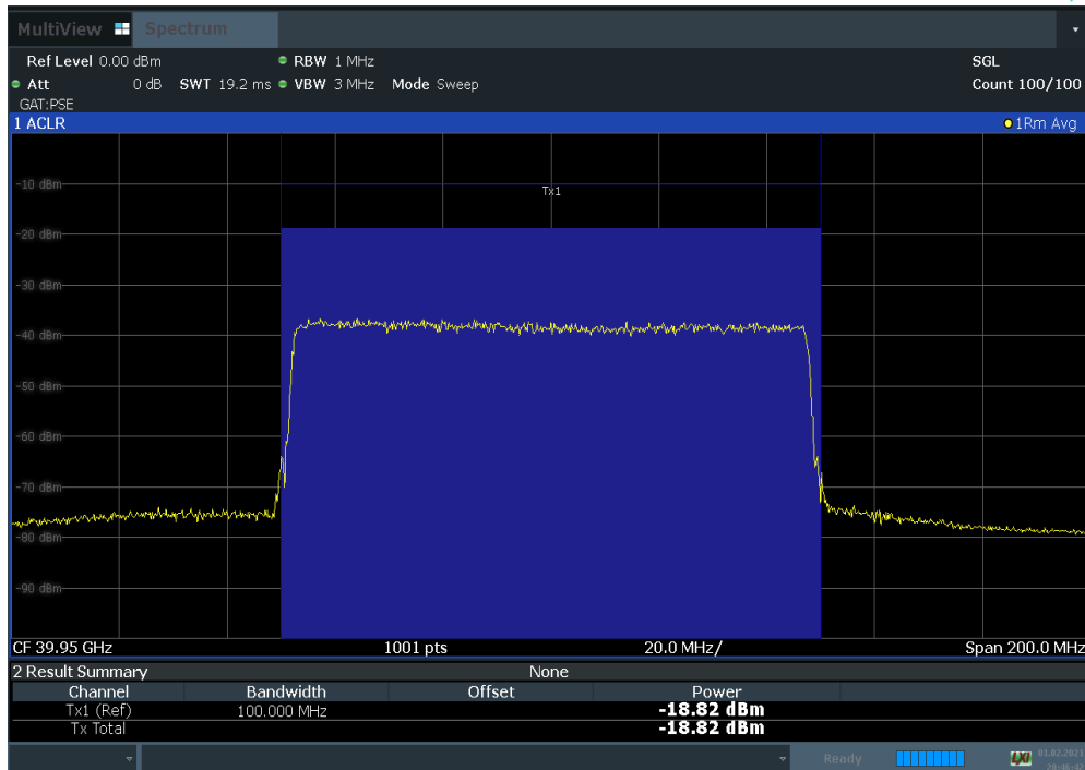
Plot 7-71. Antenna B EIRP Density Plot (100 MHz BW 1CC 16QAM High Channel)
