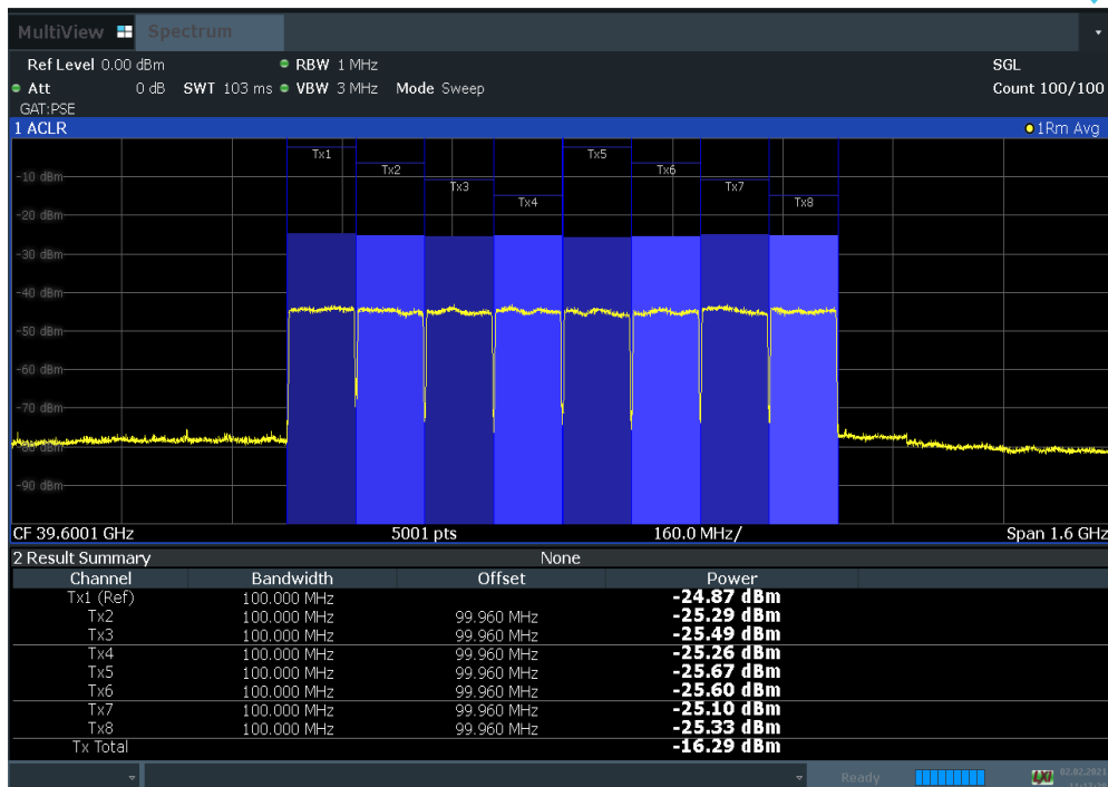
Plot 7-100. Antenna C EIRP Density Plot (100 MHz BW 8CC QPSK High Channel)
