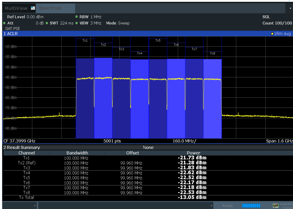
Plot 7-29. Antenna A EIRP Density Plot (100 MHz BW 8CC 16QAM Low Channel)
