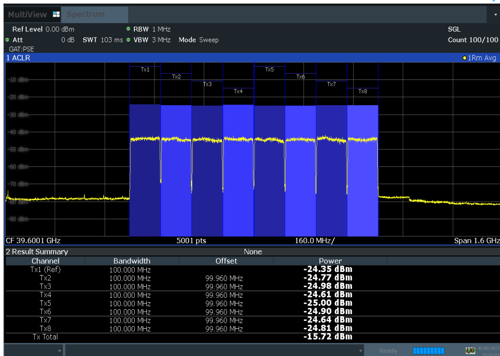
Plot 7-46. Antenna A EIRP Density Plot (100 MHz BW 8CC QPSK High Channel)
