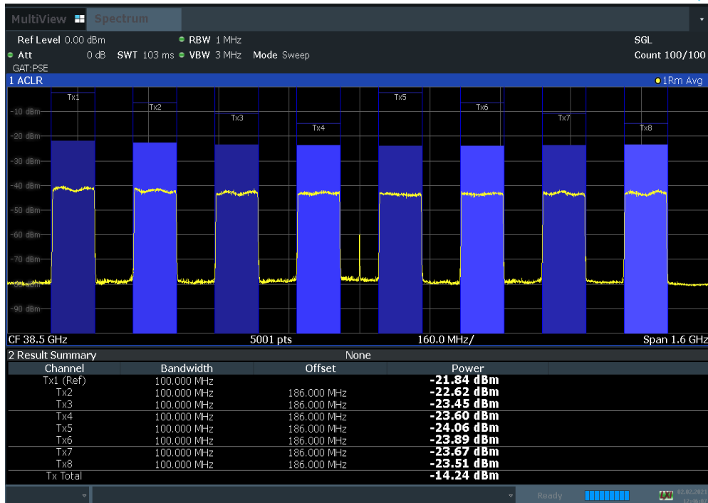
Plot 7-94. Antenna C EIRP Density Plot (100 MHz BW 8CC NC QPSK Mid Channel)
