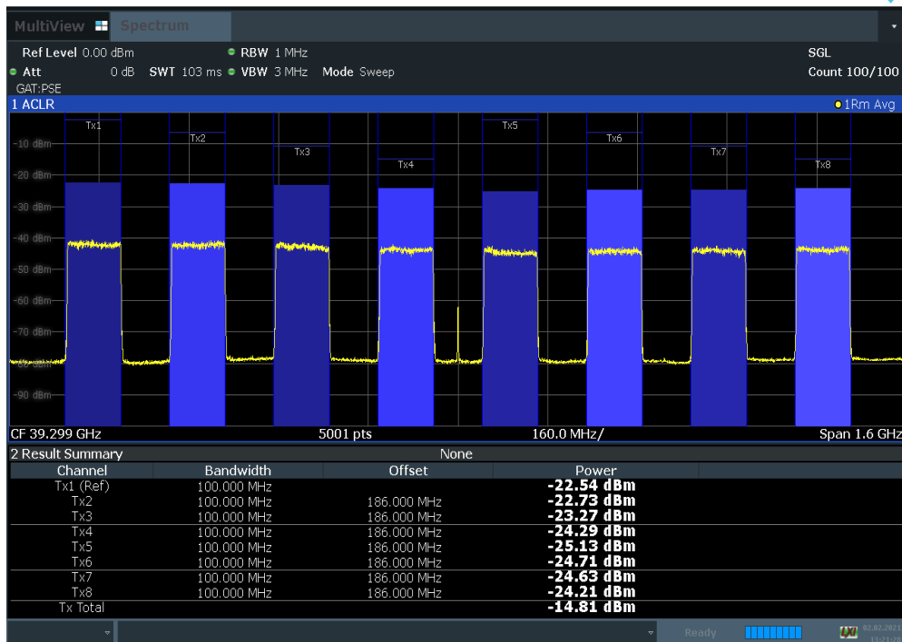
Plot 7-77. Antenna B EIRP Density Plot (100 MHz BW 8CC NC 16QAM High Channel)
