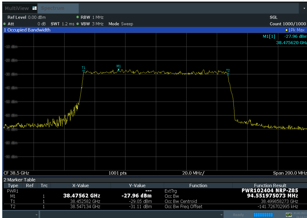
Plot 7-21. Occupied Bandwidth Plot (100 MHz 1CC BW 64QAM Mid Channel)
