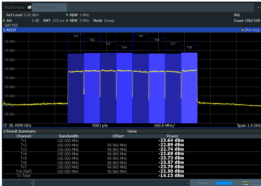
Plot 7-37. Antenna A EIRP Density Plot (100 MHz BW 8CC QPSK Mid Channel)
