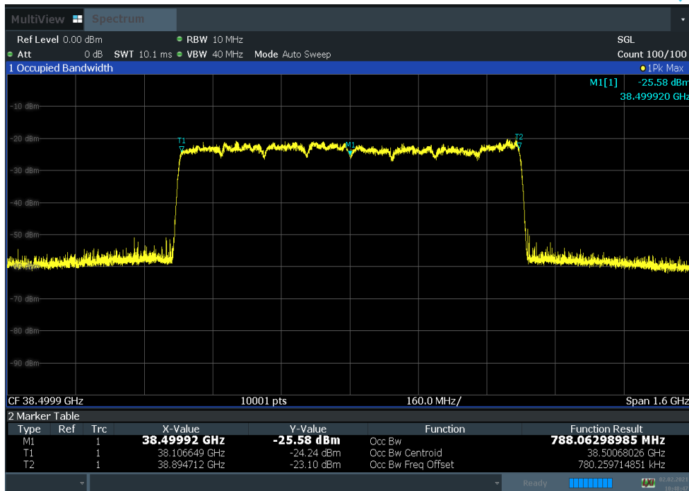
Plot 7-12. Occupied Bandwidth Plot (100 MHz BW 8CC 64QAM Mid Channel)
