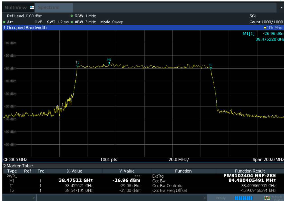
Plot 7-3. Occupied Bandwidth Plot (100 MHz 1CC BW 64QAM Mid Channel)
