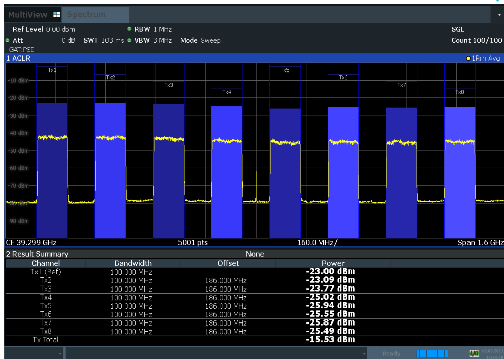
Plot 7-104. Antenna C EIRP Density Plot (100 MHz BW 8CC NC 16QAM High Channel)
