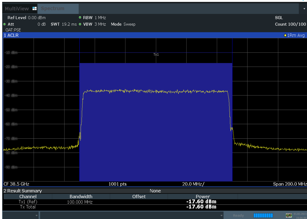
Plot 7-35. Antenna A EIRP Density Plot (100 MHz 1CC BW 16QAM Mid Channel)
