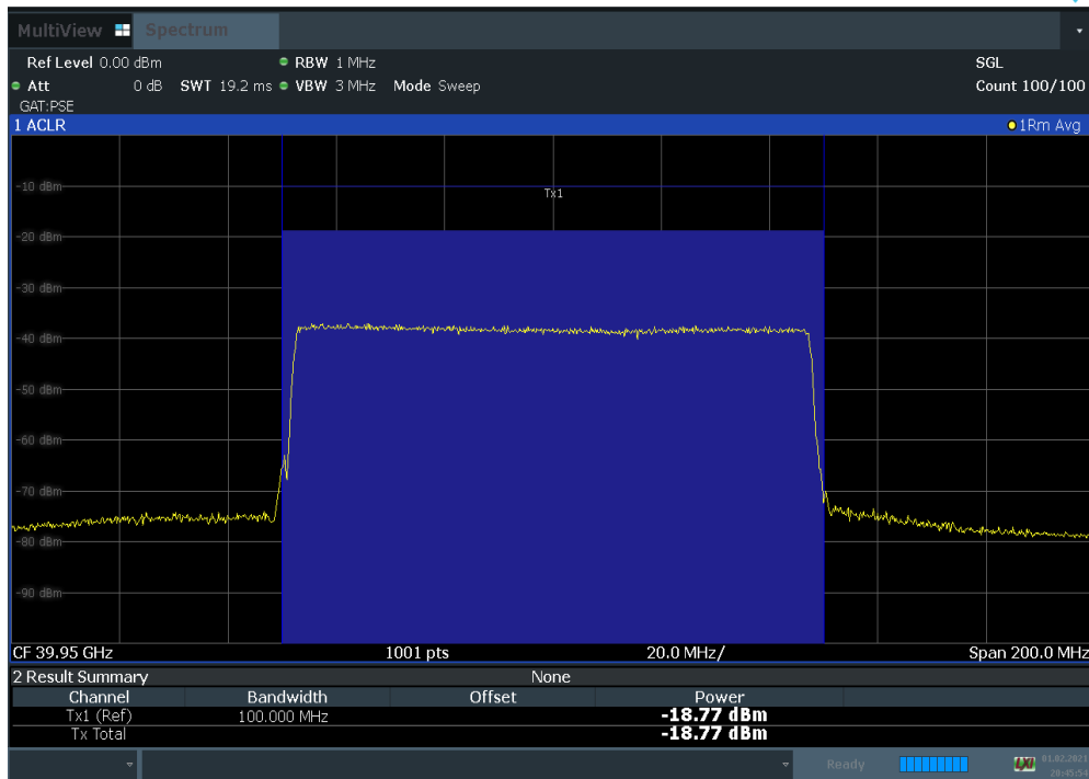
Plot 7-70. Antenna B EIRP Density Plot (100 MHz BW 1CC QPSK High Channel)
