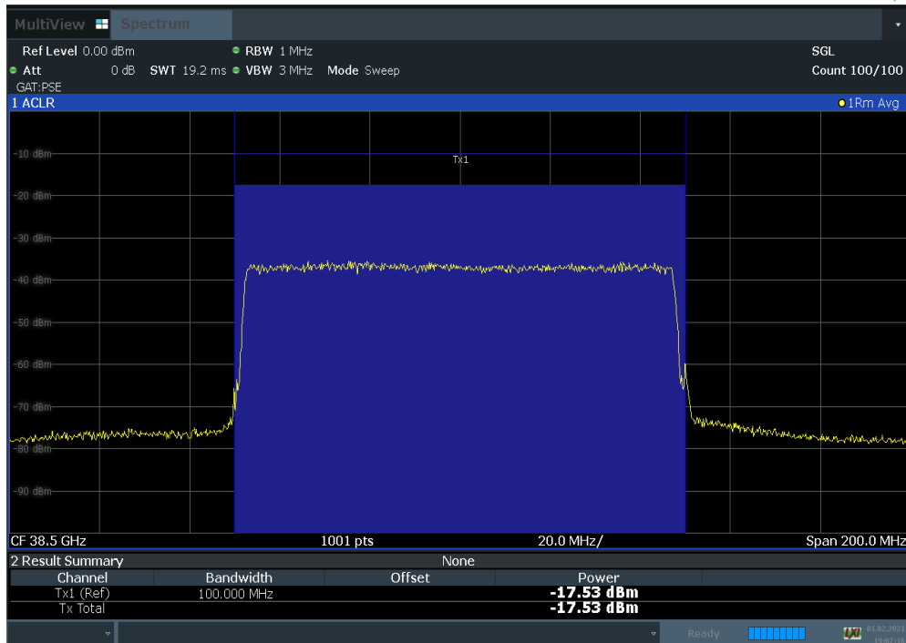
Plot 7-36. Antenna A EIRP Density Plot (100 MHz 1CC BW 64QAM Mid Channel)
