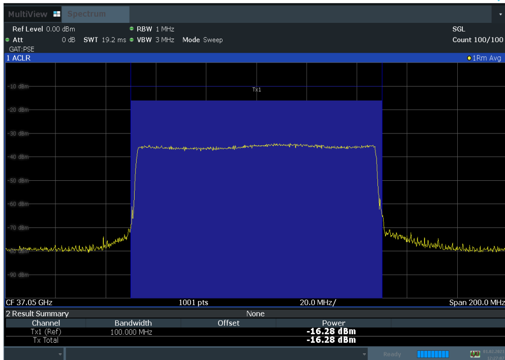
Plot 7-79. Antenna C EIRP Density Plot (100 MHz BW 1CC QPSK Low Channel)
