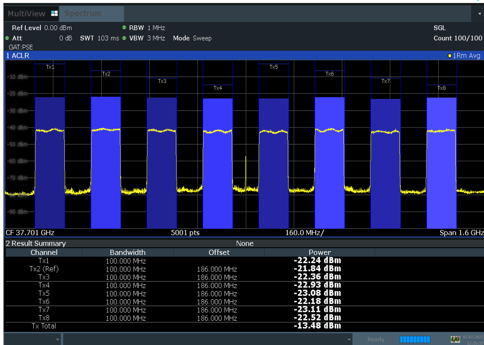
Plot 7-85. Antenna C EIRP Density Plot (100 MHz BW 8CC NC QPSK Low Channel)
