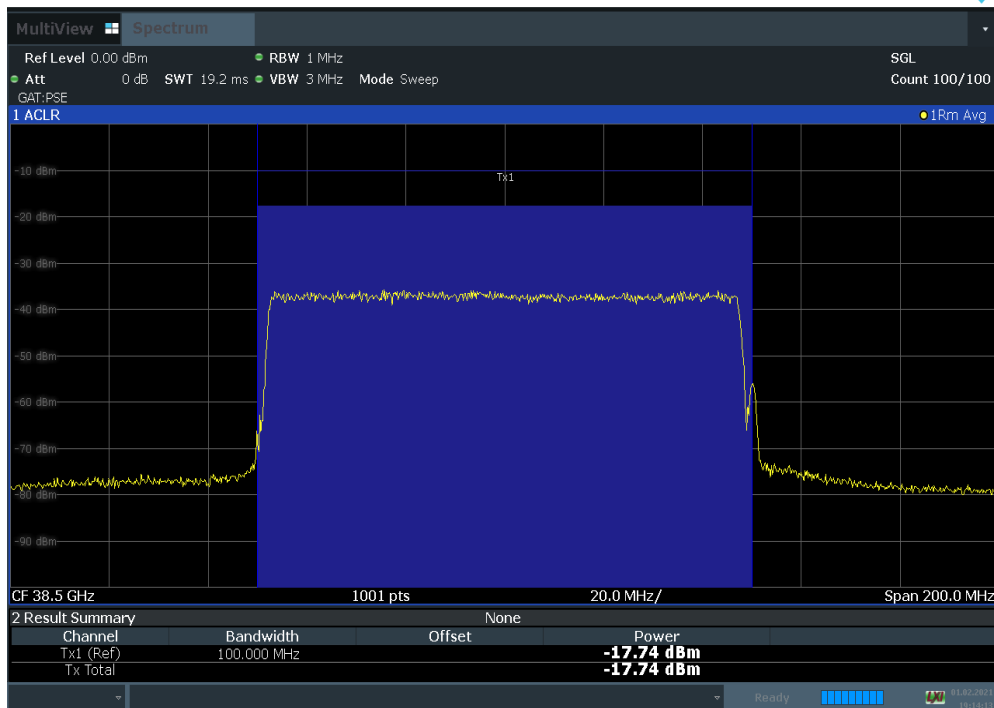
Plot 7-117. Antenna D EIRP Density Plot (100 MHz 1CC BW 64QAM Mid Channel)
