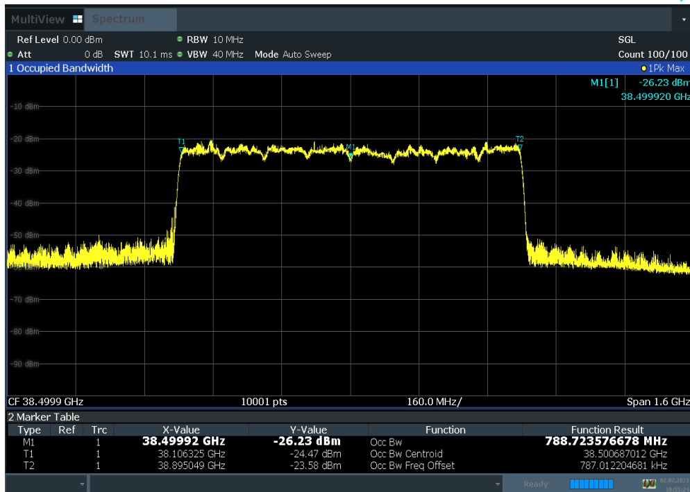
Plot 7-22. Occupied Bandwidth Plot (100 MHz BW 8CC QPSK Mid Channel)
