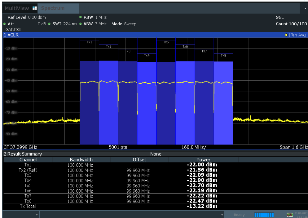
Plot 7-82. Antenna C EIRP Density Plot (100 MHz BW 8CC QPSK Low Channel)
