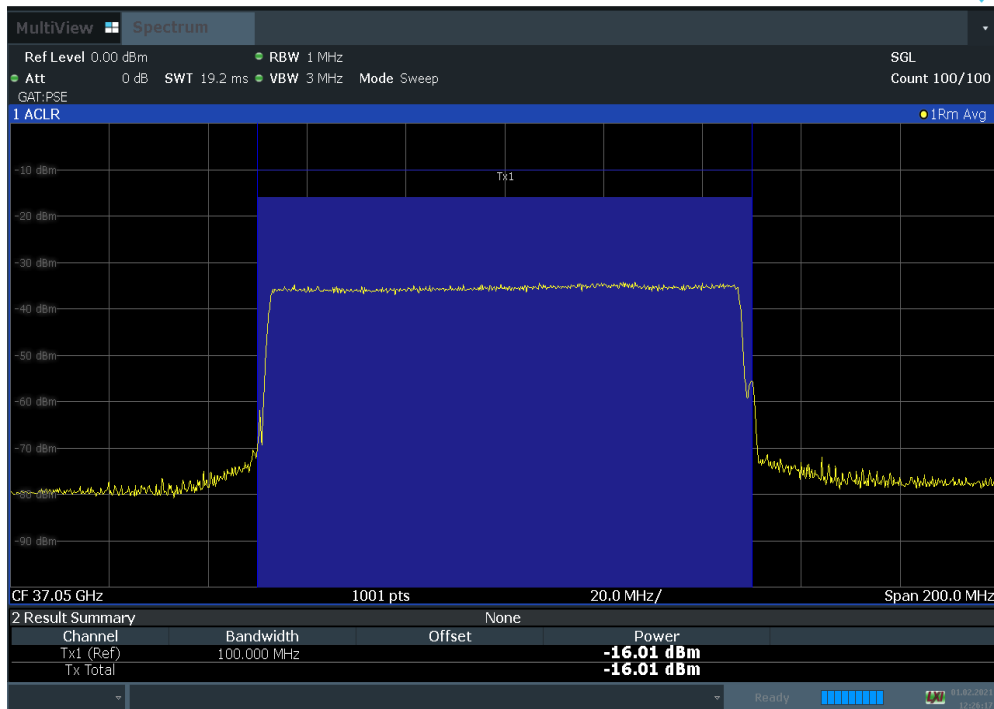
Plot 7-25. Antenna A EIRP Density Plot (100 MHz BW 1CC QPSK Low Channel)
