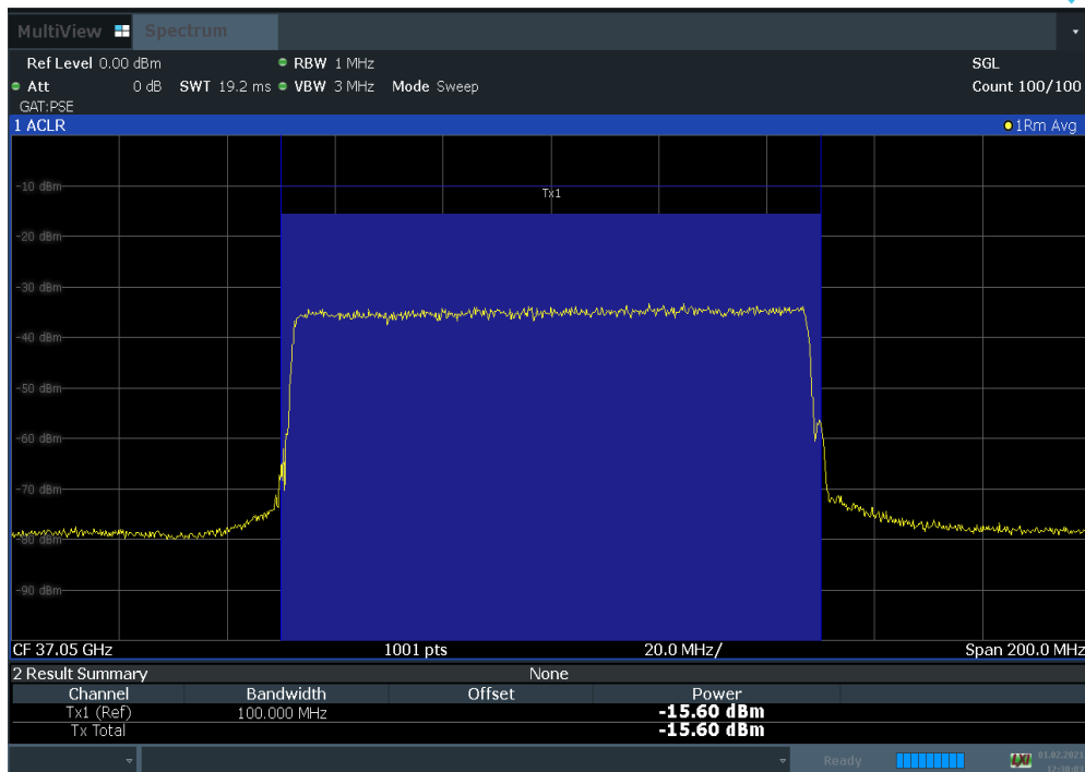
Plot 7-107. Antenna D EIRP Density Plot (100 MHz 1CC BW 16QAM Low Channel)
