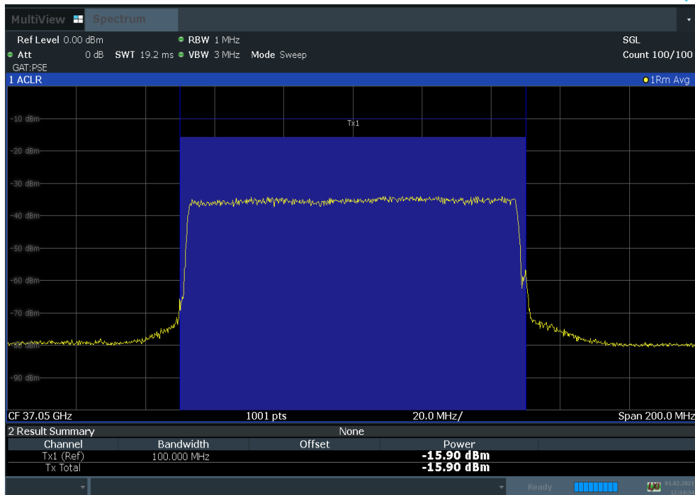
Plot 7-54. Antenna B EIRP Density Plot (100 MHz 1CC BW 64QAM Low Channel)
