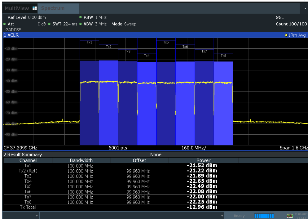
Plot 7-57. Antenna B EIRP Density Plot (100 MHz BW 8CC 64QAM Low Channel)
