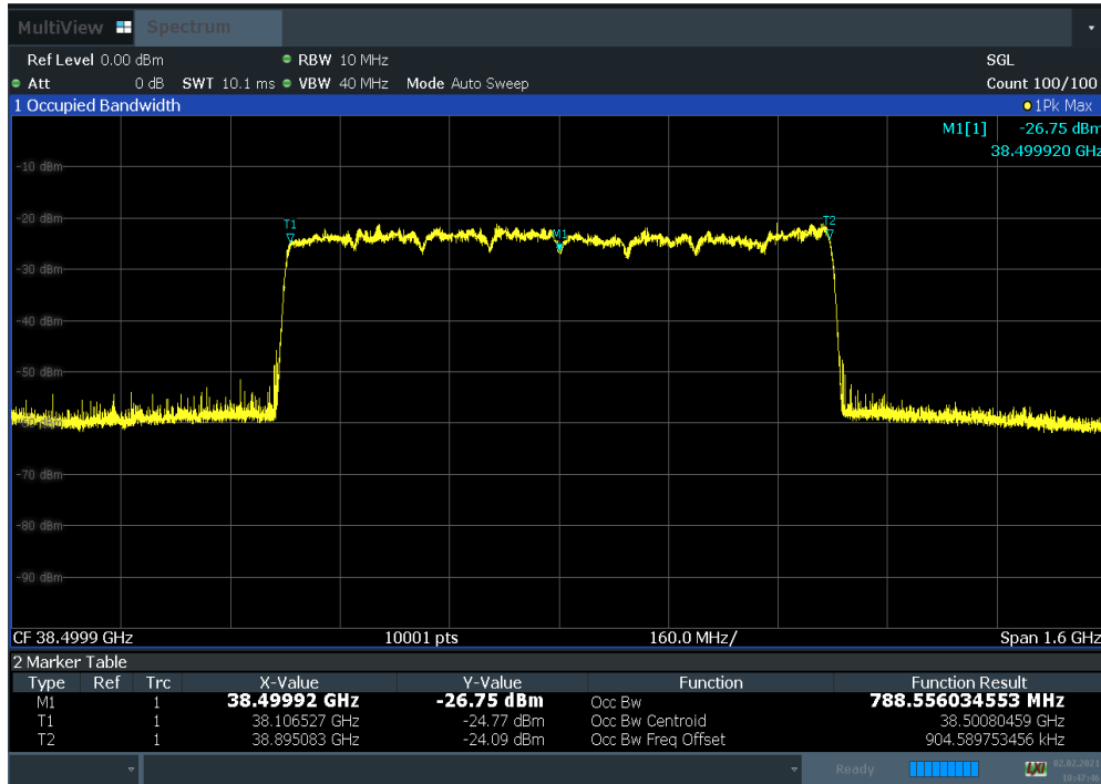
Plot 7-6. Occupied Bandwidth Plot (100 MHz BW 8CC 64QAM Mid Channel)
