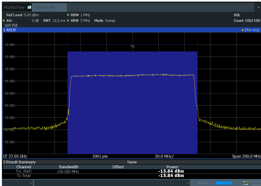
Plot 7-52. Antenna B EIRP Density Plot (100 MHz BW 1CC QPSK Low Channel)
