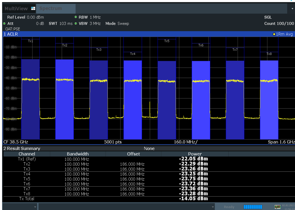
Plot 7-42. Antenna A EIRP Density Plot (100 MHz BW 8CC NC 64QAM Mid Channel)
