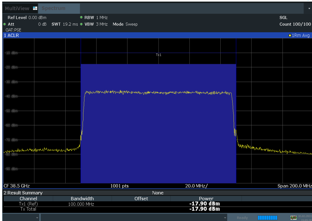
Plot 7-90. Antenna C EIRP Density Plot (100 MHz 1CC BW 64QAM Mid Channel)
