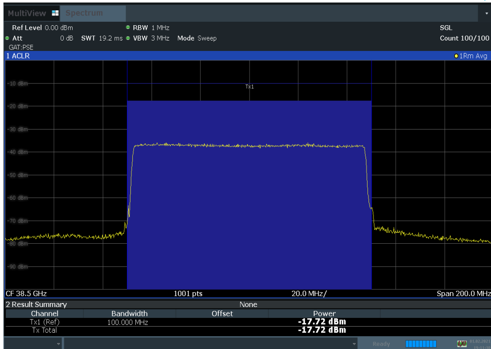
Plot 7-88. Antenna C EIRP Density Plot (100 MHz BW 1CC QPSK Mid Channel)
