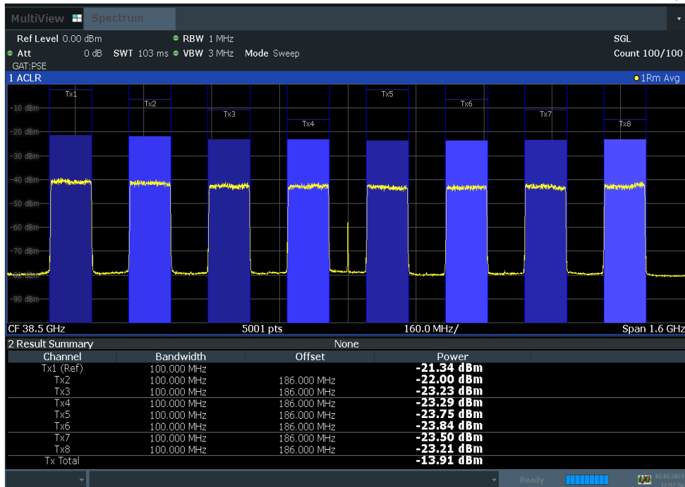
Plot 7-69. Antenna B EIRP Density Plot (100 MHz BW 8CC NC 64QAM Mid Channel)
