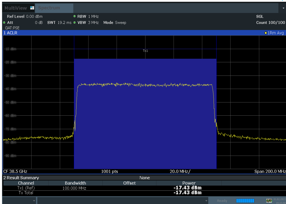
Plot 7-62. Antenna B EIRP Density Plot (100 MHz 1CC BW 16QAM Mid Channel)
