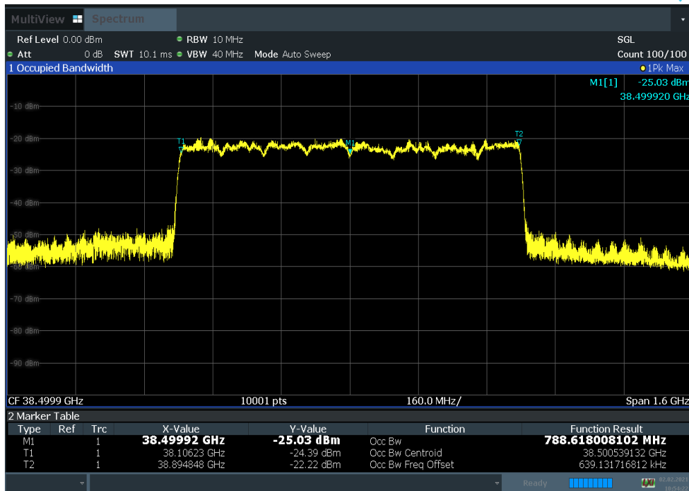
Plot 7-10. Occupied Bandwidth Plot (100 MHz BW 8CC QPSK Mid Channel)
