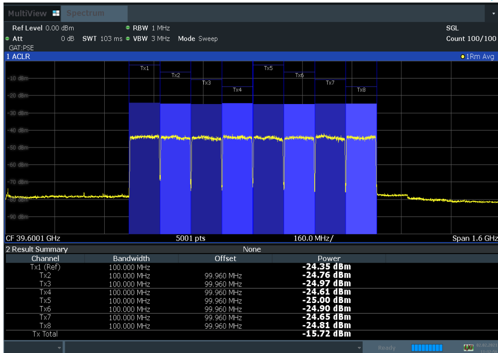
Plot 7-48. Antenna A EIRP Density Plot (100 MHz BW 8CC 64QAM High Channel)
