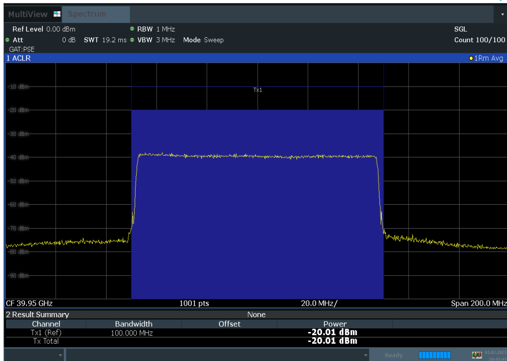
Plot 7-97. Antenna C EIRP Density Plot (100 MHz BW 1CC QPSK High Channel)
