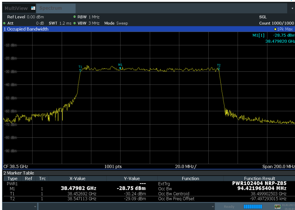
Plot 7-8. Occupied Bandwidth Plot (100 MHz 1CC BW 16QAM Mid Channel)
