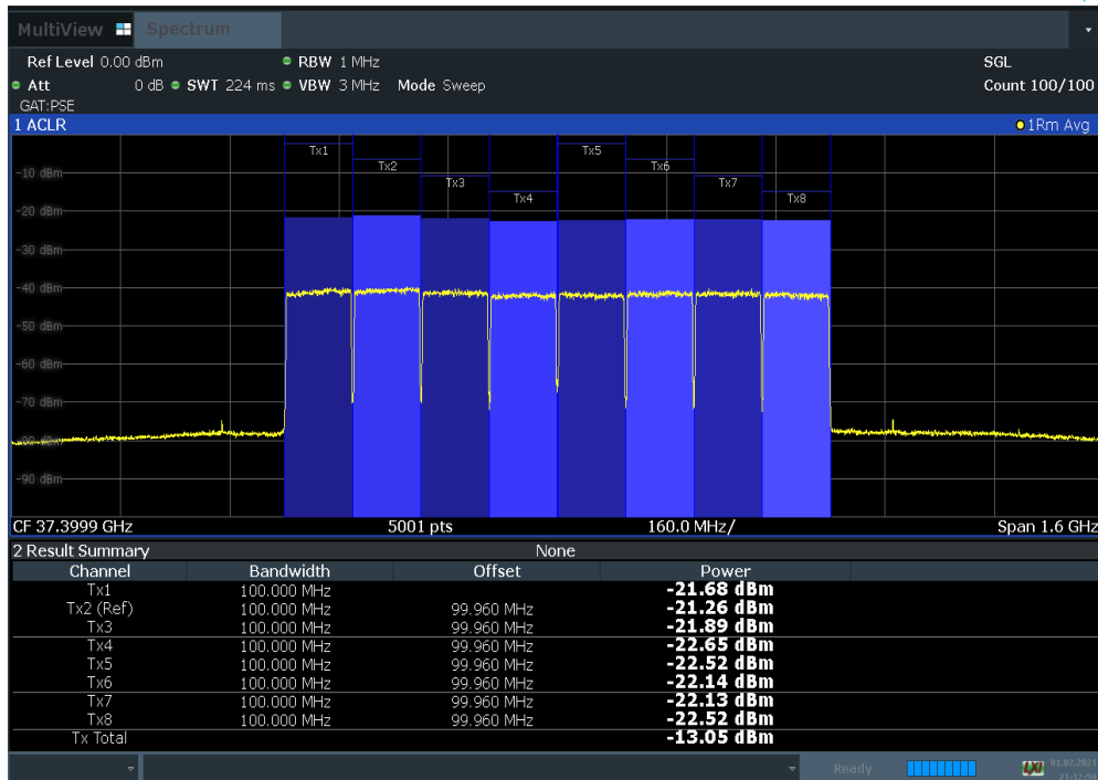
Plot 7-30. Antenna A EIRP Density Plot (100 MHz BW 8CC 64QAM Low Channel)
