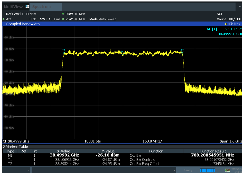
Plot 7-16. Occupied Bandwidth Plot (100 MHz BW 8CC QPSK Mid Channel)
