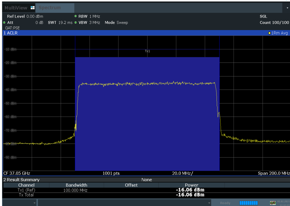
Plot 7-26. Antenna A EIRP Density Plot (100 MHz 1CC BW 16QAM Low Channel)
