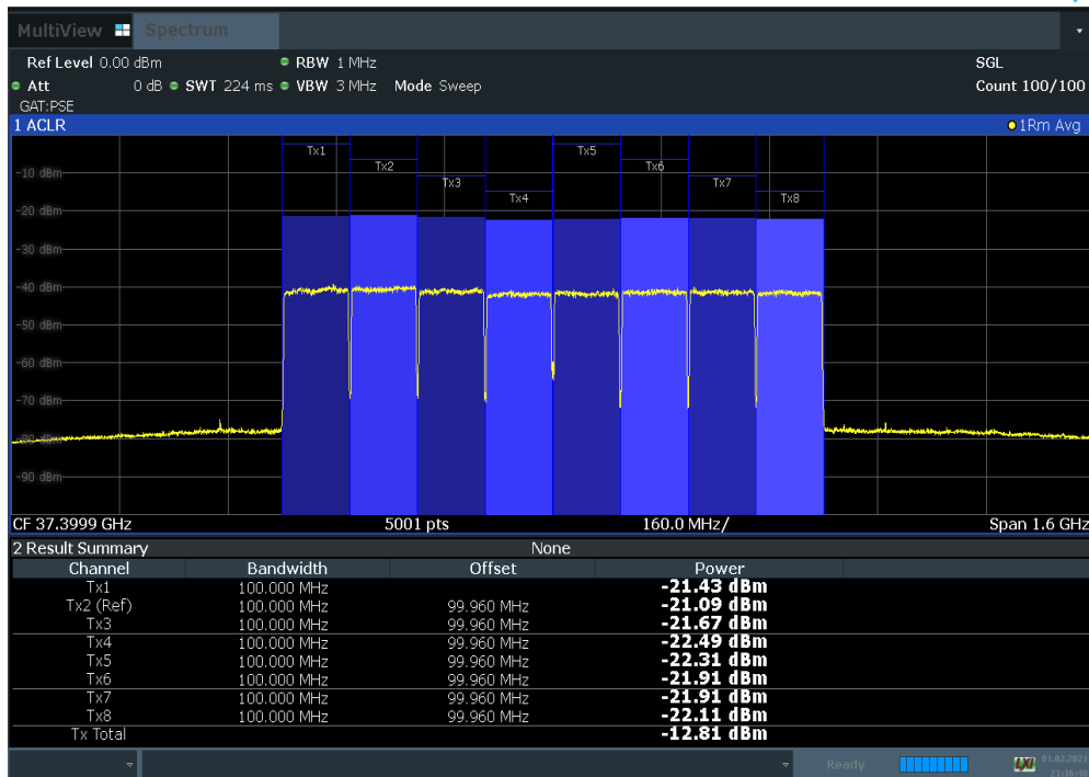
Plot 7-56. Antenna B EIRP Density Plot (100 MHz BW 8CC 16QAM Low Channel)
