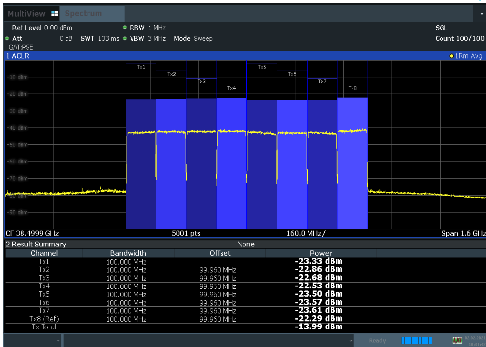
Plot 7-118. Antenna D EIRP Density Plot (100 MHz BW 8CC QPSK Mid Channel)
