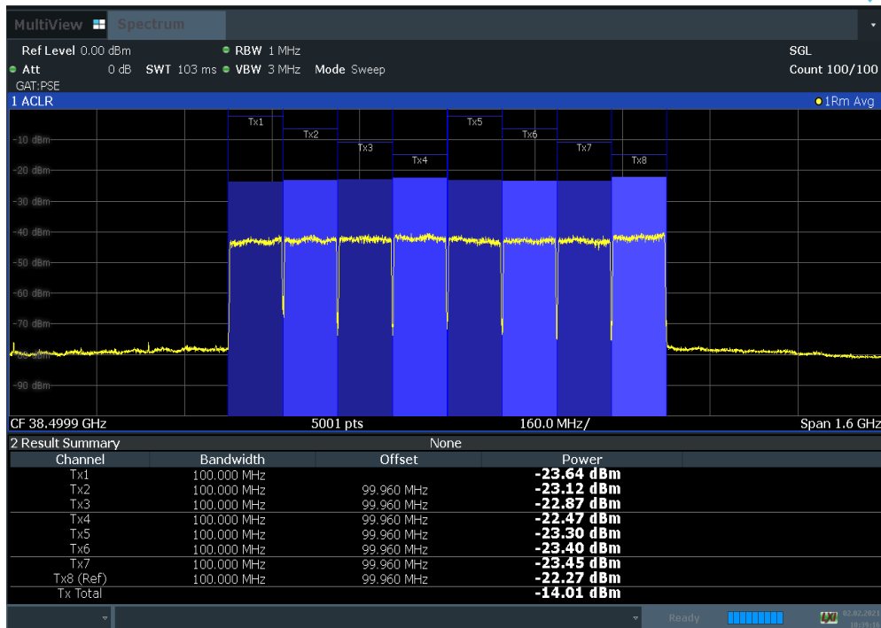
Plot 7-93. Antenna C EIRP Density Plot (100 MHz BW 8CC 64QAM Mid Channel)
