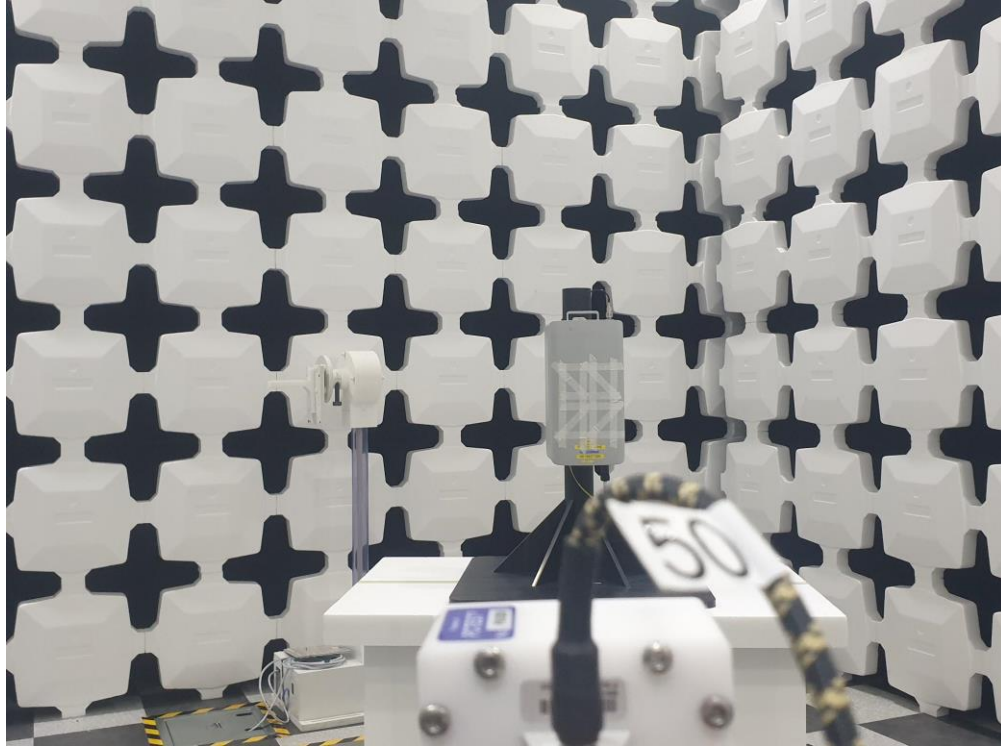
RSE 18 GHz – 40 GHz
