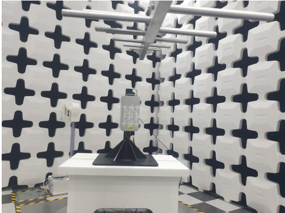
RSE 30 MHz – 1000 MHz
