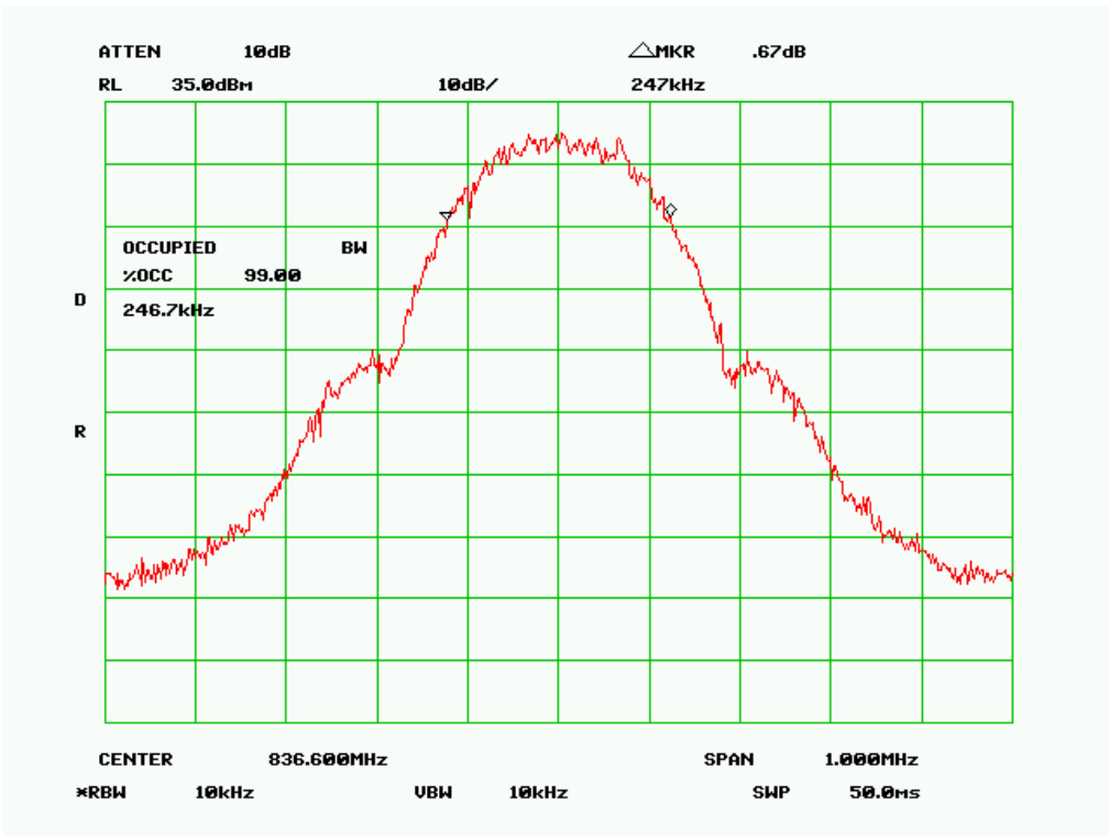
99% Occupied Bandwidth – GSM850, Channel 190, Mid Channel
