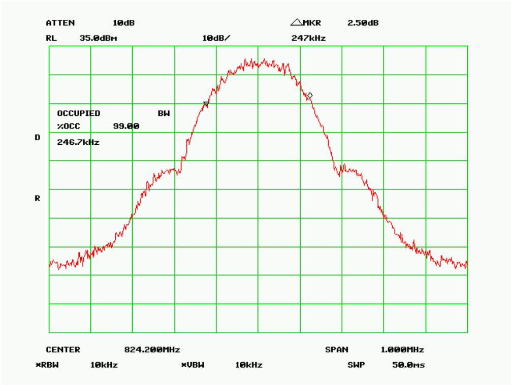
99% Occupied Bandwidth – EGPRS850, Channel 128, Low Channel
