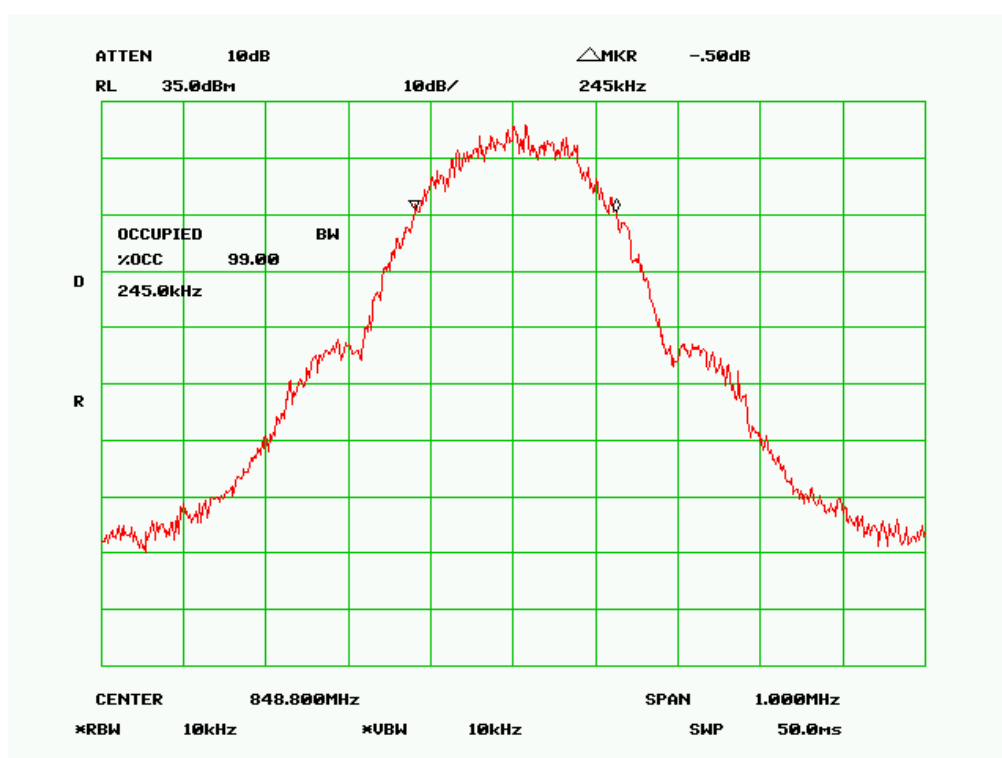
99% Occupied Bandwidth –EGPRS850, Channel 251, High Channel
