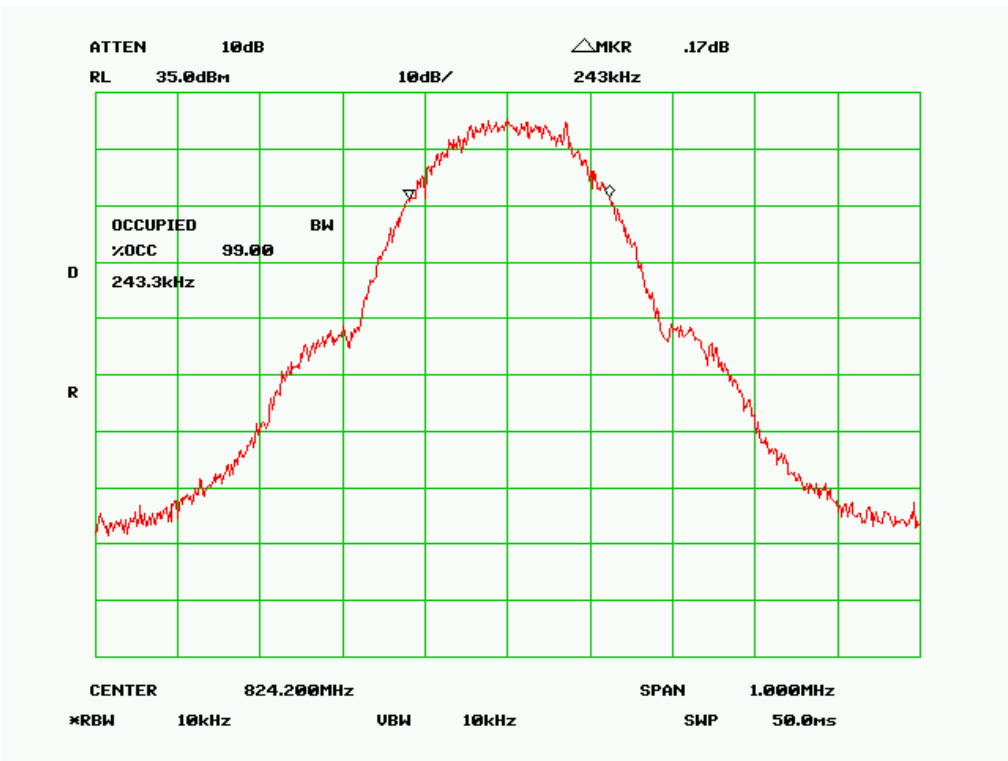
99% Occupied Bandwidth – GSM850, Channel 128, Low Channel
