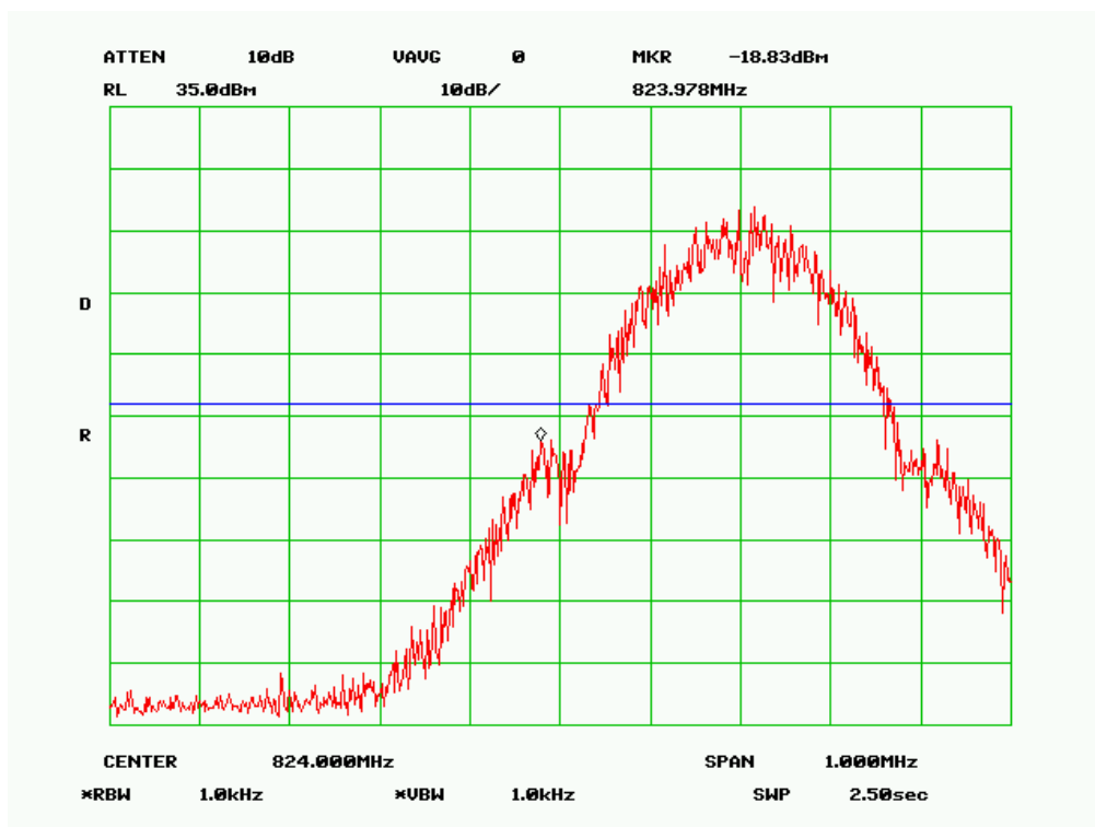
Lower Band Edge Plot – EGPRS850, Channel 128, Low Channel
