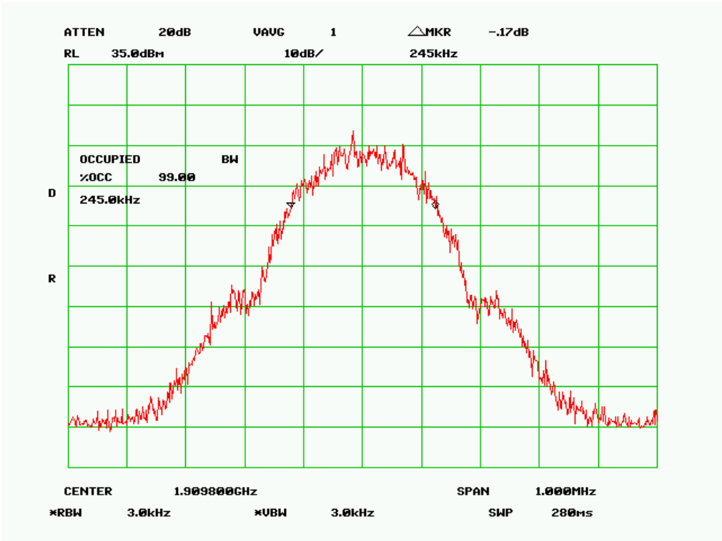
99% Occupied Bandwidth –EGPRS1900, Channel 810, High Channel
