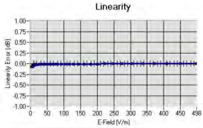
Linearity: \pm 1.61\% ( \pm 0.07\text{dB} )
