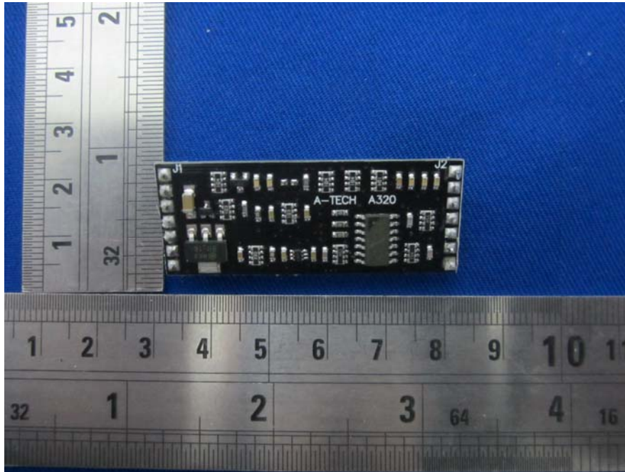
EUT – SLIC Board Top View
