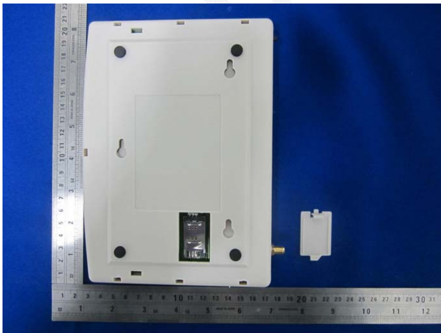
EUT – Sim Card Slot View
