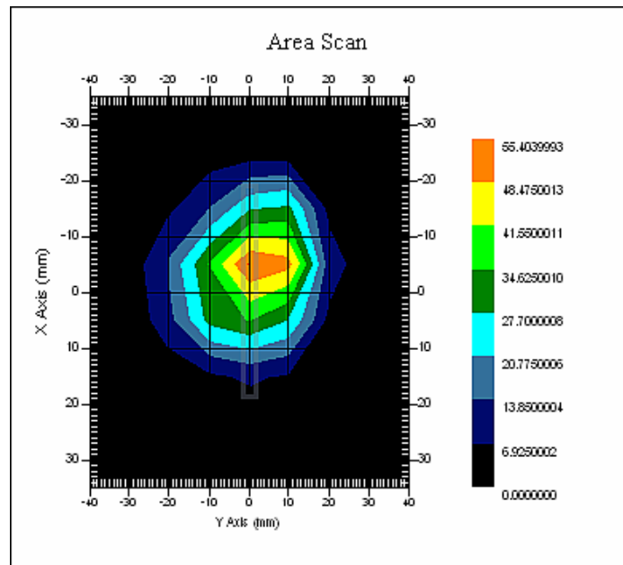
2450 MHz System Validation with Head Tissue
