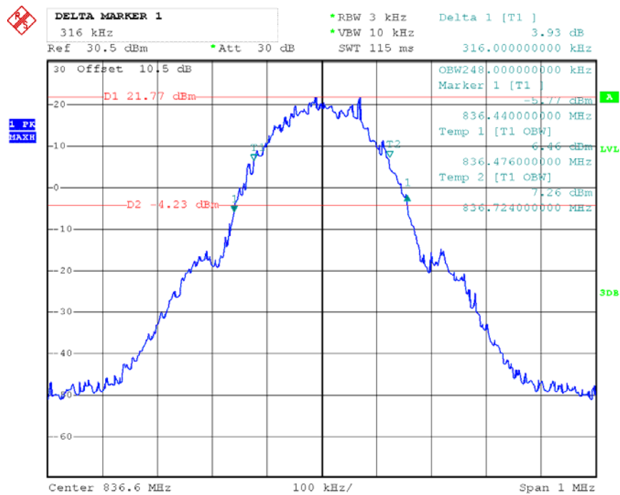
Cellular Band (Part 22H)
