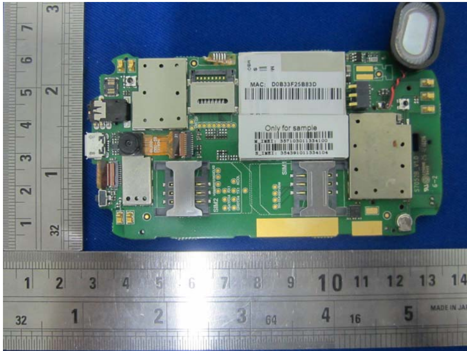
EUT – Main Board Bottom unshielding View
