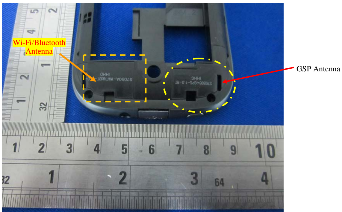
EUT – Wi-Fi/Bluetooth & GPS Antenna View
