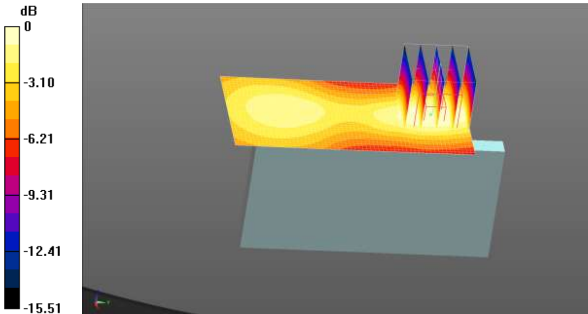
0 dB = 0.154 W/kg = -8.12 dBW/kg
