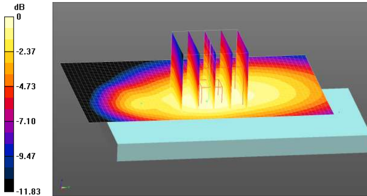
0 dB = 0.797 W/kg = -0.99 dBW/kg
