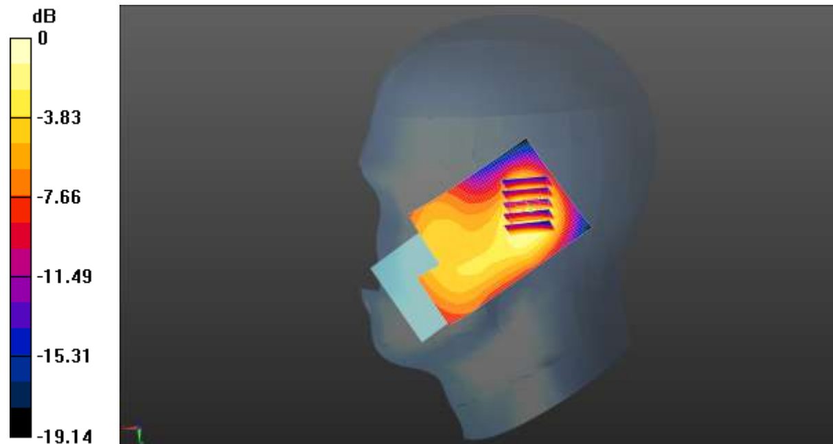
0 dB = 0.145 W/kg = -8.39 dBW/kg
