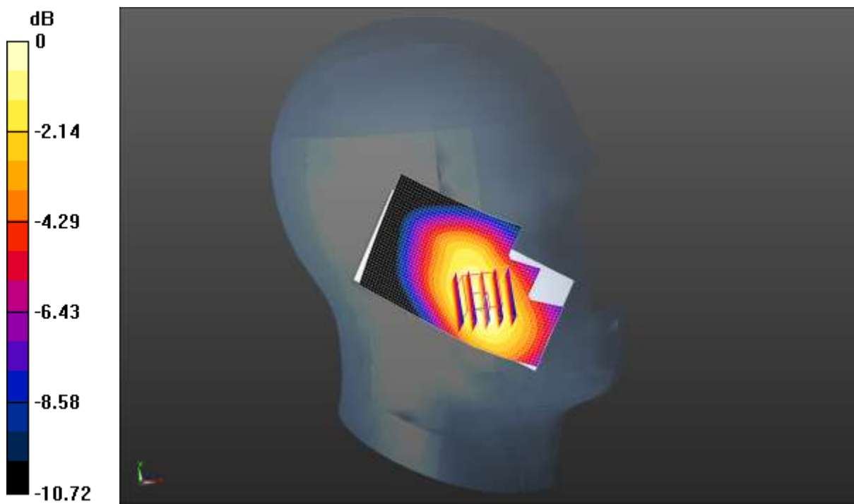
0 dB = 0.595 W/kg = -2.25 dBW/kg
