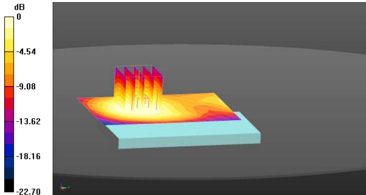
0 dB = 0.665 W/kg = -1.77 dBW/kg
