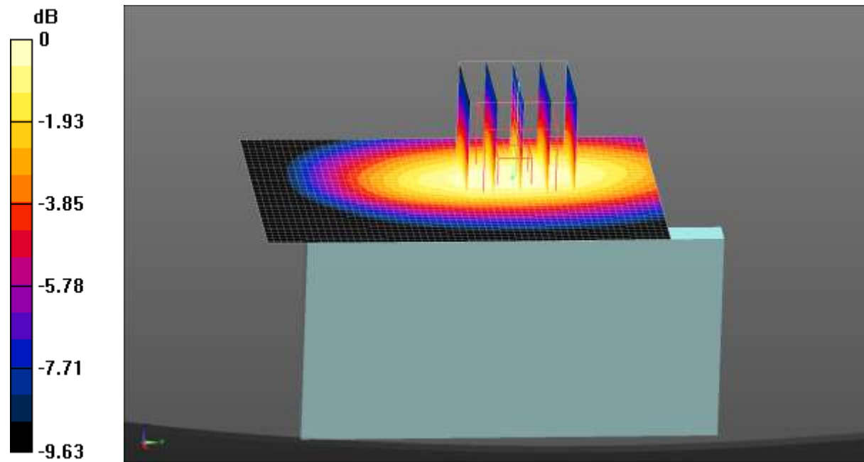
0 dB = 0.495 W/kg = -3.05 dBW/kg
