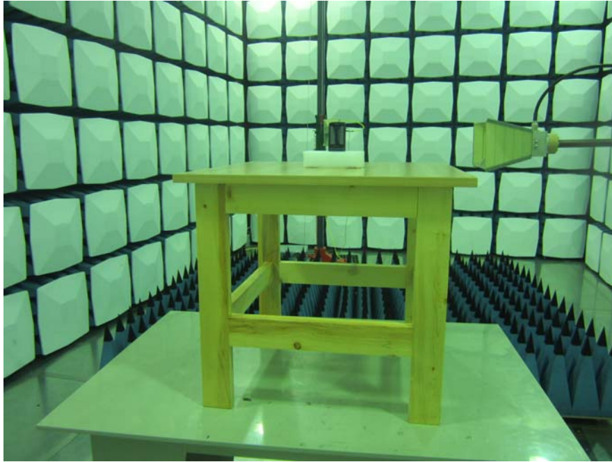
Radiated Emission View
