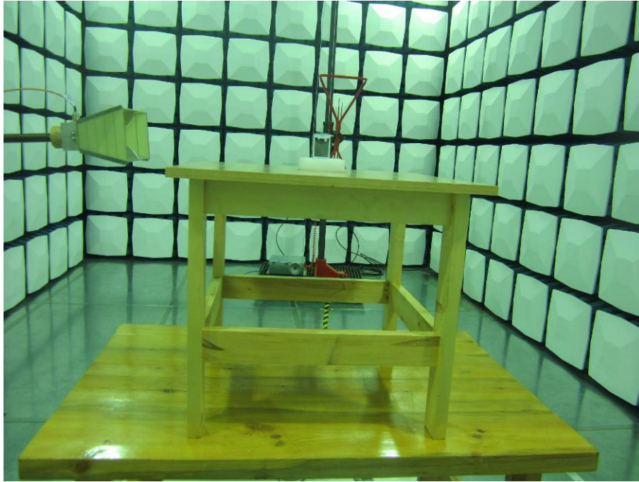
Radiated Emissions View 1
