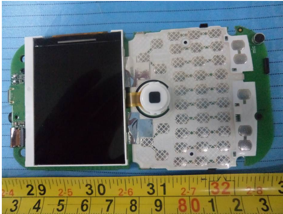
EUT – Main Board Bottom LCD & Keypad off View
