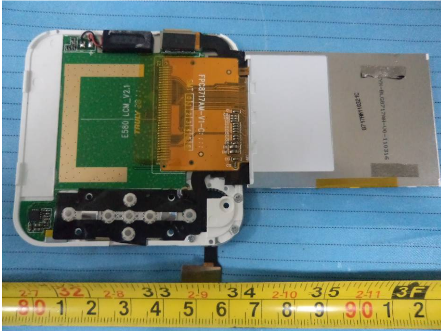
EUT – Display Cover off View 3
