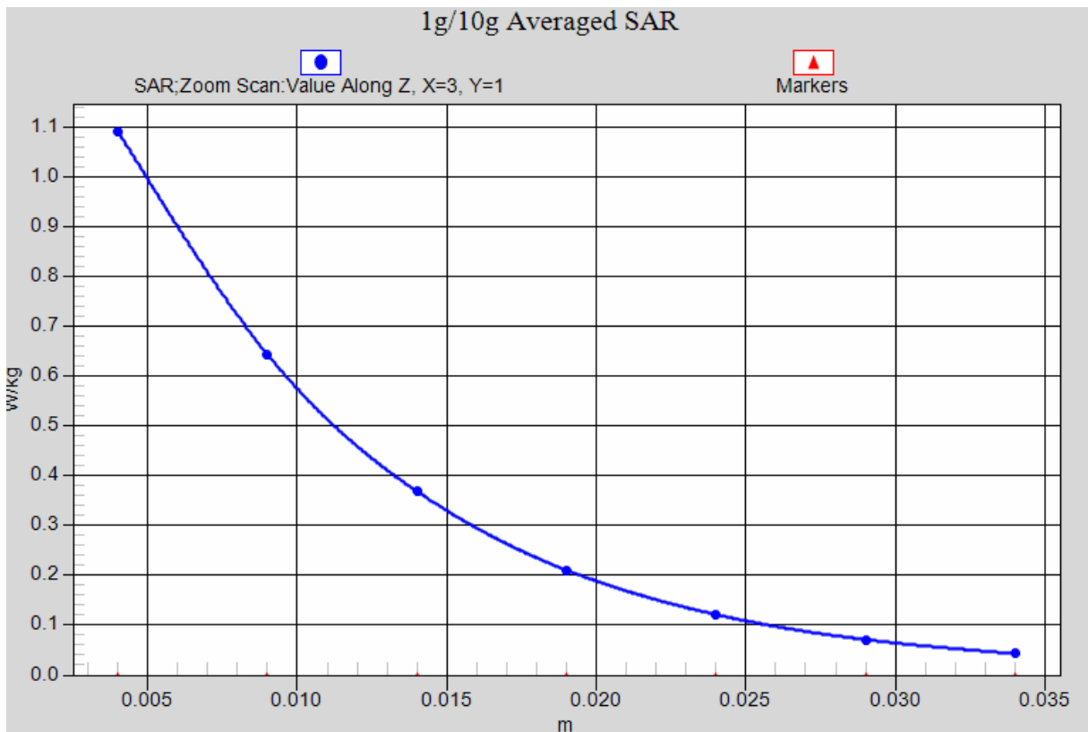
WCDMA Band II LEFT/CHEEK-Low_ z-axis scan
