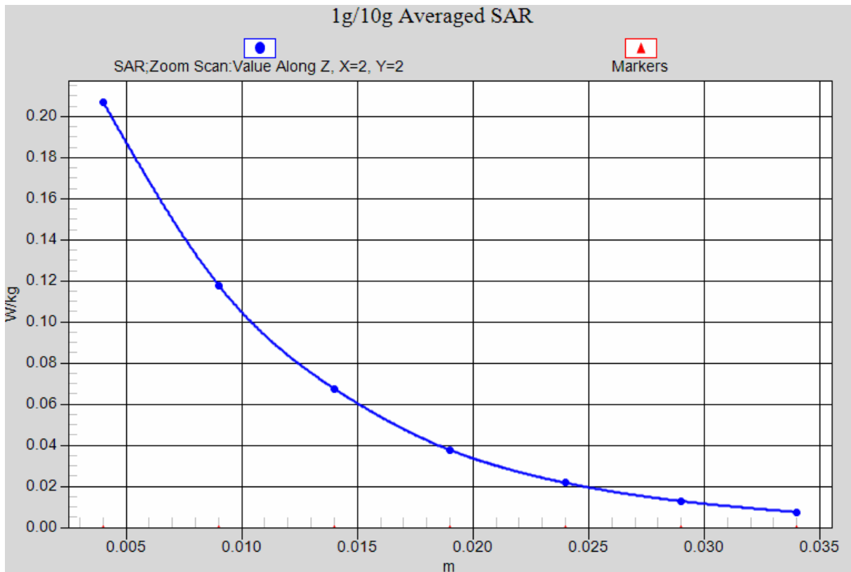
WiFi 802.11b RIGHT/CHEEK-Low_ z-axis scan
