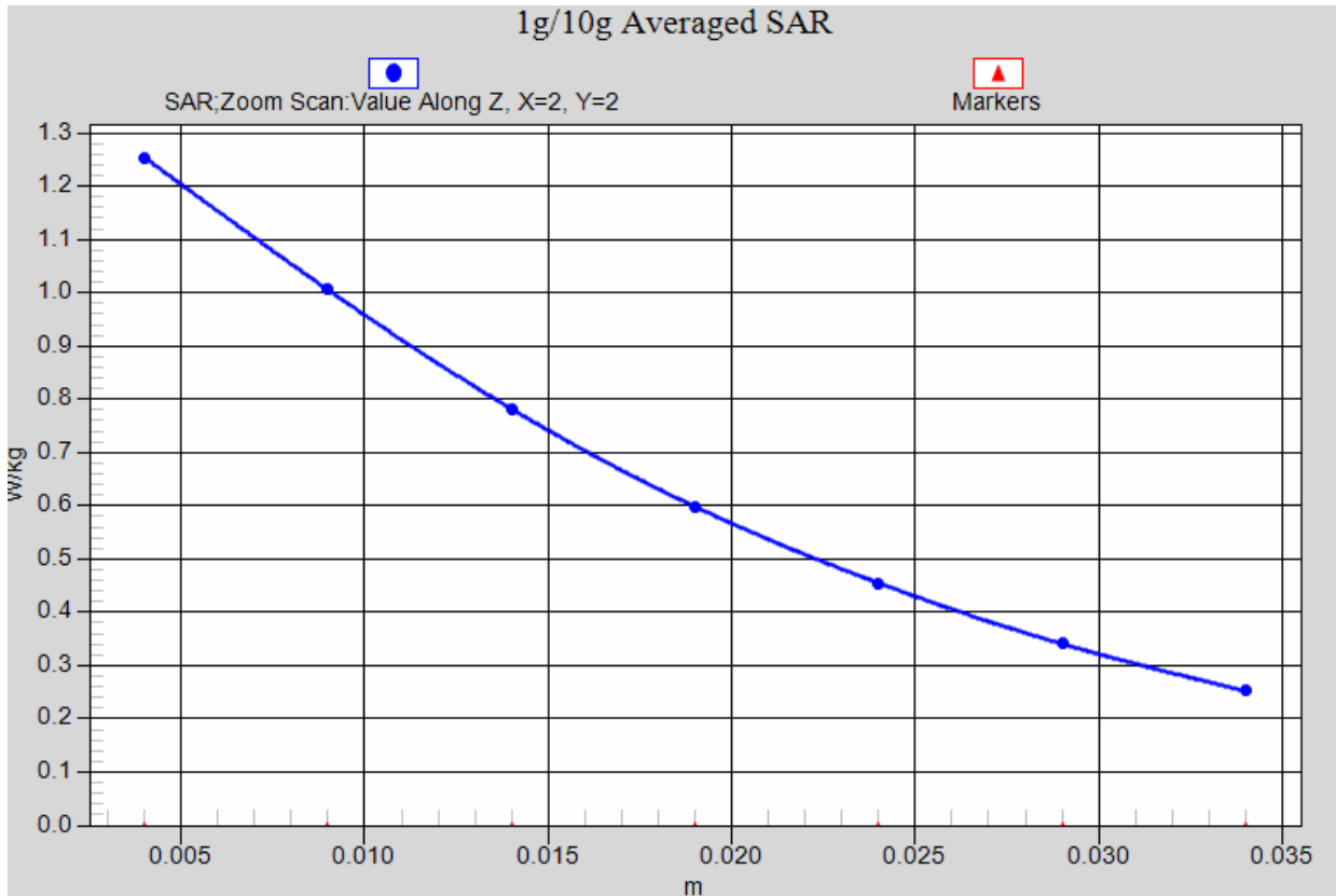
WCDMA Band V- LEFT/CHEEK-Low_ z-axis scan
