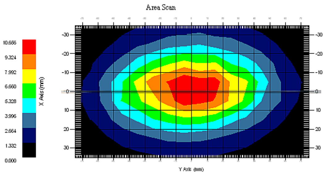
835 MHz System Validation with Body Tissue
