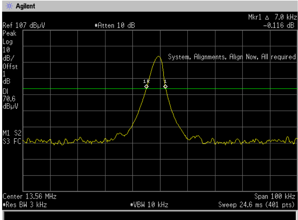
13.56HZ bandwidth test plot
