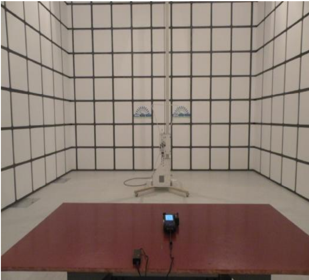
Radiated Emission Test Setup in Chamber
