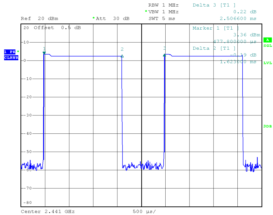
39 Channel @ 3DH3
