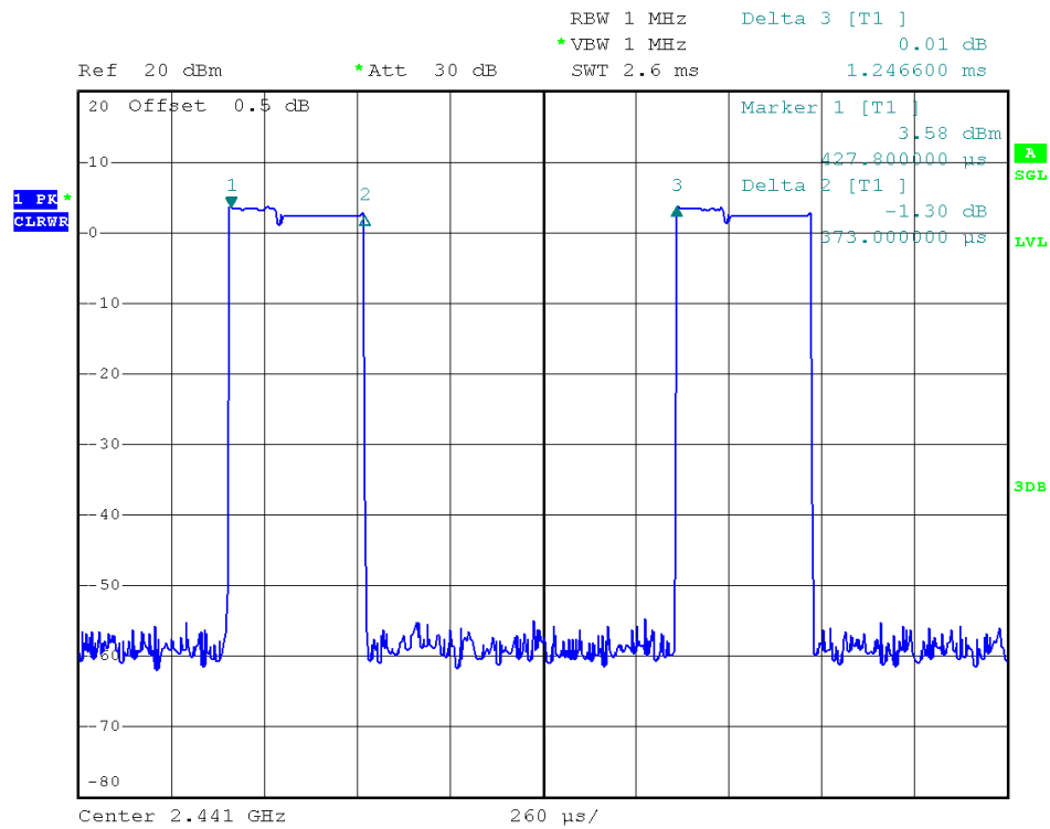
39 Channel @ 3DH1
