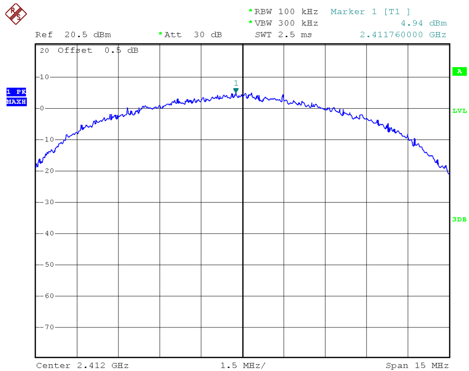
802.11b - Channel 1
