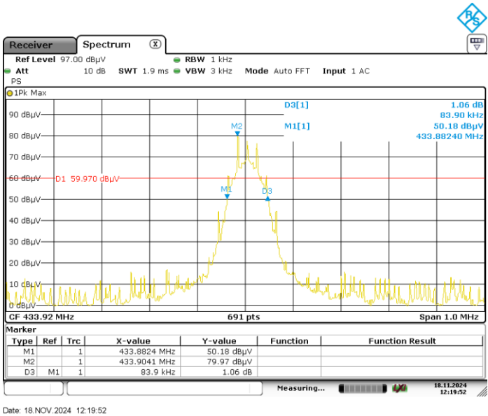
20dB Bandwidth
