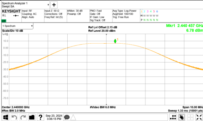
Channel 18 (2440MHz)
