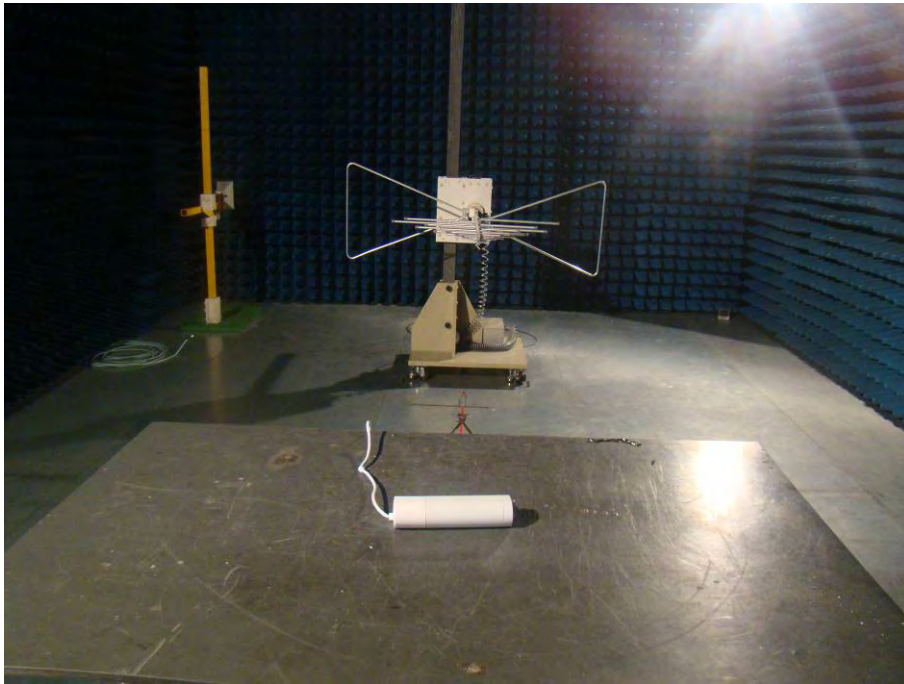
Radiated Spurious emission (up to 1G)
