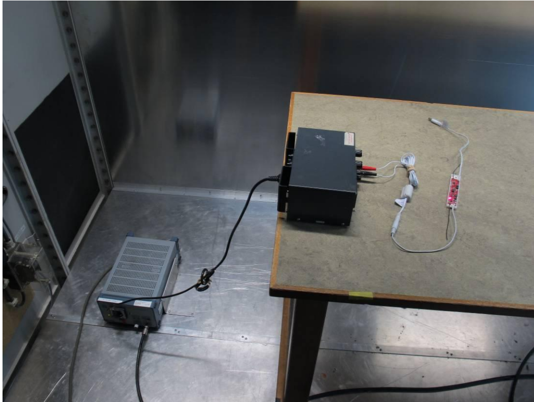
Photograph 4: - Test setup conducted emissions 0.15 – 30 MHz
