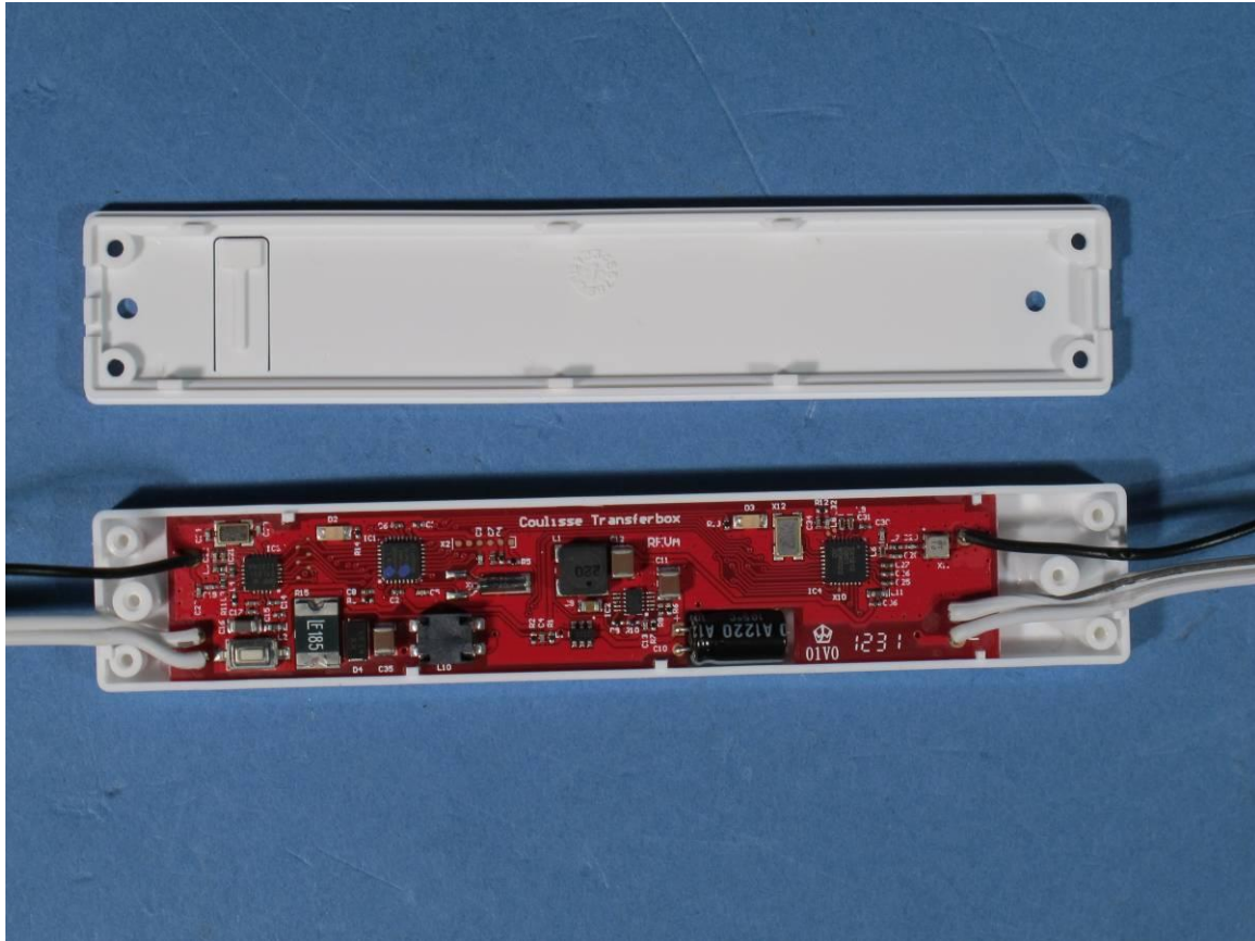
Photograph 1: - Internal view of ABC-22 PCB
