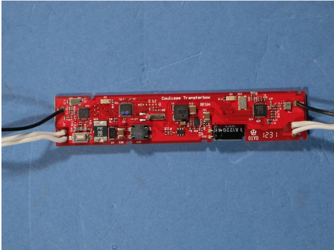
Photograph 2: - Top view of ABC-22 PCB
