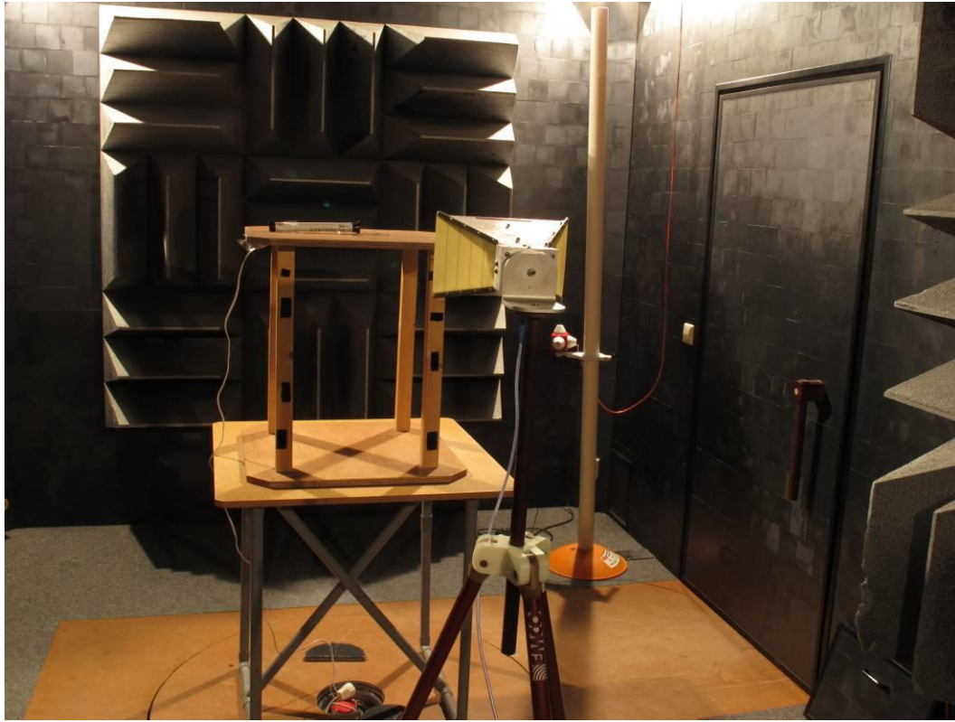
Photograph 3: Test setup radiated emissions 1-18 GHz)
