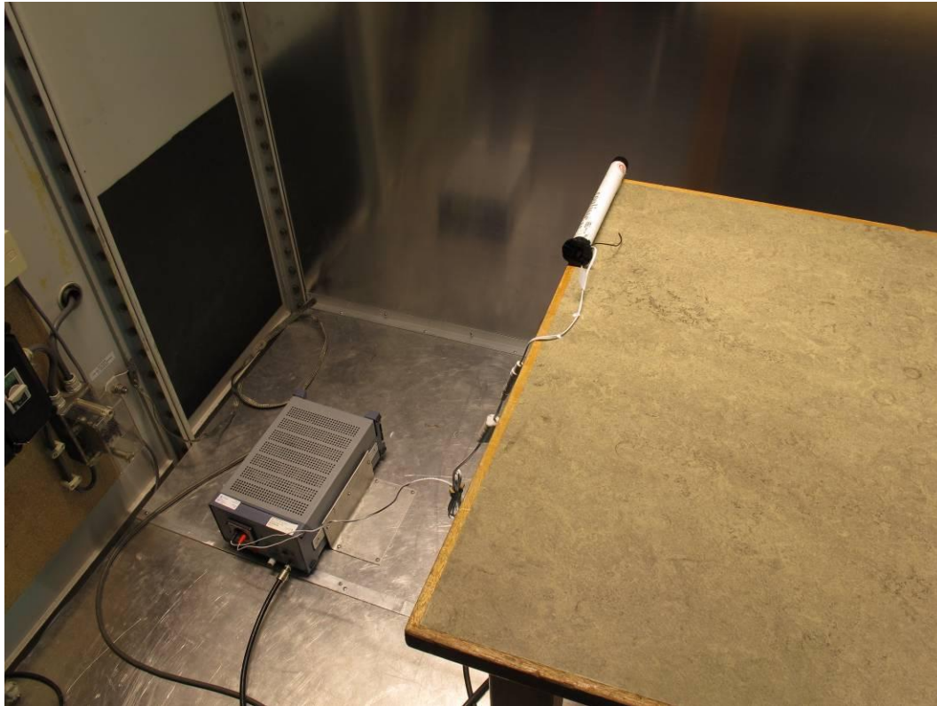
Photograph 5: Test setup conducted emissions on DC power port
