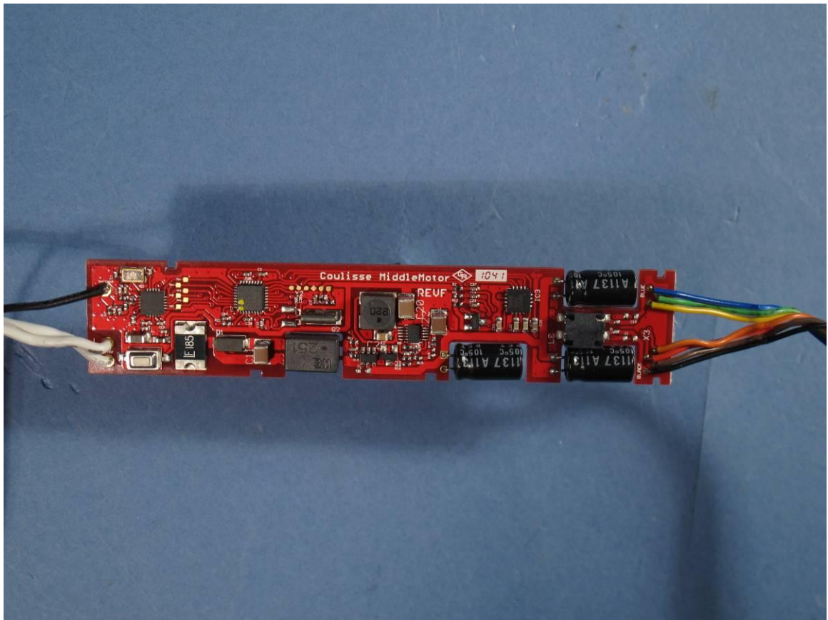
Photograph 3: - Main PCB of ABC-17, top view
