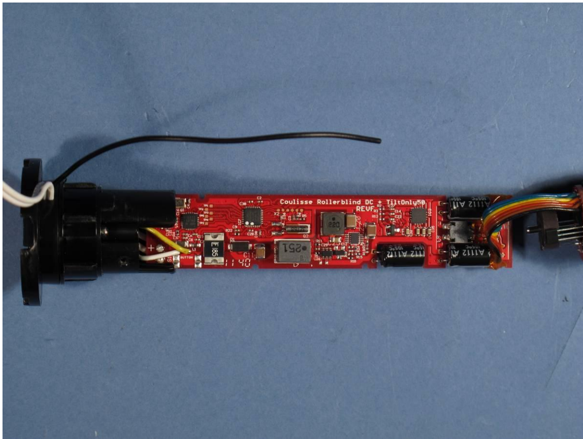
Photograph 1: - Main PCB of ABC-05, top view
