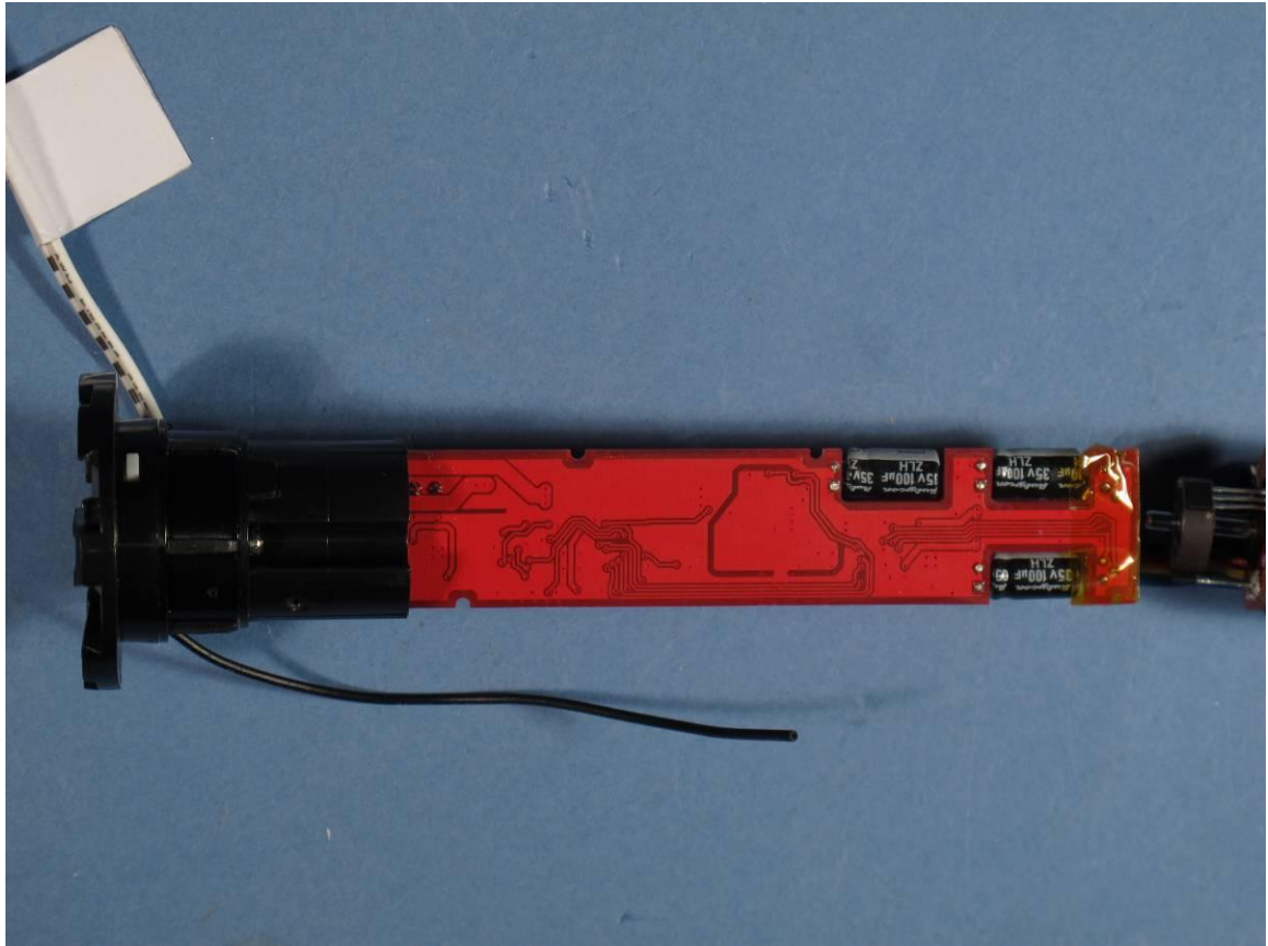
Photograph 2: - Main PCB of ABC-05, bottom view
