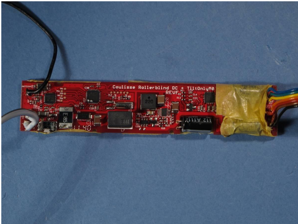
Photograph 6: - Main PCB of ABC-18, top view
