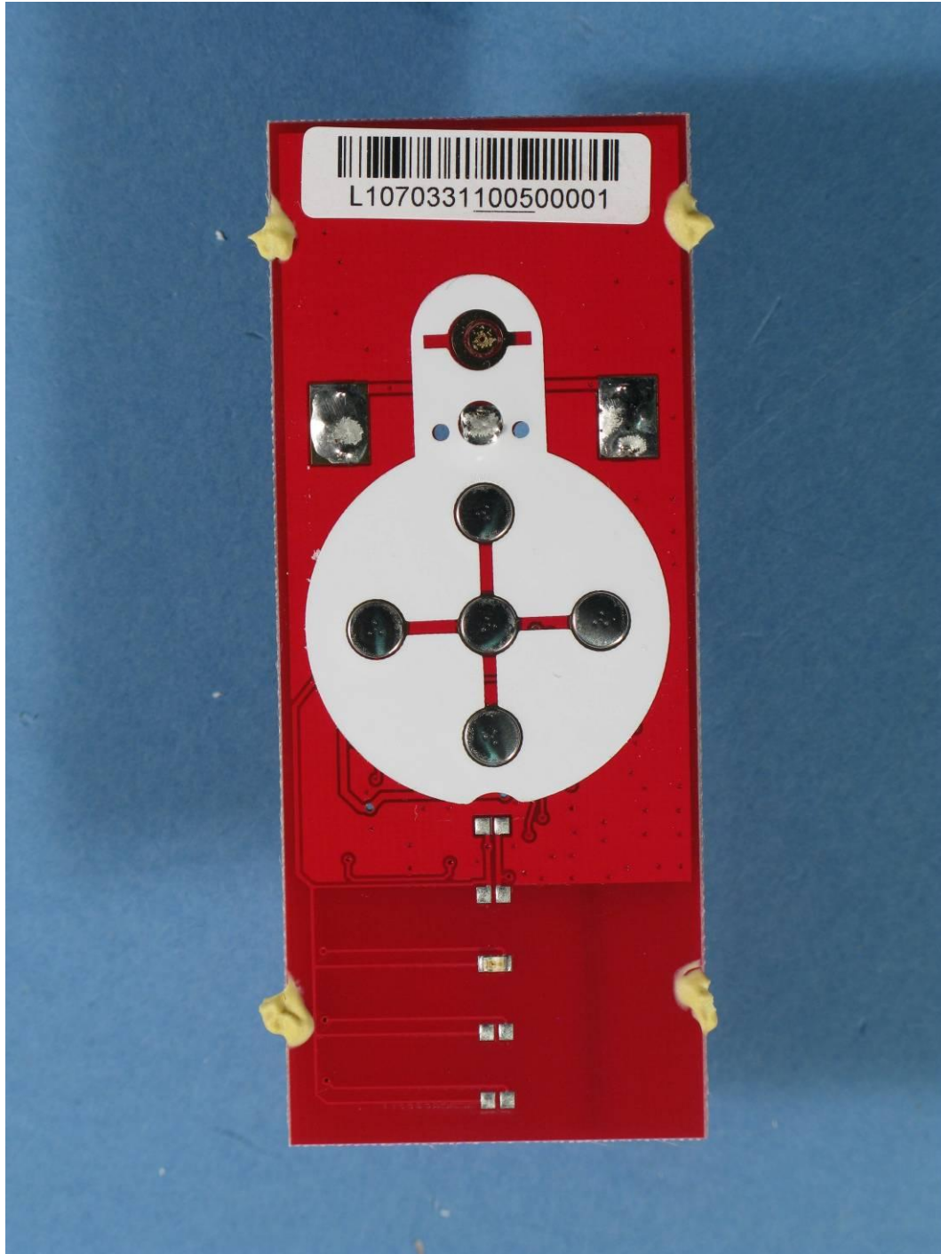
Photograph 3: - ABC-01 remote control, top view of PCB
