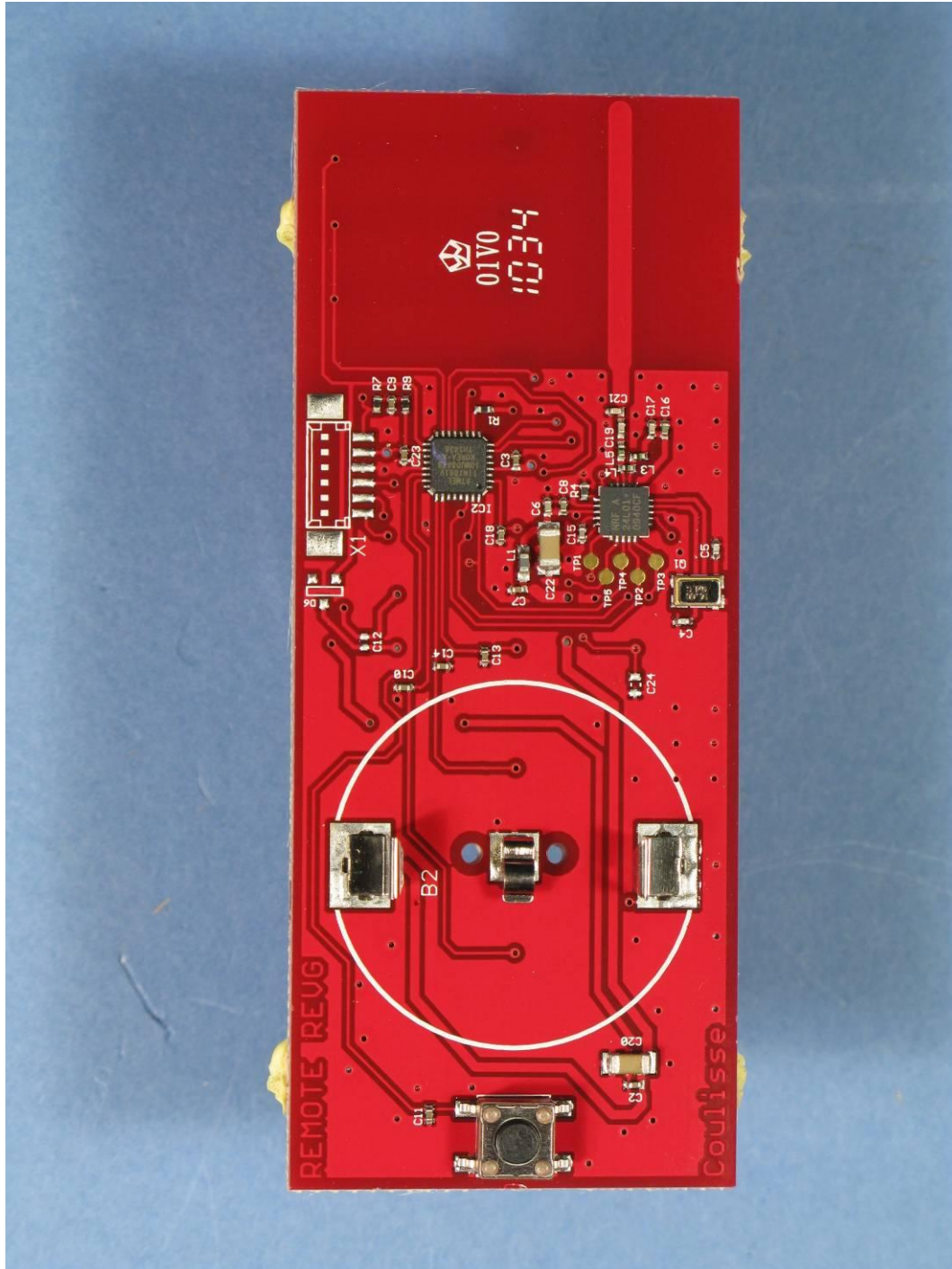
Photograph 4: - ABC-01 remote control, bottom view of PCB
