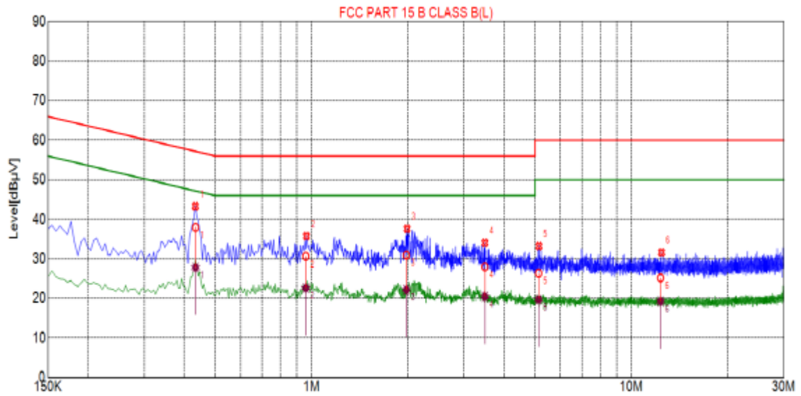
Line Conducted Emission Test Line 1-L
