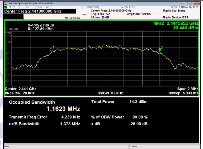
8DPSK_3-DH1_Channel 39
