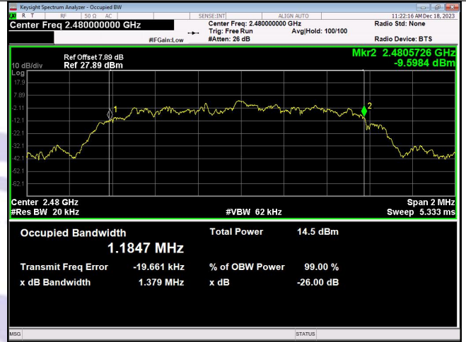
\pi/4 DQPSK_2-DH1_Channel 78
