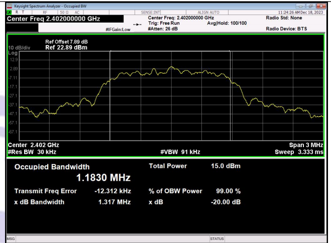
\pi/4 DQPSK_2-DH1_Channel 0
