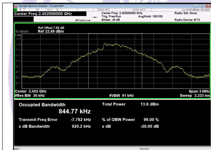
GFSK_DH1_Channel 0
