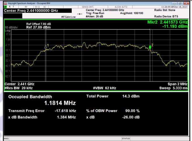
\pi/4 DQPSK_2-DH1_Channel 39
