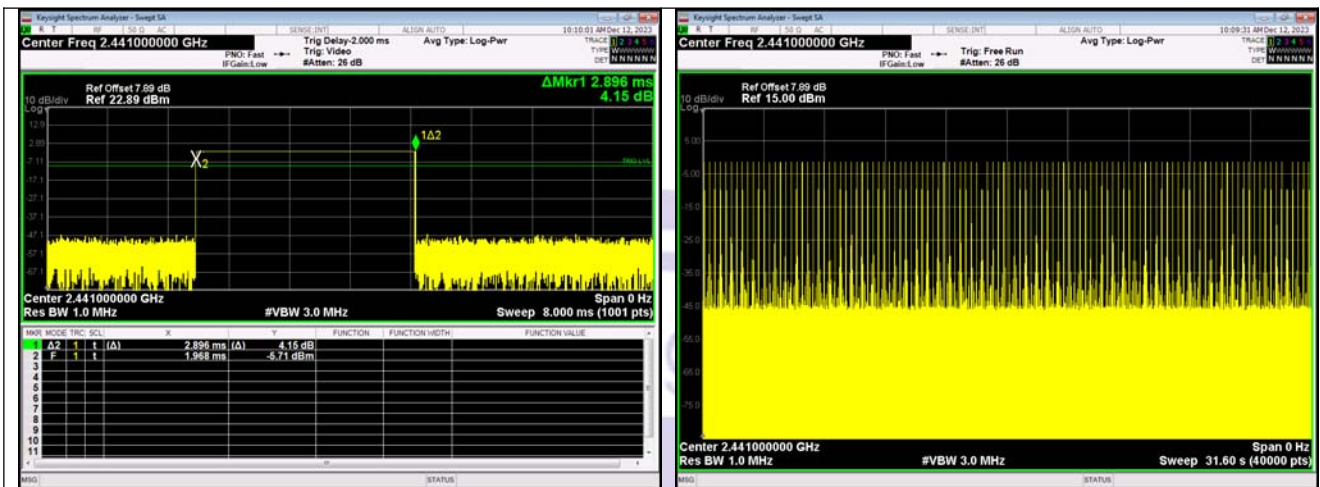
Pulse Width GFSK_DH5
